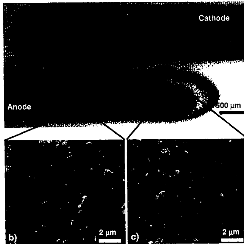
Figure 4.6: a) Optical micrograph of anode and cathode after testing (average electrode width: 858 \mu\text{m} ). The anode exhibited a white color in the region closest to the cathode and at the tip. b) Representative SEM micrograph of tested anode in region away from interelectrode gap and c) in white region close to the gap.
