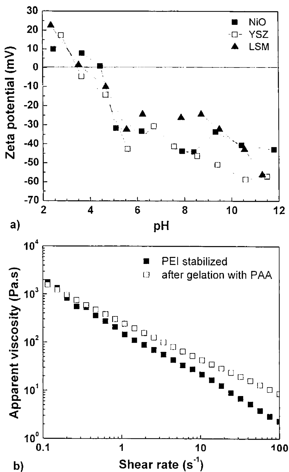
Figure A2.2: a) Zeta-potential as a function of pH for NiO, YSZ and LSM powders. b) Apparent viscosity as a function of shear rate for NiO-YSZ ink after stabilization of the powder with PEI in an aqueous suspension and after gelation.
