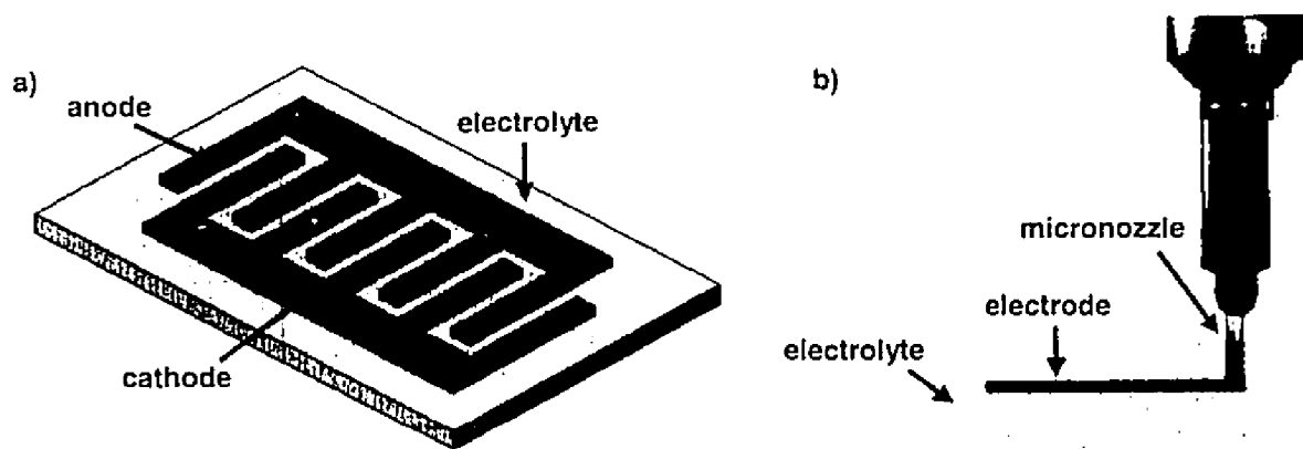
Figure A1.1: a) Schematic representation of single-chamber SOFC with interdigitated electrodes; b) Schematic representation of robot-controlled direct-write microfabrication.
