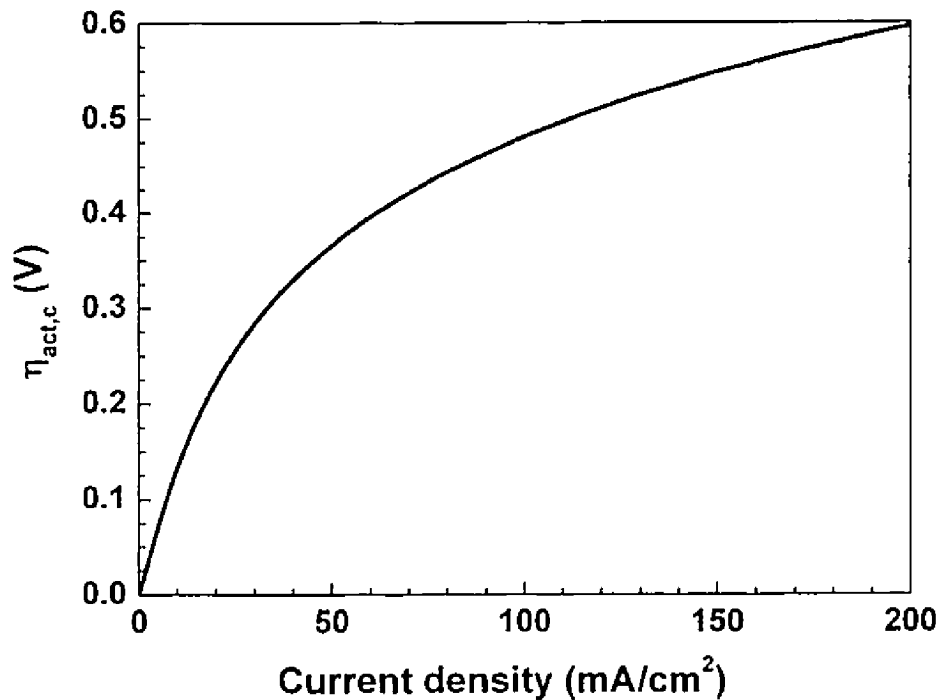
Figure 8.8: Cathode activation polarization as a function of current density.
