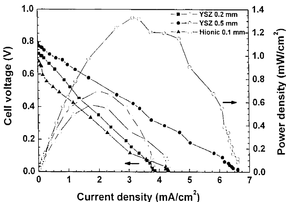
Figure 8.3: Cell voltage (closed symbols) and power density (open symbols) against current density for YSZ electrolytes of different thickness and a scandia stabilized zirconia electrolyte.
