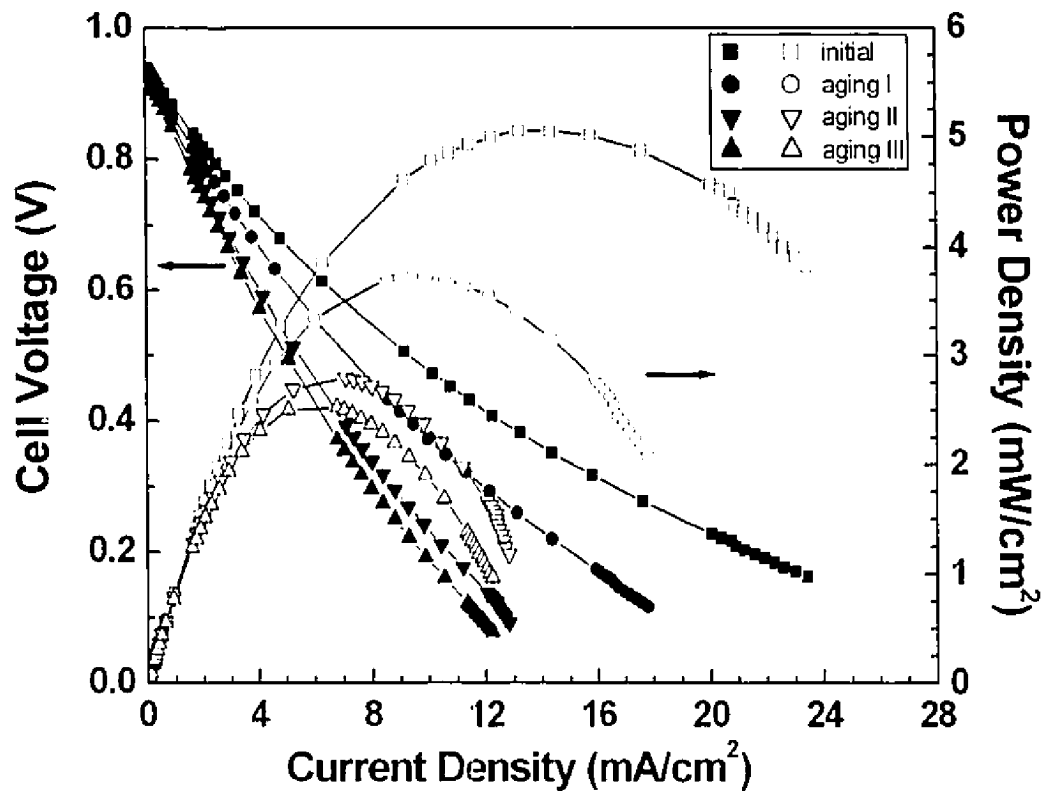
Figure 6.8: Voltage-current characteristics with performance decrease after aging I, II, and III, compared to initial performance, at 700°C and R_{\text{mix}} = 2 (cell Ni55cl).
