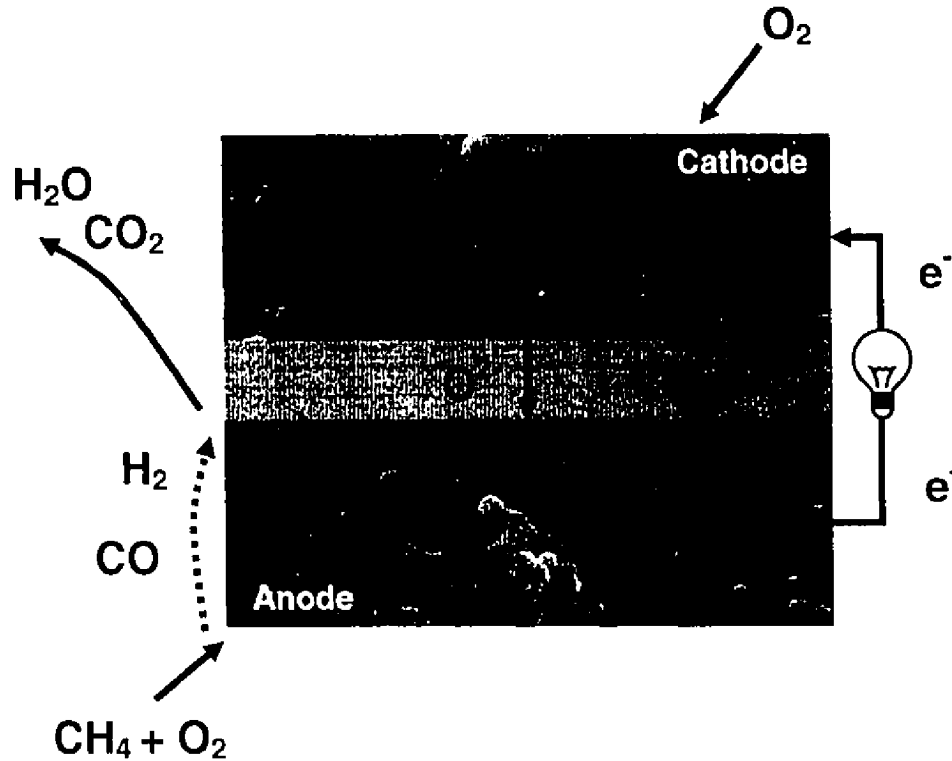
Figure 1.5: Schematic representation of the single-chamber working principle.
