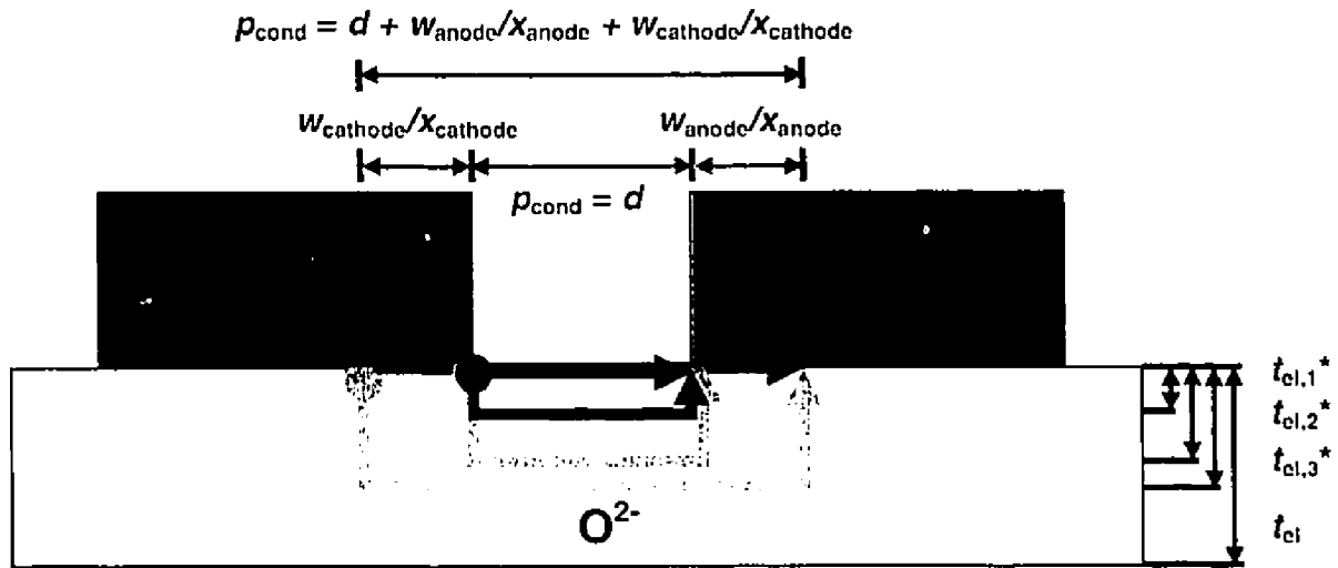
Figure 8.7: Schematics of possible ionic conduction paths.
