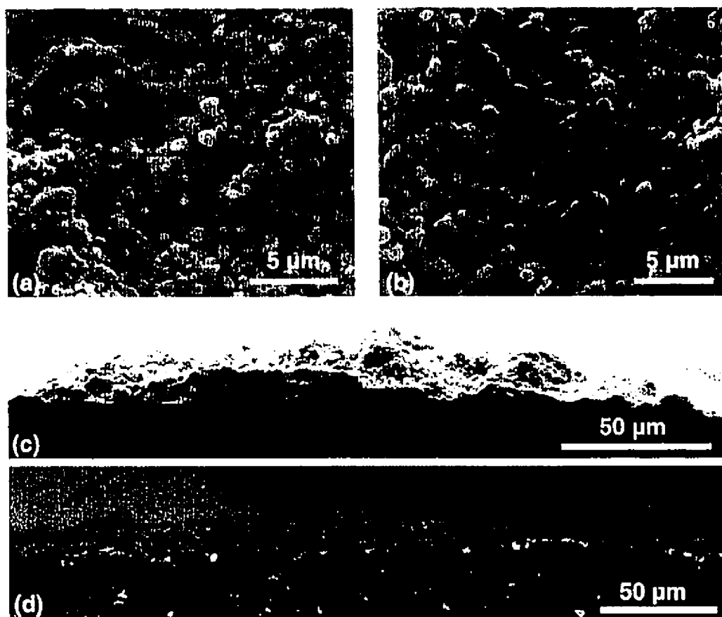
Figure 5.3: Scanning electron micrographs of the sintered electrodes showing plan views of a) anode and b) cathode, and cross-sectional views of c) anode and d) cathode.
