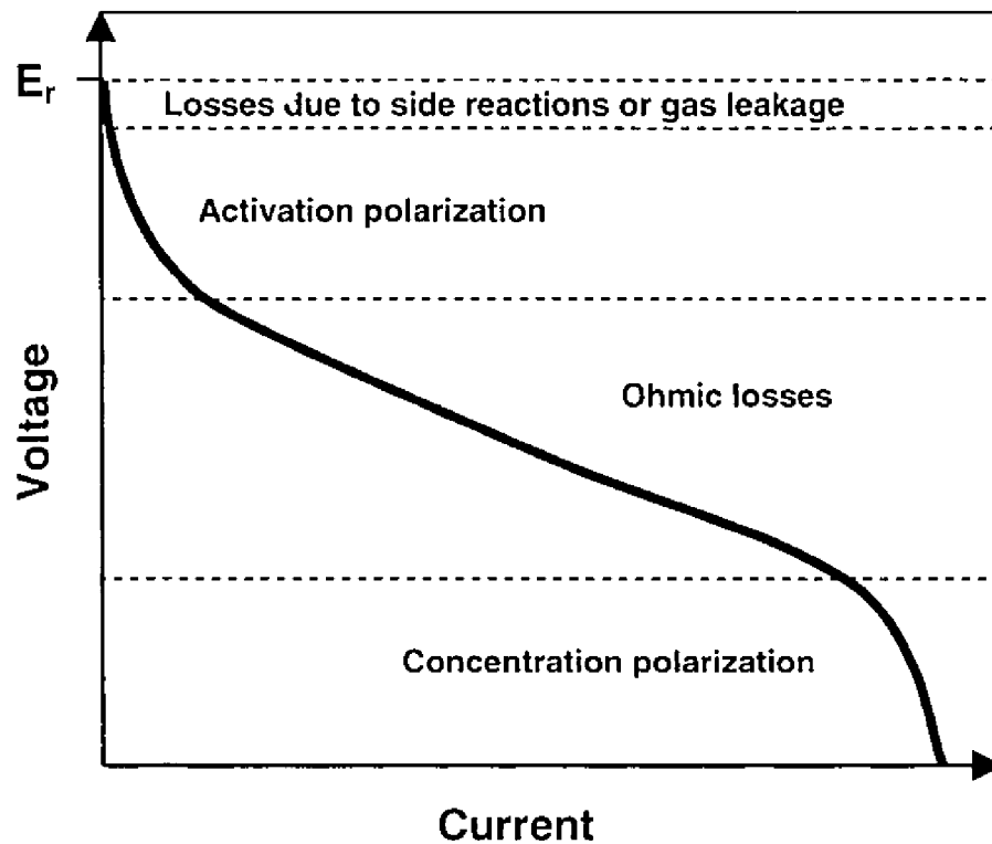
Figure 1.2: Typical polarization curve of a fuel cell.
