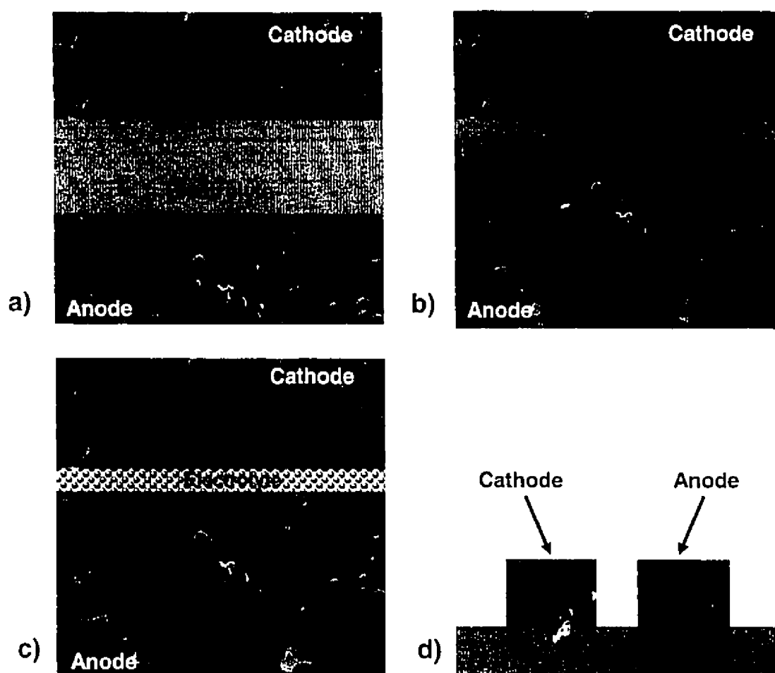
Figure 1.9: Schematics of the different SC-SOFC cell designs: a) electrolyte-supported cell, b) anode-supported cell, c) fully porous cell and d) single-face cell with coplanar electrodes.
