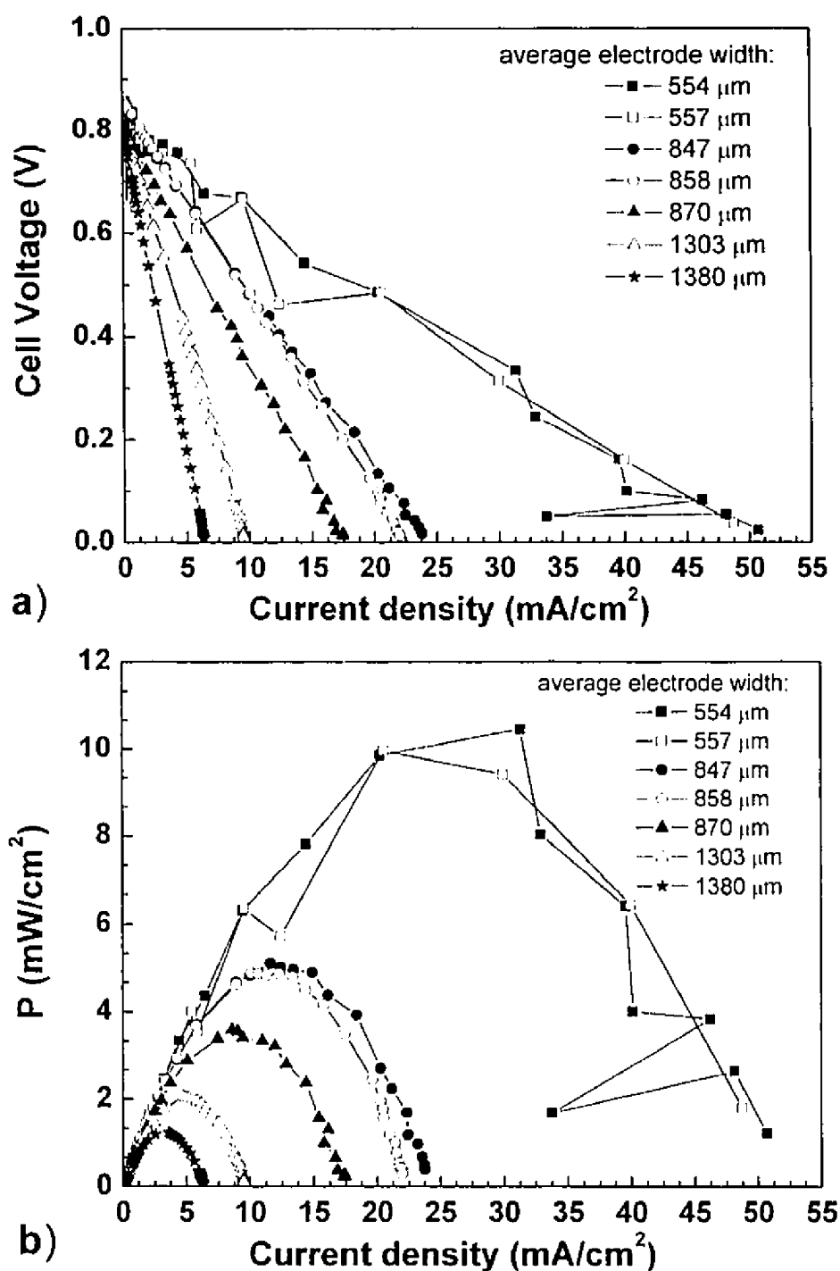
Figure 4.4: a) Cell voltage and b) power density against current density for cells with a single electrode pair delivering a non-zero OCV at 700^\circ\text{C} , R_{\text{mix}} = 2 and a total gas flow of 150 sccm.
