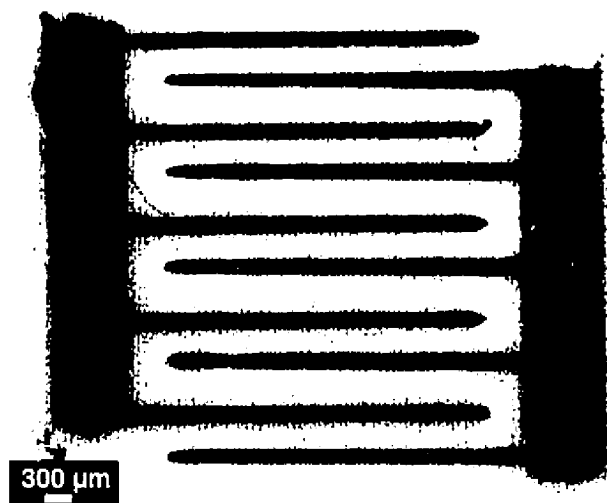
Figure A1.5: Optical micrograph of interdigitated LSM cathode (black) and NiO-YSZ anode (green) on YSZ electrolyte; average electrode width: 140 \mu\text{m} , average interelectrode spacing: 300 \mu\text{m} .
