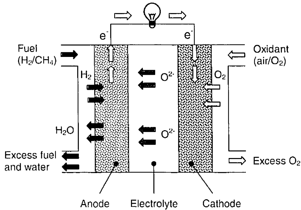
Figure 1.1: Schematic representation of the working principle of a solid oxide fuel cell.
