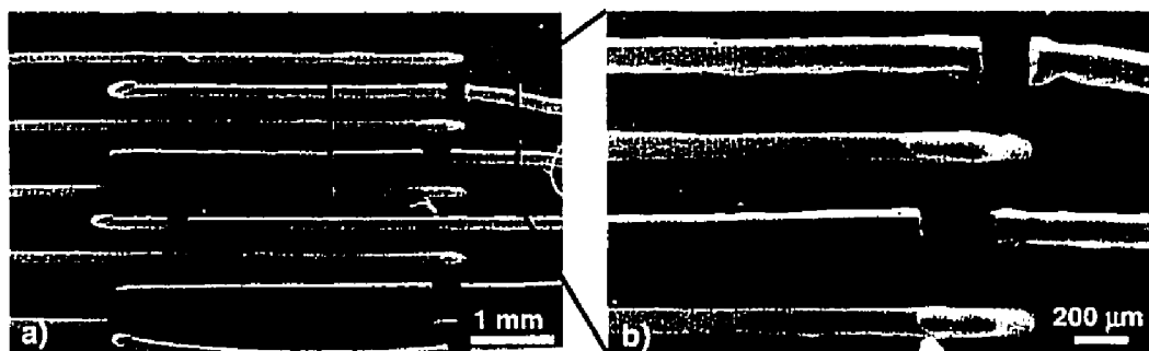
Figure A2.5: SEM images of a) anode and cathode lines in an interdigitated electrode structure, and b) close-up on broken anodes.
