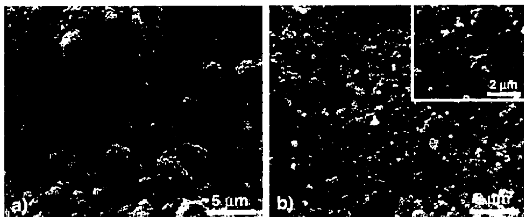
Figure 6.5: Anode microstructure of a) Ni55 cell and b) Ni80 cell after electrochemical testing under same conditions.
