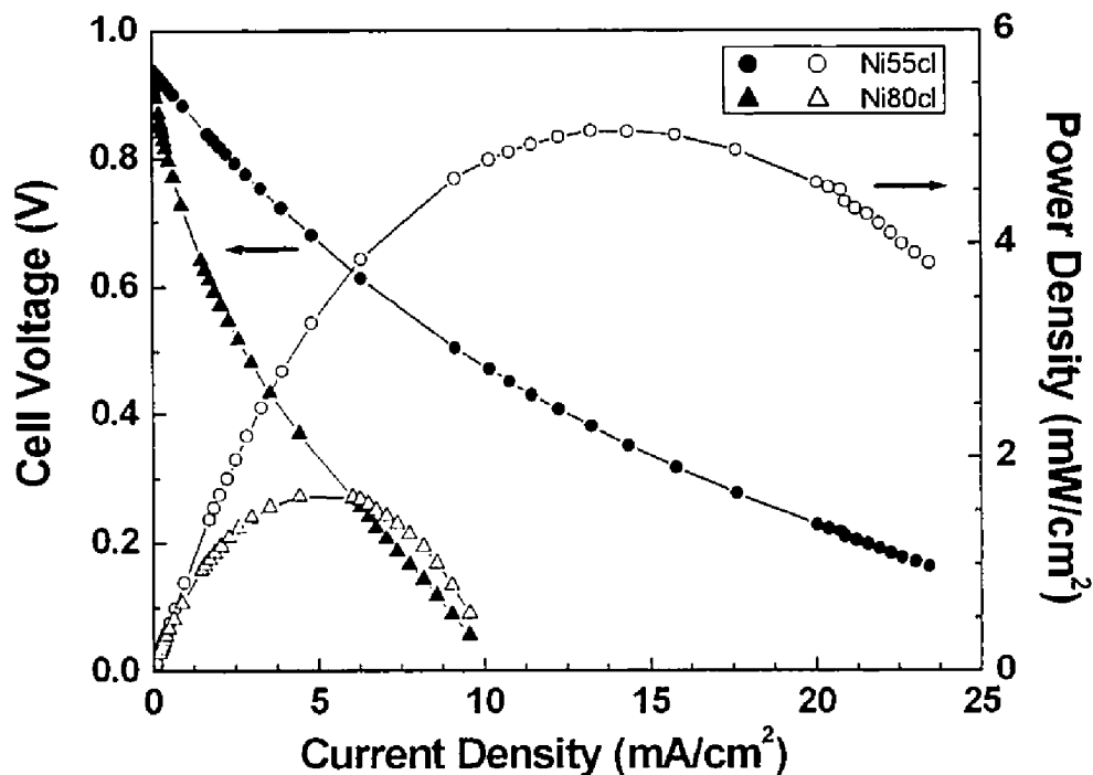
Figure 6.4: Cell voltage (closed symbols) and power density (open symbols) as a function of current density for cells Ni55cl and Ni80cl at 700°C and R_{\text{mix}} = 2 .
