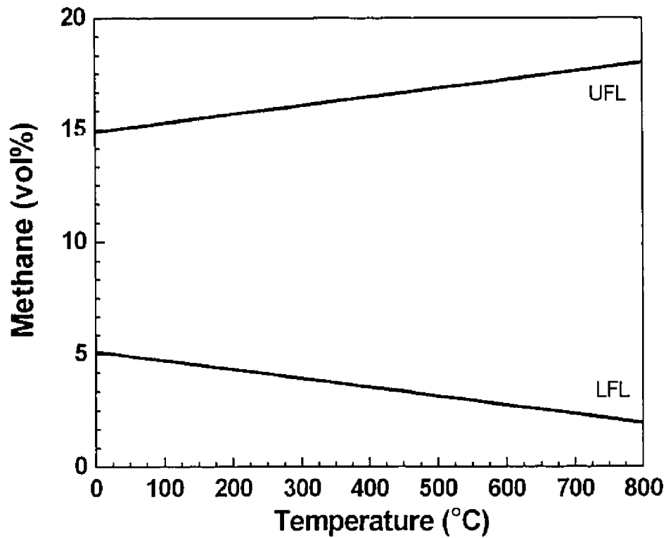
Figure 1.6: Lower and upper flammability limits of methane in air at 1 atm as a function of temperature.
