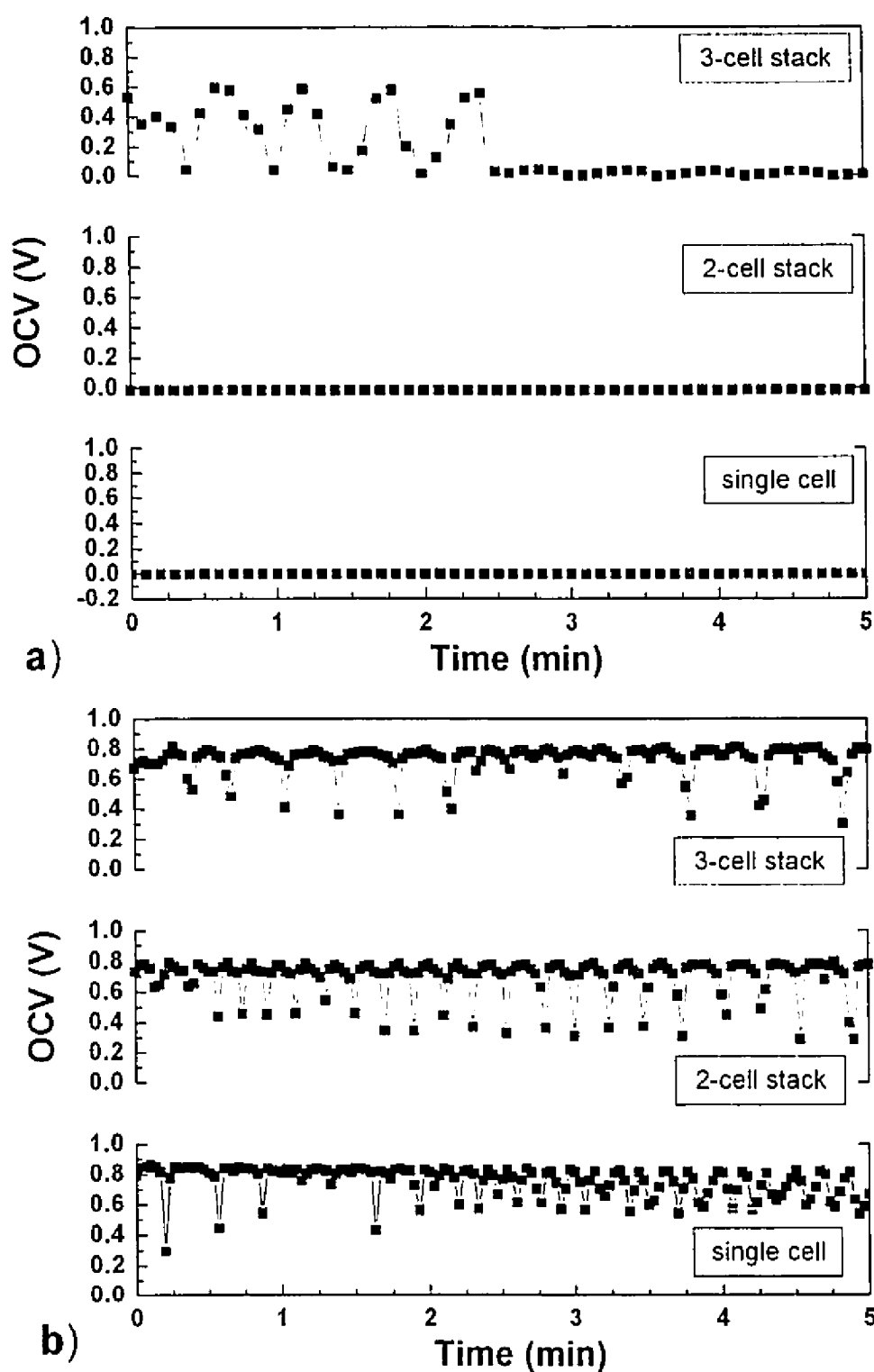
Figure 4.9: Representative time-dependent behavior of the OCV for cells with a) one and b) five electrode pairs as a single cell and assembled in a two-cell and three-cell stack. The OCV was measured at 700°C, R_{\text{mix}} = 2 and a total gas flow of 150 sccm.
