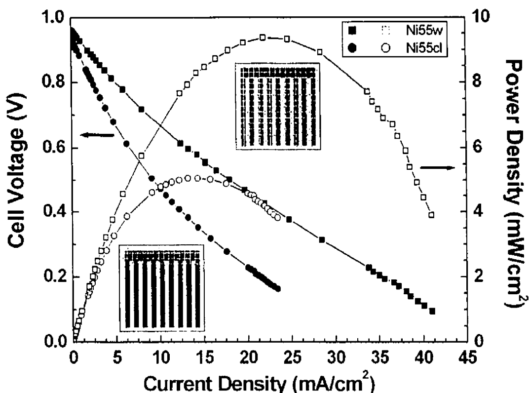
Figure 6.3: Cell voltage (closed symbols) and power density (open symbols) as a function of current density for current collection on the whole anode surface and on the connecting line at 700^\circ\text{C} and R_{\text{mix}} = 2 (cell Ni55).
