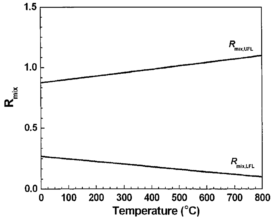
Figure 1.7: Critical methane-to-oxygen ratio R_{mix} as a function of temperature. The area between R_{mix,LFL} and R_{mix,UFL} represents the zone of flammability.
