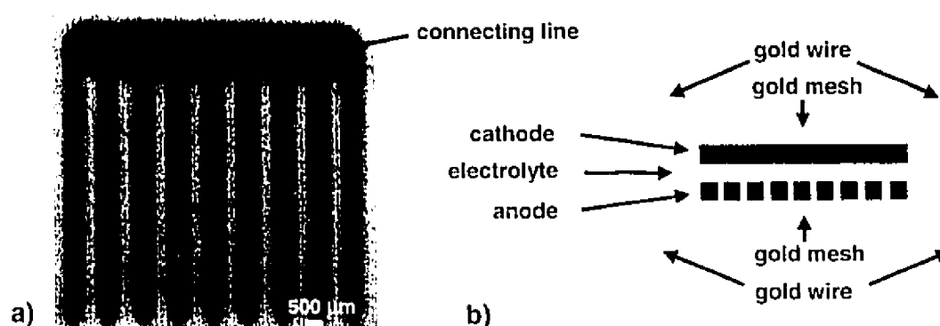
Figure 6.1: a) Micrograph of comblike anode after sintering. b) Schematics of SC- \mu SOFC in dual-face configuration.
