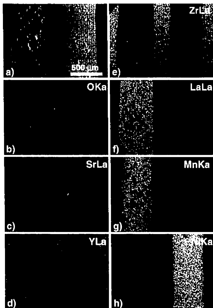
Figure 7.6: a) SEM micrograph of EDX analyzed section showing cathode (left electrode line), electrolyte and anode (right electrode line) of the NiO-YSZ/YSZ/LSM-YSZ cell. b)-h) Chemical map analysis of O, Sr, Y, Zr, La, Mn, Ni in cathode, anode and electrolyte.
