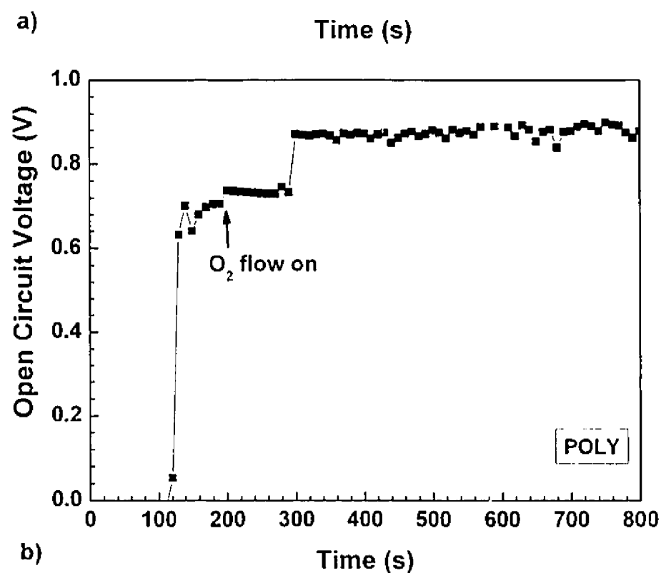
Figure 5.4: Open circuit voltage as a function of time for a) "SOFC" and b) "POLY" electrode geometry during fuel cell operation in a methane-air mixture (methane-to-oxygen ratio R_{\text{mix}} = 2 ) at 700°C and a gas flow rate of 150 sccm. The methane/nitrogen mixture was allowed to flow over the cell at t = 0 s.
