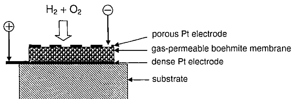
Figure 1.8: Schematics of Dyer's room-temperature single-chamber fuel cell.
