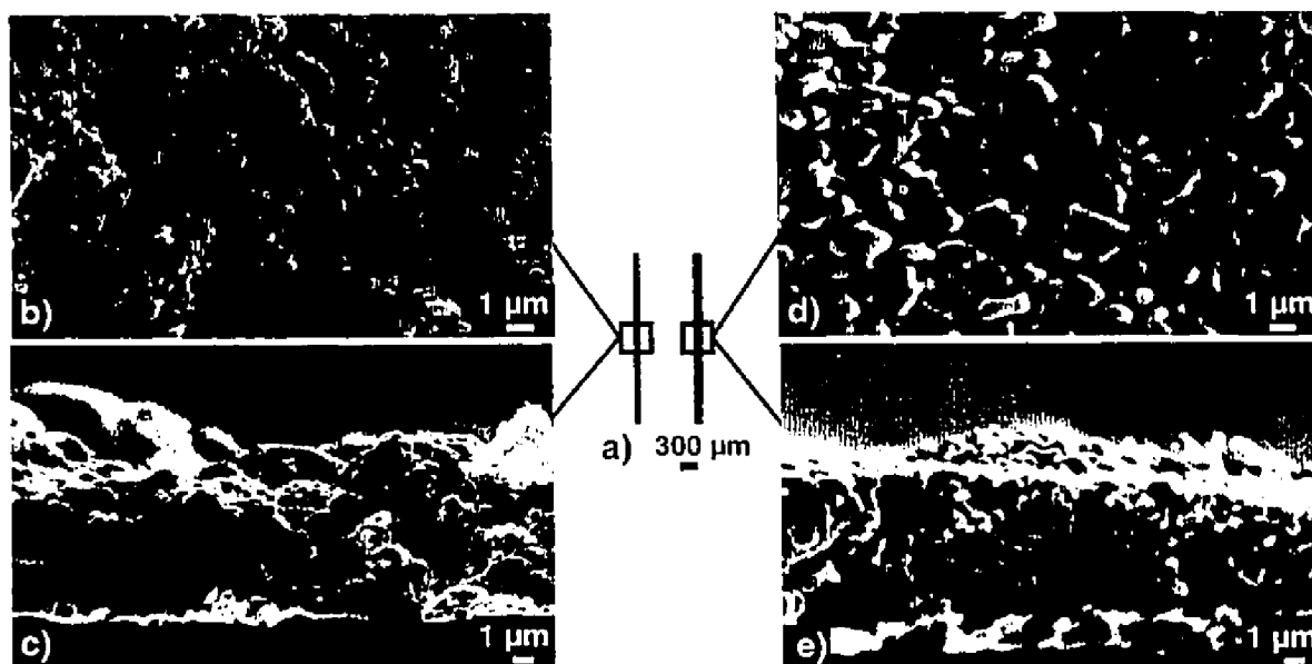
Figure A1.4: a) Optical micrograph of NiO-YSZ anode (left) and LSM cathode (right) lines on YSZ electrolyte; b) - e) SEM images of sintered direct-written electrode microstructures: b) anode, top surface; c) anode, cross-section; d) cathode, top surface; e) cathode, cross-section.
