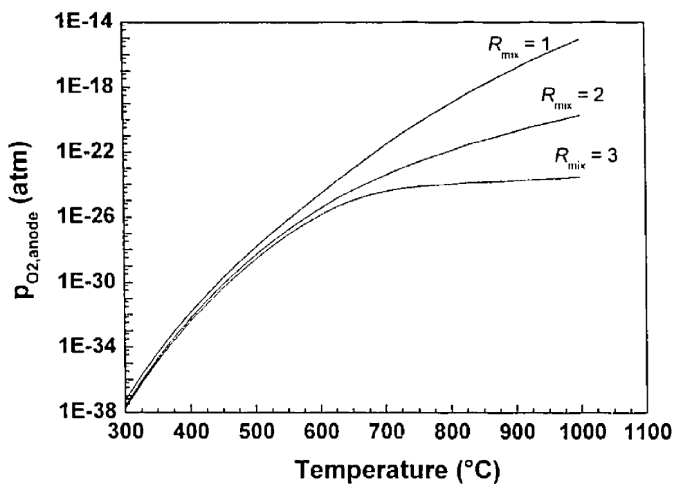
Figure 8.4: Oxygen partial pressure at the anode as a function of temperature for different methane-air gas mixture compositions.
