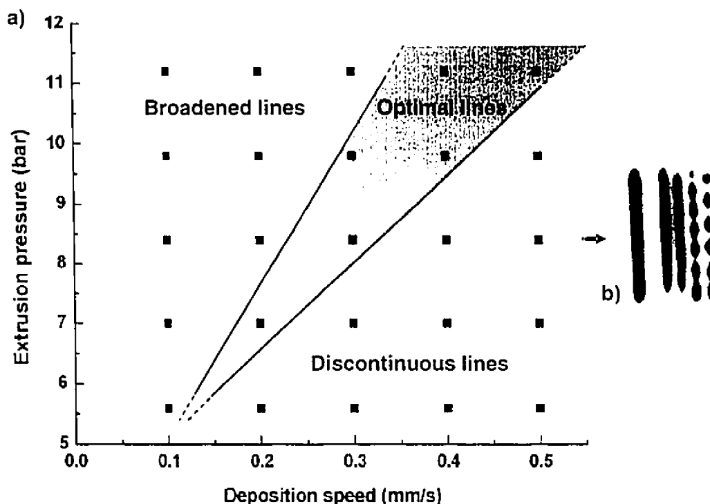
Figure 3.4: a) Representative process map for direct-write microfabrication of anode lines with axes corresponding to extrusion pressure and deposition speed. The 60 wt% anode suspension was extruded through a micronozzle with an inner nozzle diameter of 150 \mu\text{m} . Optimal deposits with uniform, continuous lines were obtained for pressure-speed combinations within the grey area. b) Optical micrograph corresponding to an extrusion pressure of 8.4 bar. From left to right, the single lines correspond to the deposition speed of 0.1, 0.2, 0.3, 0.4 and 0.5 mm/s, respectively.
