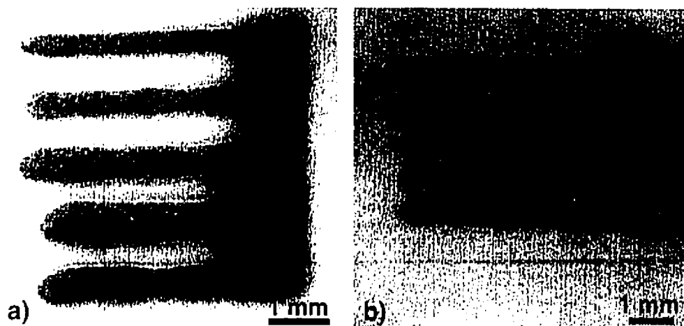
Figure A2.1: Optical micrograph of a) anode fabricated from Newtonian ink, featuring spreading and uniformity limitations, and b) homogenous cathode fabricated from viscoelastic ink using the direct-write microfabrication technique.
