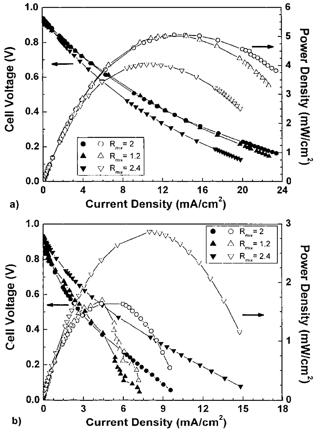
Figure 6.7: Cell voltage (closed symbols) and power density (open symbols) as a function of current density for different R_{mix} at 700°C. The cells, a) cell Ni55cl and b) Ni80cl, were first exposed to R_{mix} = 2 , followed by R_{mix} = 1.2 and then R_{mix} = 2.4 .
