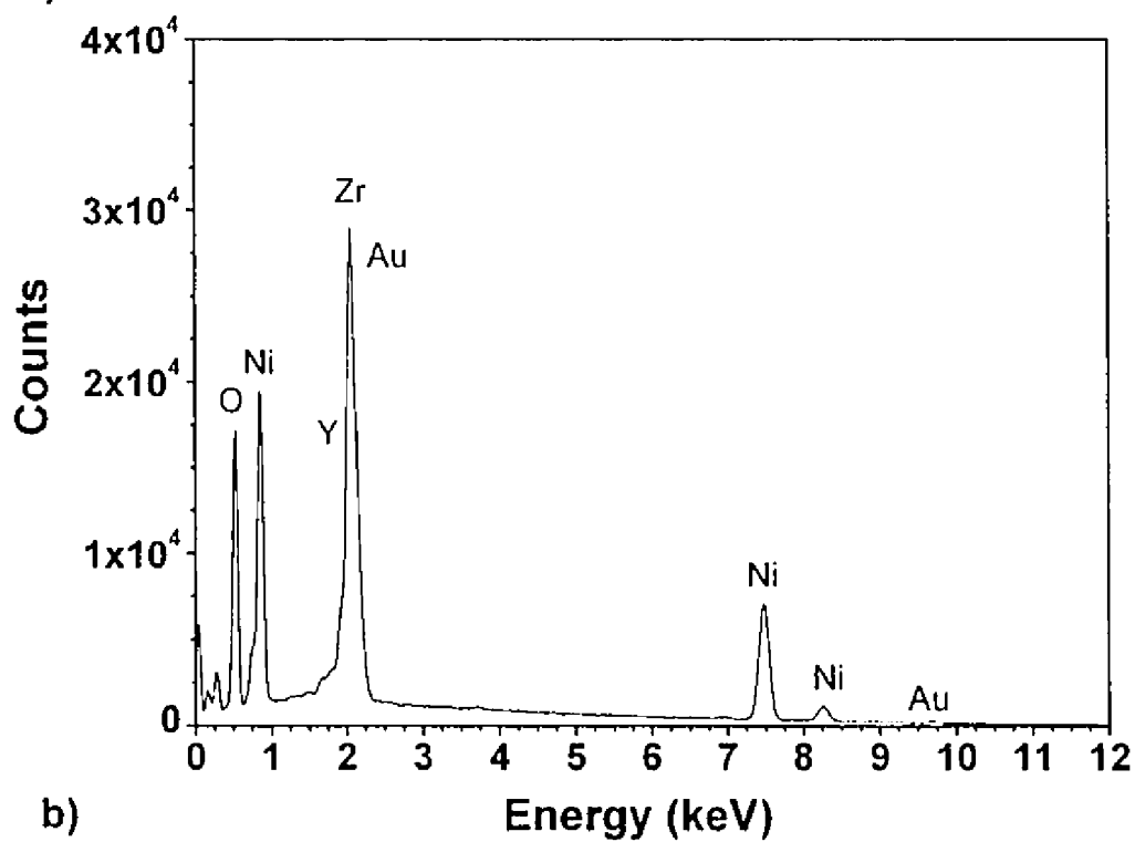
Figure 7.4: EDX spectra of NiO-YSZ anodes in close vicinity of a) LSM-YSZ and b) LSCF cathodes after sintering.
