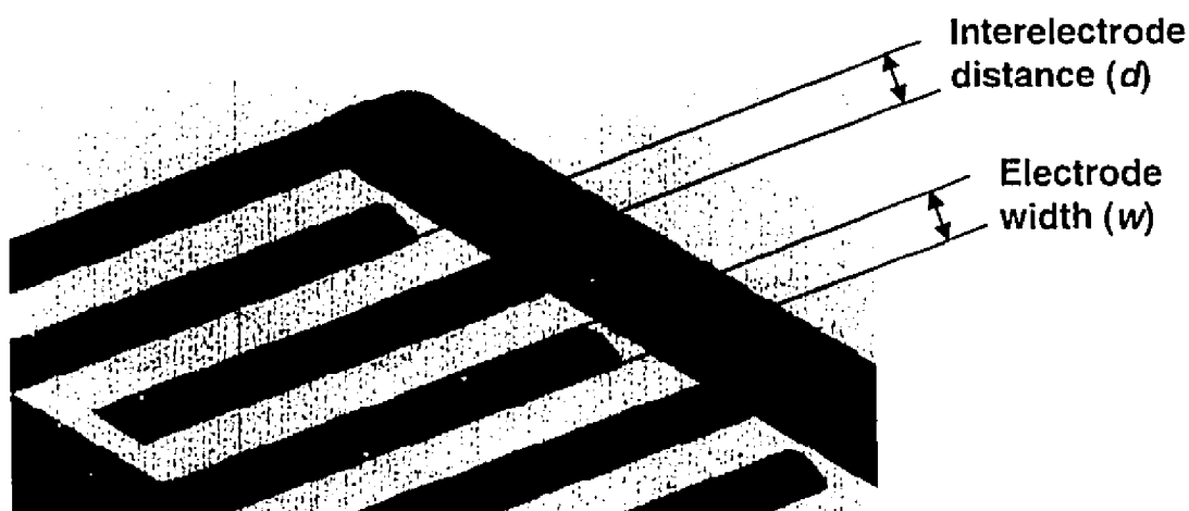
Figure I2: Schematic illustration of interelectrode distance and electrode width.
