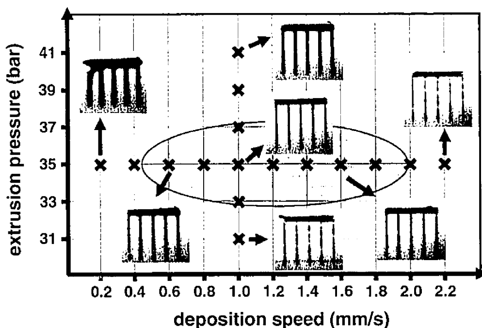
Figure A1.3: Effects of extrusion pressure and deposition speed on size and uniformity of direct-write deposition of 60 wt% anode suspension using a 100 \mu\text{m} diameter nozzle.
