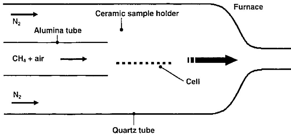
Figure 3.6: Schematic of the electrochemical testing setup. The cell is placed in a ceramic holder inside a quartz tube. The methane-air mixture is supplied to the cell through an inner alumina tube. Additional nitrogen is used as carrier gas and to avoid counter-diffusion.
