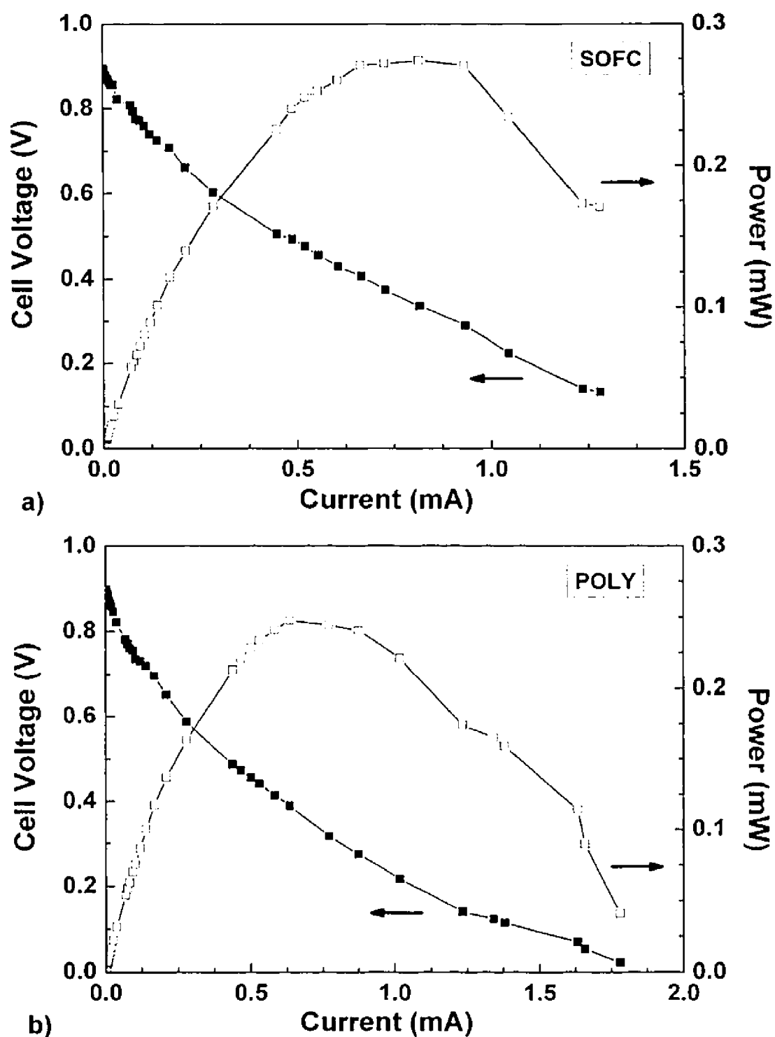
Figure 5.5: Voltage-current characteristics of the a) "SOFC" and b) "POLY" geometry. Both tests were performed in a methane-air mixture with R_{\text{mix}} = 2 and a total gas flow of 150 sccm at 700°C.
