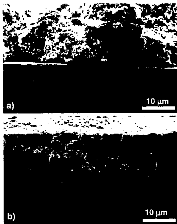
Figure 7.3: SEM micrograph of a) NiO-GDC and b) NiO-YSZ anode cross-section on top of the YSZ electrolyte after sintering.
