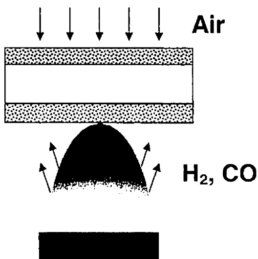
Figure 1.3: No-chamber or direct-flame SOFC.
