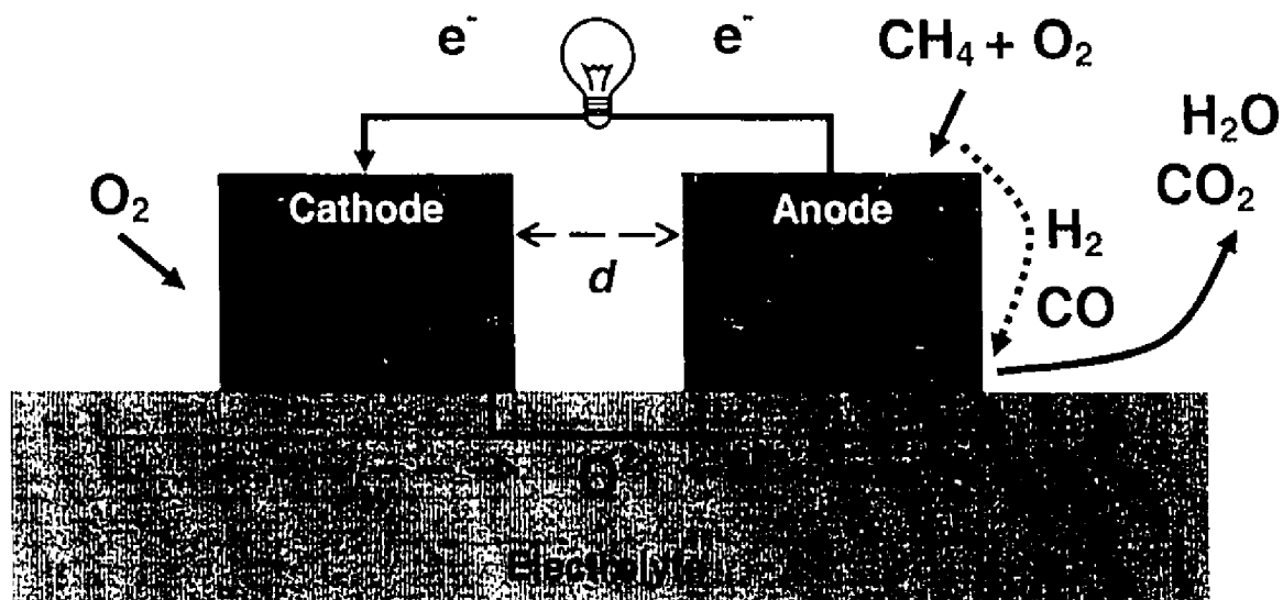
Figure 1.10: Schematics of the operating principle of SC-SOFCs with coplanar electrodes; d is the interelectrode spacing and w denotes the electrode width.
