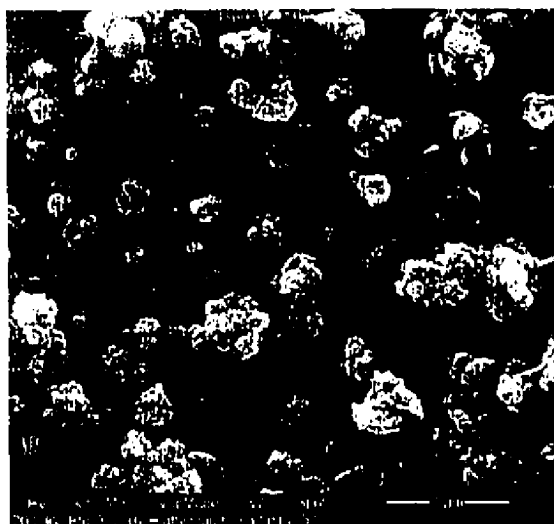
Figure 3.9: Scanning electron micrograph of the anode after electrochemical testing. The bright flake-like regions consist of metallic nickel.
