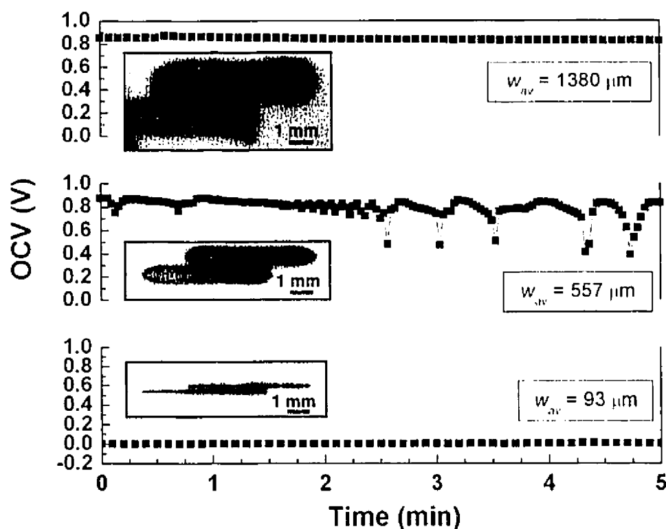
Figure 4.5: Representative time-dependent behavior of the OCV for cells with one electrode pair of different average electrode widths (93, 557 and 1380 \mu\text{m} ) at 700°C, R_{\text{mix}} = 2 and a total gas flow of 150 sccm.
