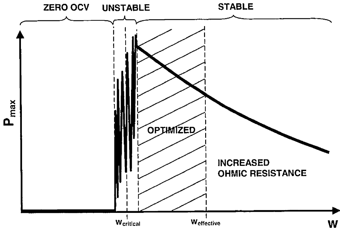
Figure 4.7: Schematic representation of design criteria for SC- \mu SOFCs with one coplanar electrode pair.
