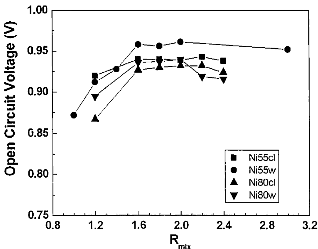
Figure 6.6: OCV as a function of R_{mix} for the four tested cells at 700°C.
