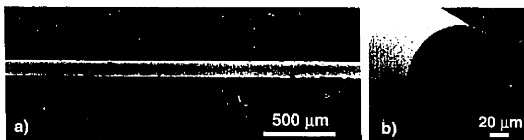
Figure 8.2: SEM image of a sintered NiO-YSZ electrode line fabricated from viscoelastic, gel-like inks using the direct-writing technique: a) top view, b) cross-sectional view.
