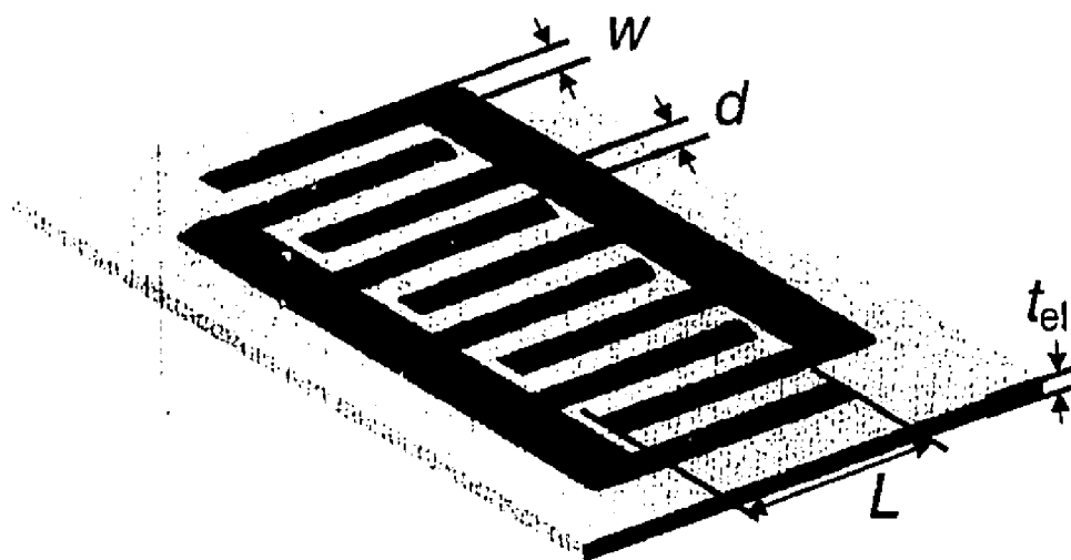
Figure 8.6: Definition of the geometrical cell parameters: w = electrode width, d = interelectrode gap, t_{el} = electrolyte thickness, L = overlapping electrode length.
