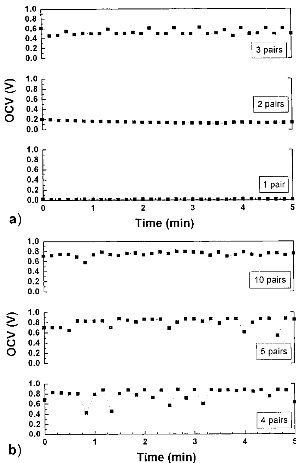
Figure 4.8: Representative time-dependent behavior of the OCV for cells with a) one, two, three and b) four, five and ten pairs of interdigitated electrodes. The OCV was measured at 700°C, R_{\text{mix}} = 2 and a total gas flow of 150 sccm.
