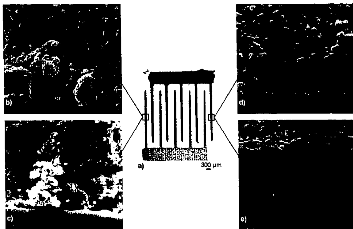
Figure 3.5: a) Optical micrograph of SC- \mu SOFC with interdigitated electrodes fabricated by the direct-write technique. SEM images of the anode microstructure in b) top and c) cross-sectional view. SEM microstructure characterization of the cathode in d) top and e) cross-sectional view.
