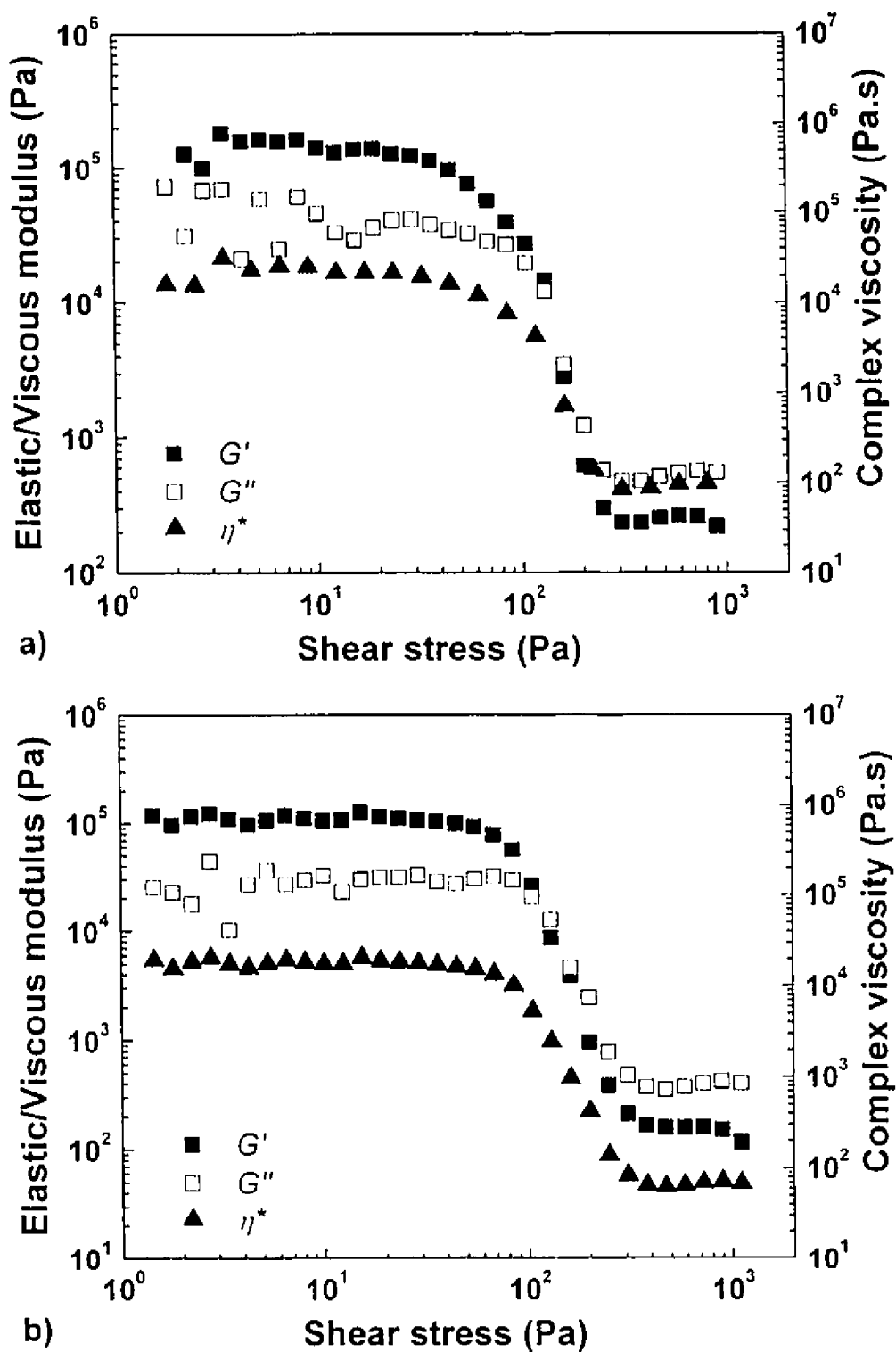
Figure A2.3: Shear stress amplitude sweeps of a) NiO-YSZ and b) LSM-YSZ electrode inks at 1 Hz and 25°C.
