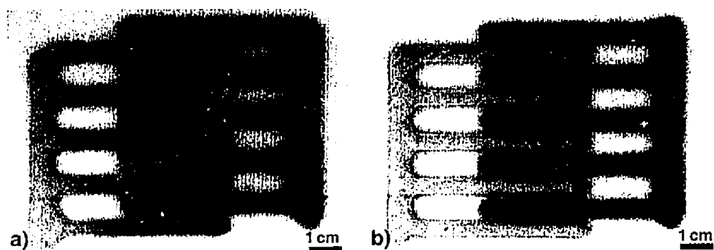
Figure 7.1: Optical micrograph of cell a) NiO-YSZ/YSZ/LSM-YSZ and b) NiO-YSZ/YSZ/LSCF after sintering.
