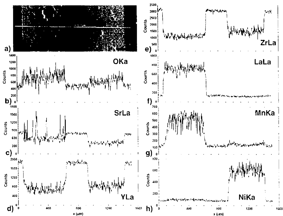
Figure 7.5: a) SEM micrograph of the section analyzed by EDX showing cathode (left electrode line), electrolyte and anode (right electrode line) of the NiO-YSZ//YSZ//LSM-YSZ cell; b)-h) Line scan chemical analysis performed over the three cell components.
