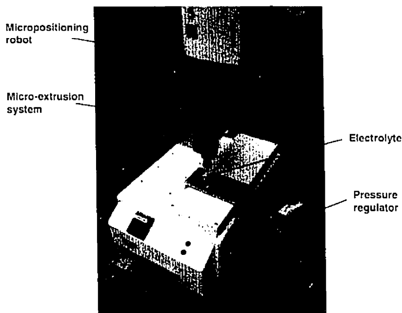
Figure 3.3: Picture of the direct-write microfabrication setup. The sample is mounted on a translation stage, and the micro-extrusion system on a robotic arm permits writing of arbitrary shapes.
