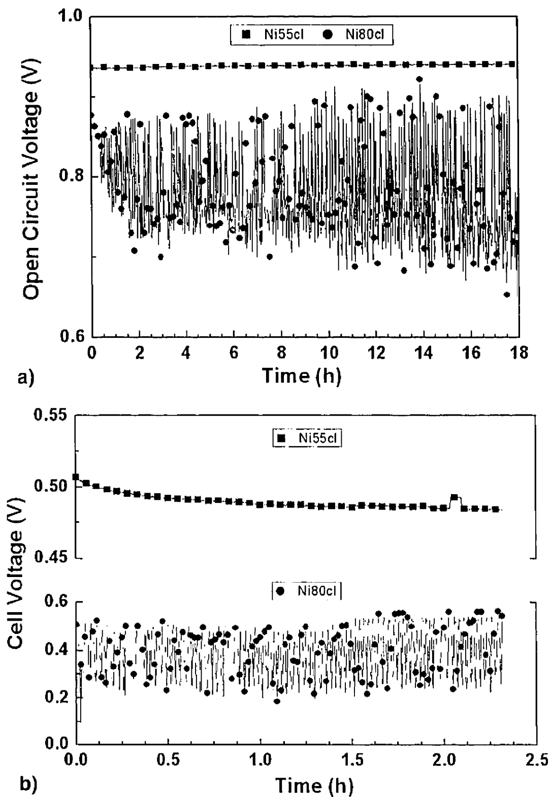
Figure 6.9: Voltage as a function of time for cells Ni55cl and Ni80cl during a) aging at I = 0 mA and b) at I = 50\% of I_{\max} ( 700^{\circ}\text{C} , R_{\max} = 2 ).
