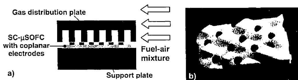
Figure 4.2: a) Schematic representation of the cell holder, where the SC- \mu SOFC with coplanar electrodes is placed between a support plate and a gas distribution plate. b) Photograph of the lower side of the gas distribution plate facing the cell. Holes are machined into the plate to let the reaction gases access the cell underneath, whereas the posts are to enhance mixing of the reactant gases flowing over the electrodes.
