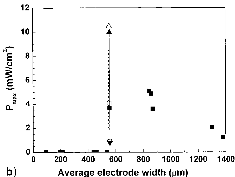
Figure 4.3: a) Open circuit voltage and b) maximum power density as a function of average electrode width for cells with a single electrode pair. The tests were performed at 700^\circ\text{C} , R_{\text{mix}} = 2 and a total gas flow rate of 150 sccm. \blacktriangle\triangle and \blacktriangledown\triangledown correspond to the maximum and minimum value of the OCV and maximum power density obtained for the unstable cells with fluctuating voltage.
