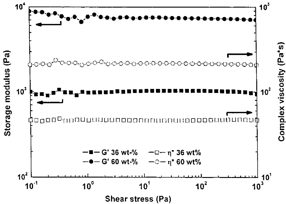
Figure 3.2: Rheological properties (storage modulus, G' , and complex viscosity, \eta^* ) of anode suspensions with two different particle loadings as a function of shear stress at a frequency of 10 Hz.
