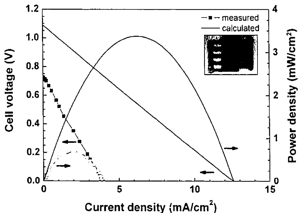
Figure 8.10: Measured and calculated cell voltage and power density as functions of current density for cell C5L_Ch7 with five lines per anode and cathode.
