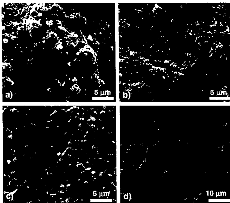
Figure 6.2: Anode microstructure of a) Ni55 cell and b) Ni80 cell after sintering. Cathode microstructure: c) top view, d) cross-sectional view.
