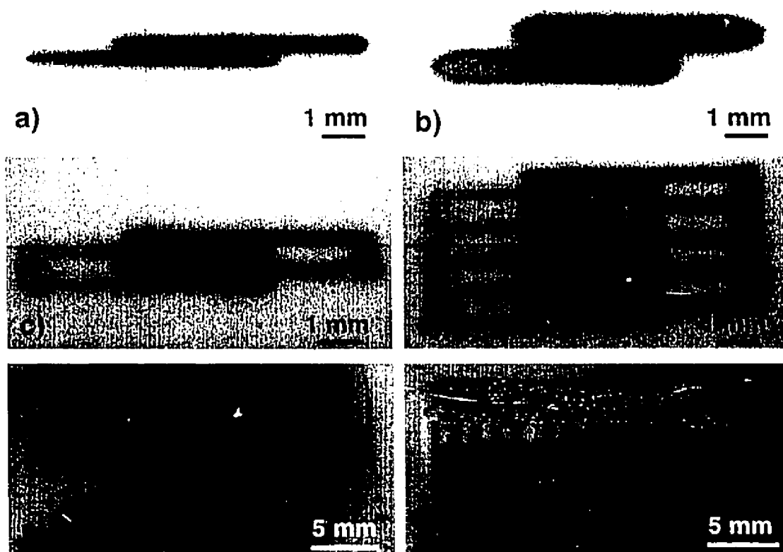
Figure 4.1: Optical micrographs of SC- \mu SOFCs with single electrode pair (average electrode width of a) 201 \mu m and b) 537 \mu m) and with c) two and d) five pairs of electrodes. Stack of three cells with e) one line per electrode and f) five lines per electrode.
