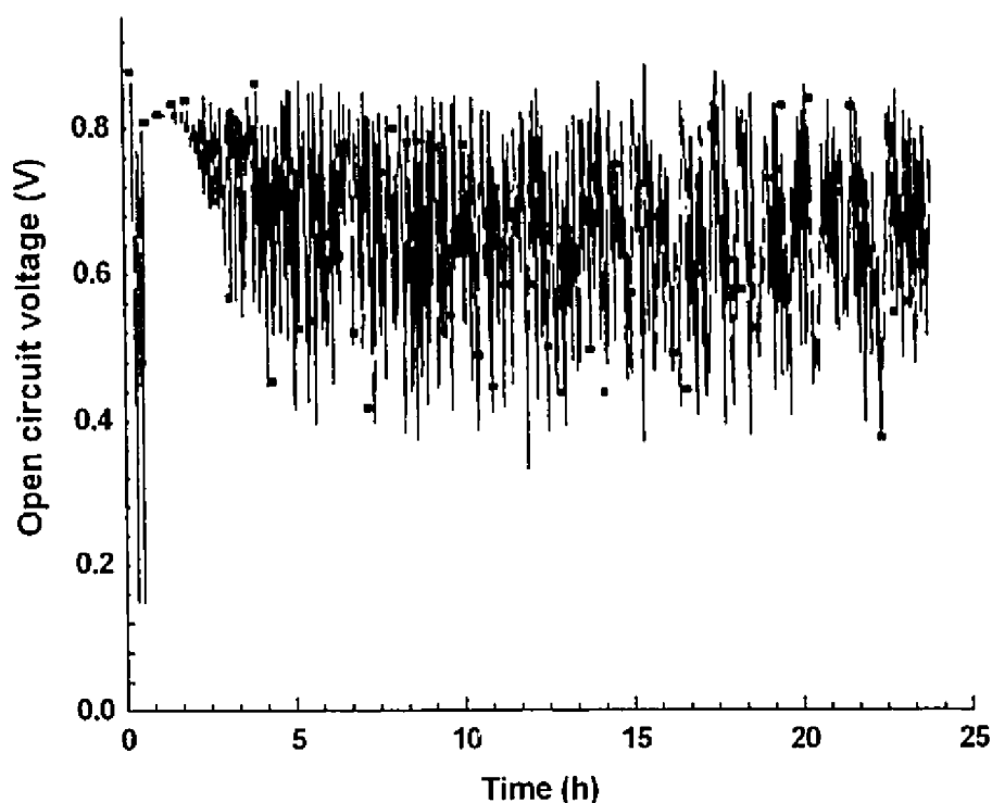
Figure 3.8: Open circuit voltage (OCV) as a function of time for aging of a direct-written SC- \mu SOFC at 700°C, R_{\text{mix}} = 2 and a total gas flow of 150 sccm. No current load was applied.
