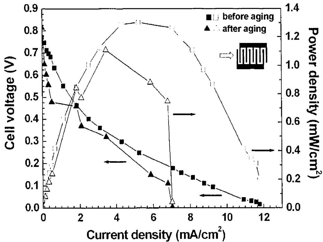
Figure 3.7: Polarization curve of SC- \mu SOFC with interdigitated electrodes (average interelectrode spacing of 517 \mu\text{m} ) at 700°C, a total gas flow of 150 sccm and a methane-to-oxygen ratio R_{\text{mix}} = 2 . The results before and after an aging period of 24 h are shown.
