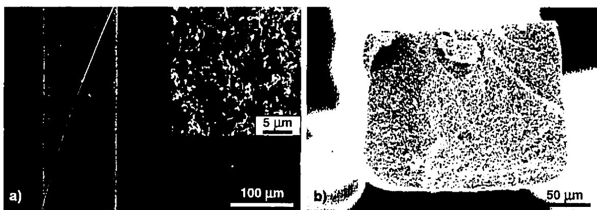
Figure A2.4: SEM images of deposited NiO-YSZ anode after sintering: a) Top view of cylindrical anode. The inset shows a close-up of the anode microstructure. b) Cross-sectional view of rectangular anode.
