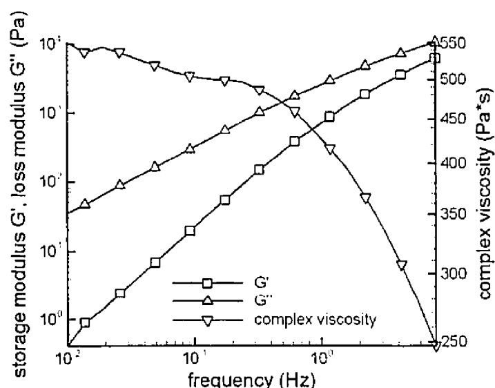
Figure A1.2: Storage modulus, G' , loss modulus, G'' , and complex viscosity as functions of frequency for 60 wt% anode suspension.
