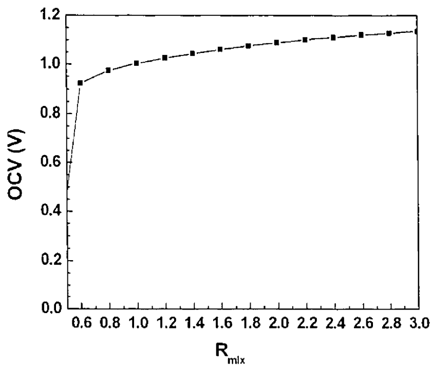
Figure 8.5: Open circuit voltage obtained from equilibrium gas calculations as a function of R_{\text{mix}} at 700°C for methane-air mixtures.
