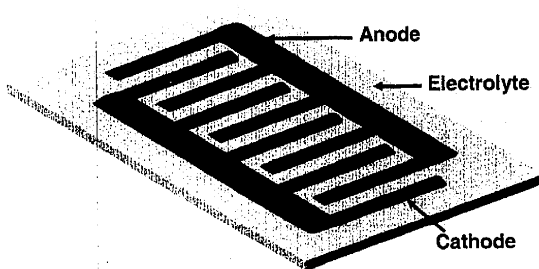
Figure 11: Schematic representation of SC-SOFC with coplanar interdigitated electrodes.
