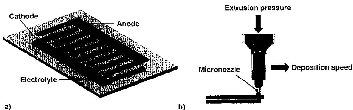
Figure 3.1: a) Schematic illustration of a single-chamber solid oxide fuel cell in single-face configuration with interdigitated electrodes. b) Schematic illustration of the robot-controlled direct-write microfabrication of electrode lines on an electrolyte plate. The quality of the deposited structures strongly depends on the two main process parameters, extrusion pressure and deposition speed.
