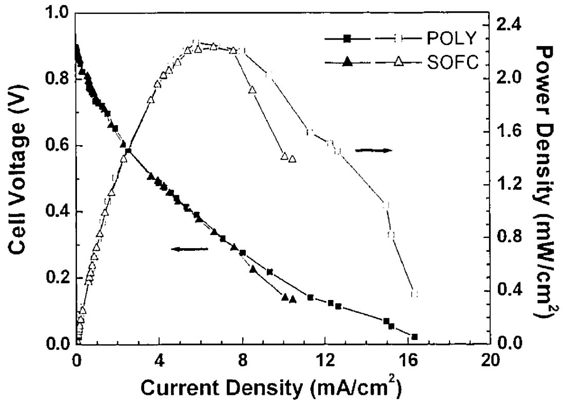
Figure 5.6: Comparison of the electrochemical performance of the "SOFC" and "POLY" geometry in a methane-air mixture with R_{\text{mix}} = 2 and a total gas flow of 150 sccm at 700^\circ\text{C} . Voltage (closed symbols) and power density (open symbols) are plotted as functions of current density. The average electrode surface area is the normalization parameter.
