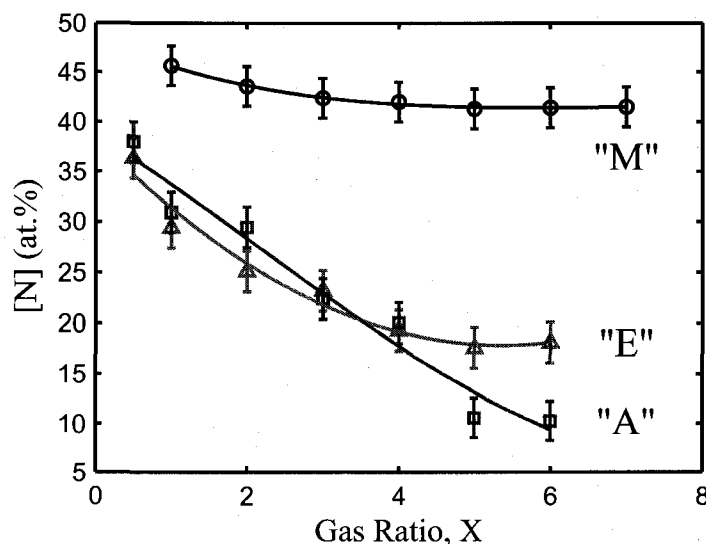
FIGURE 3.9 Concentrations of nitrogen, [N] in at.%, determined by XPS, versus gas flow ratio, X (see text), for the three PP:N families : PPM:N (« M », \circ ), PPE:N (« E », \triangle ), and PPA:N (« A », \square ).
