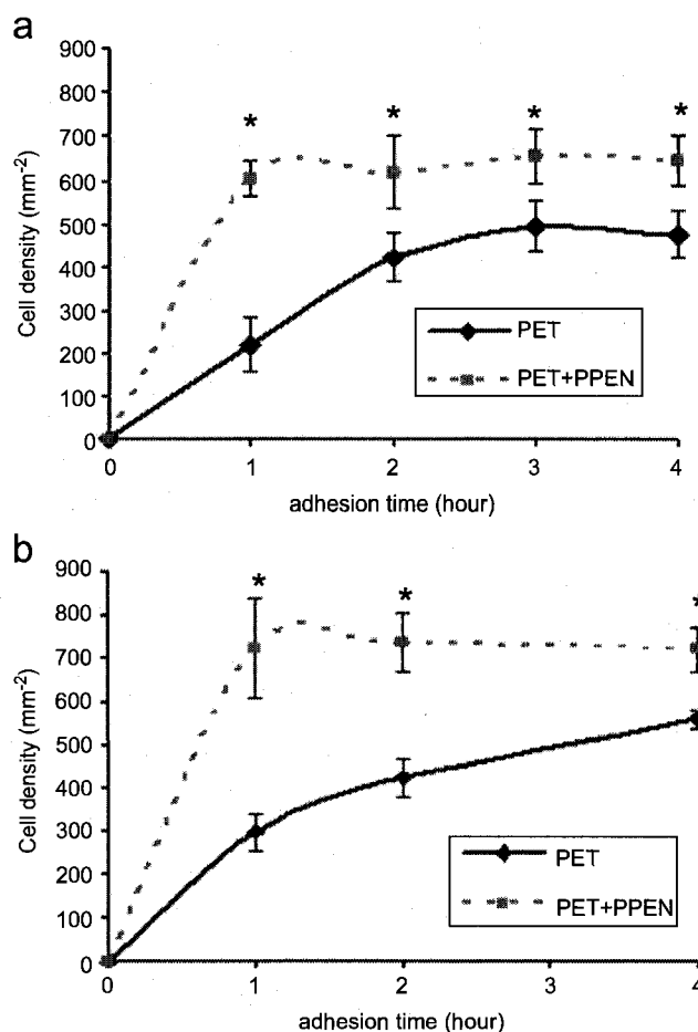
Fig. 3. Rate of adhesion of VSMC (a) and fibroblasts (b) on PPE:N-coated and control PET films, expressed as densities of cells on the surfaces after 1, 2, 3 and 4 h of incubation (* p < 0.001 , n = 6 ).
