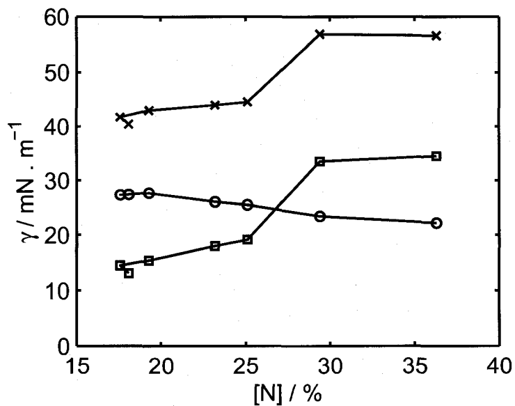
FIGURE 3.5 Surface energy ( \gamma_s, \times ) variation with [N] in PPE:N films. Polar ( \gamma_s^p, \square ) and dispersive ( \gamma_s^d, \circ ) components are also shown.
