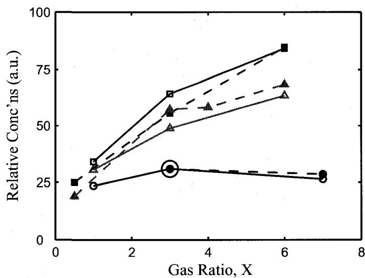
FIGURE 3.21 Composite plot of IR and NEXAFS data : IR data corresponding to relative concentrations of nitrile groups in samples from the three PP:N families, versus X (open symbols, taken from Fig. 3.19) are superimposed on the corresponding integrated NEXAFS resonance areas (full symbols, dashed lines, from Fig. 3.15) . As explained in the text, only the data points for sample PPA:N(6) (top right) were made to overlap, while all other data points then fell into the positions shown.
