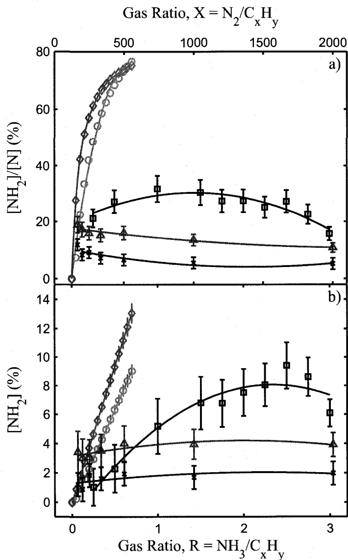
FIGURE 4.3 Contributions of primary amines to the total nitrogen content, [NH_2]/[N] (in %), the so-called « amine selectivity », a); the total amine content per 100 atoms measured by XPS, [NH_2] (in %) (b). Results are based on XPS analyses (including chemical derivatisation), and are presented as functions of the gas flow ratios : X , for H-PPE:N ( \Delta ) and H-PPAN(x); or R , for L-PPE :N ( \square ), VUV-PE:N ( \circ ), and VUV-PM:N ( \diamond ). Solid curves serve to guide the eye. Compiled from [9, 11, 50]
