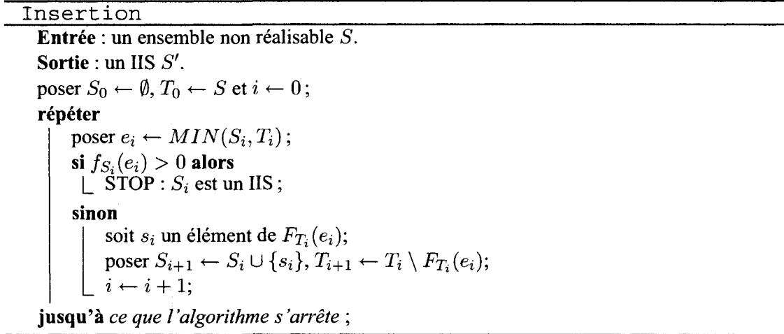
Figure 4.4 – Algorithme exact d'insertion, Insertion
