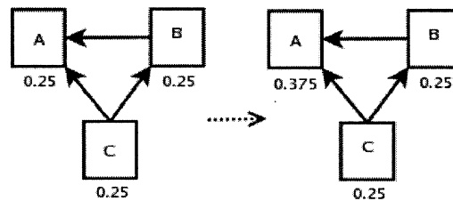
Figure 3.2 Simplified PageRank: first iteration.
