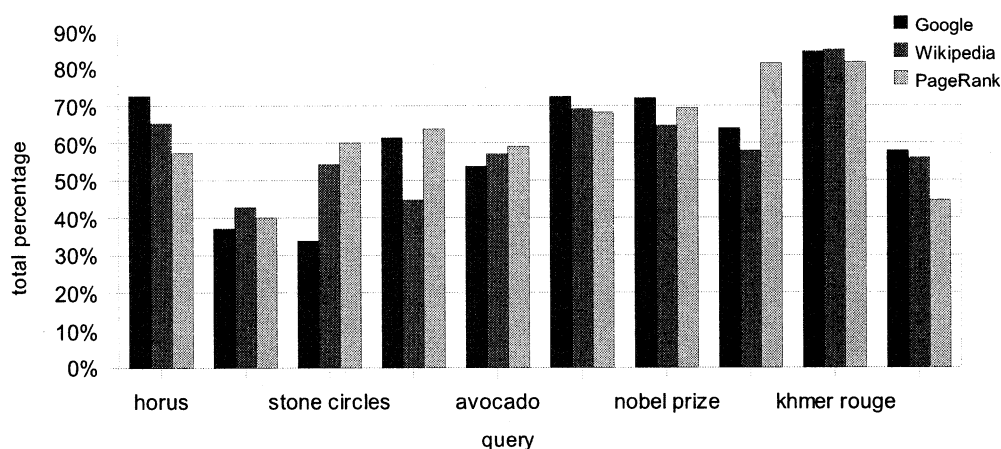
Figure 5.5 First test set: chart from Table 5.2.
