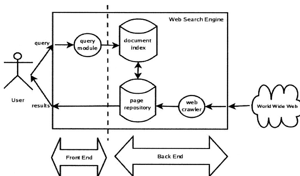
Figure 1.2 Main components of a web search engine.
