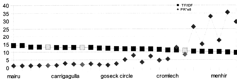
Figure 5.16 Comparison between TF/IDF and PageRank for query Stone circle.
