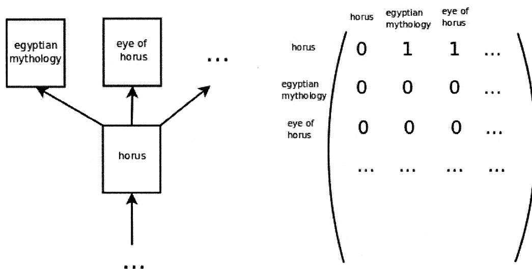
Figure 4.4 Representation of the links of Horus as a graph of forward links.
