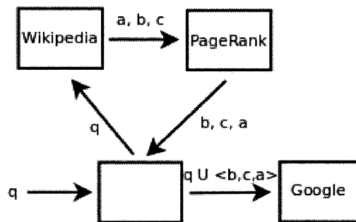
Figure 4.2 Query expansion with Wikipedia and PageRank.
