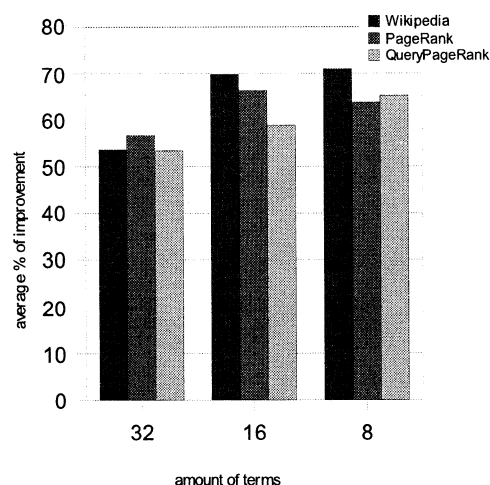
Figure 5.12 Average percentage of the improvement of our system with the next ten Google results.
