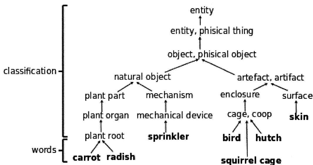
Figure 2.5 “is-a” relation example.
