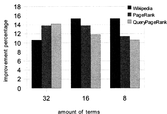
Figure 5.11 Improvement of our system with respect to the next 10 Google results.
