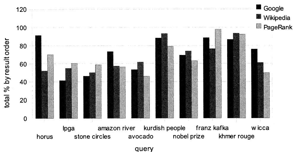
Figure 5.7 First test set: total % by result order.
