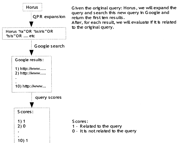
Figure 5.10 Second test set: evaluation process for the query Horus expanded with Wikipedia terms by order of QueryPageRank .
