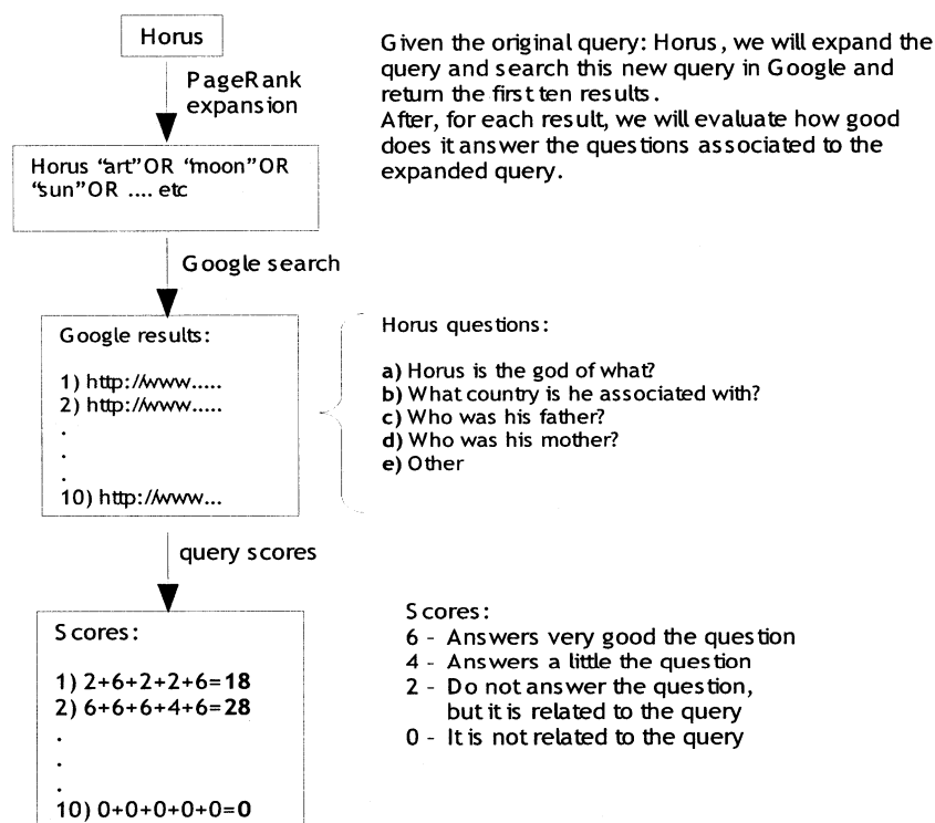
Figure 5.4 First test set: evaluation process for the query Horus expanded with terms from Wikipedia by order of PageRank.
