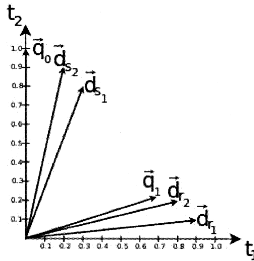
Figure 2.3 Vector model for two terms t_1 and t_2 : representing the query q , relevant documents d_{r_i} , non-relevant documents d_{s_i} .
