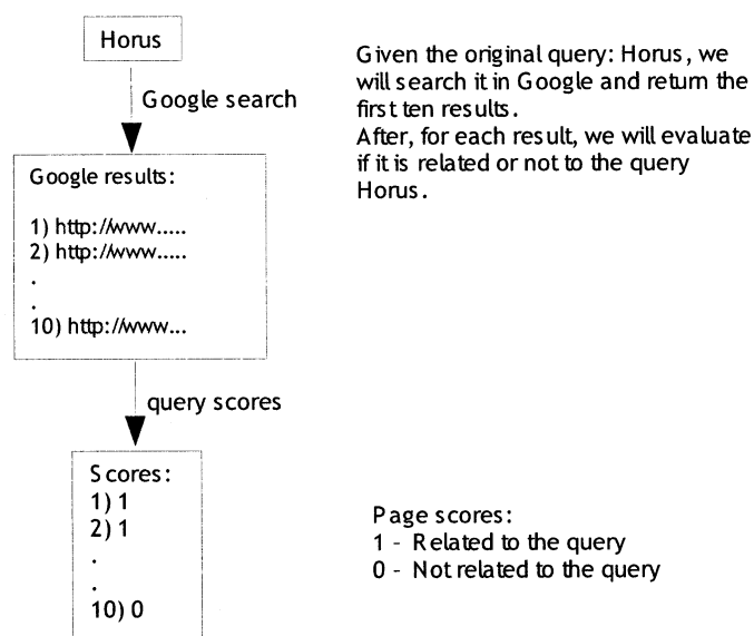
Figure 5.9 Second test set: evaluation process of the query Horus in the Google phase for the first ten results.
