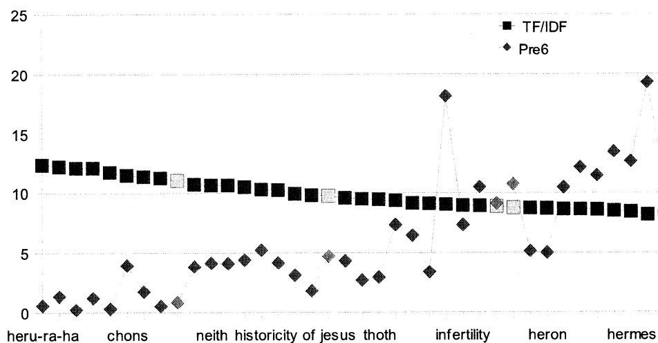
Figure 5.14 Comparison between TF/IDF and PageRank links for query Horus.
