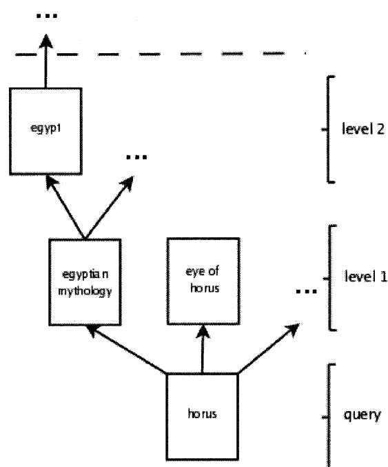
Figure 4.5 QueryPageRank for the query Horus.
