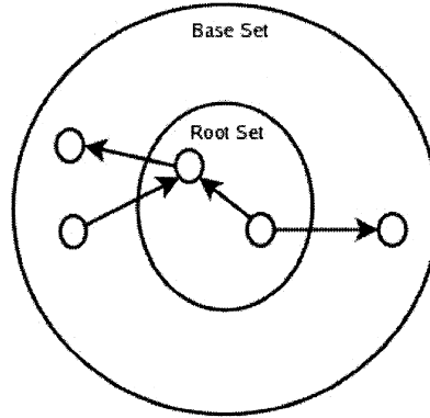
Figure 3.4 Creation of the base set from the root set.
