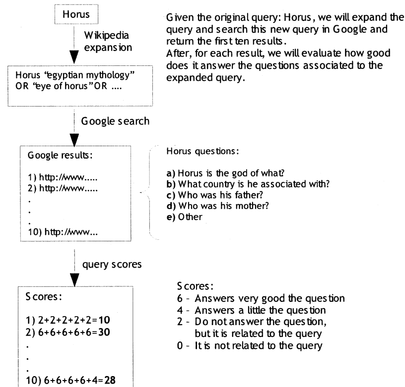
Figure 5.3 First test set: evaluation process for the query Horus expanded by Wikipedia terms by order of appearance.
