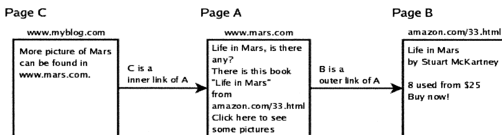
Figure 1.3 The linked structure of the web: a three pages example.
