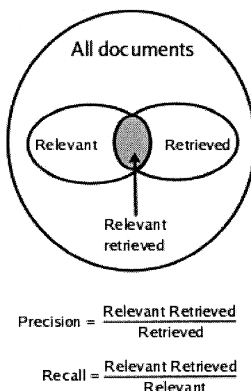
Figure 2.1 Precision and Recall.
