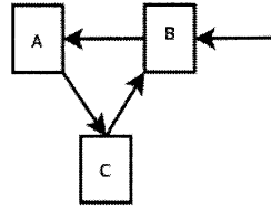
Figure 3.3 Loop that acts as a Rank Sink.
