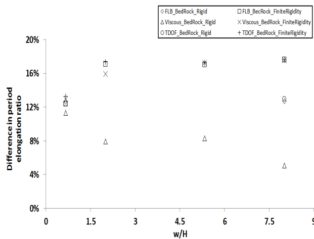
Figure 5 summarizes the values of the difference between theoretical and numerical ratios of period lengthening. As it can be seen, increasing the value of \varpi did impact the values. When the bedrock was considered rigid, the ratio did not change for the TDOF lateral boundaries. The ratio decreases in the case of the viscous lateral boundaries. When the finite rigidity of the bedrock was modelled, all types of models converged with increasing value of width up to a maximum of about 7.6%.
