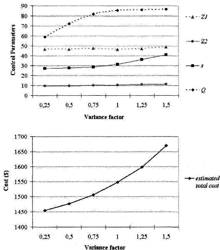
Figure 5.6 Effect of the variance on the control policy and on the estimated cost
