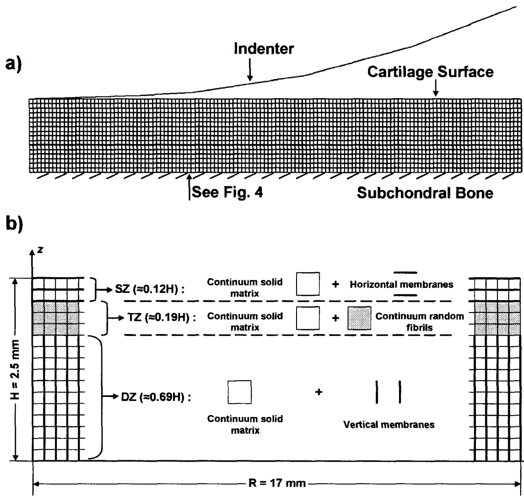
Figure 3. 1 a) Axisymmetric model of the articular cartilage along with nonporous rigid indenter b) Detailed finite element mesh showing the distinct structures representing solid matrix and collagen fibril networks in the superficial (SZ), transitional (TZ) and deep (DZ) zones.
