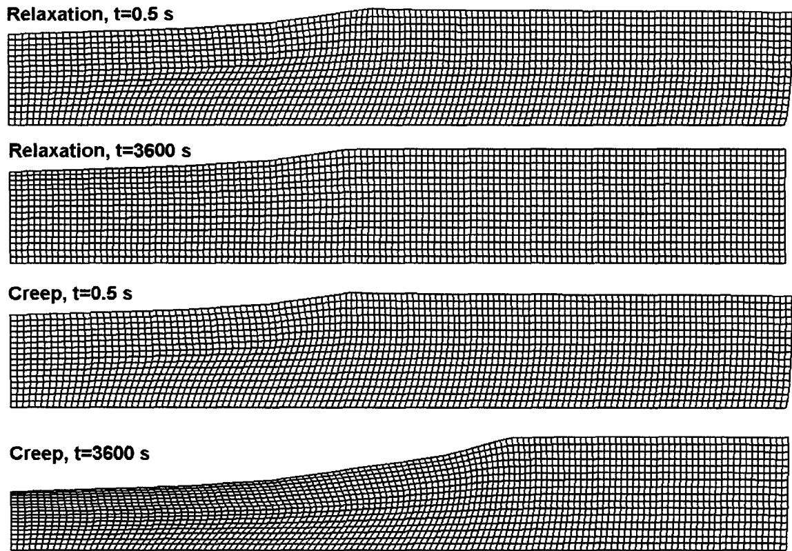
Figure 3. 5 Deformed meshes of the reference model with 9% volume content for the vertical fibrils. (a) Relaxation model at transient t=0.5 s, (b) Relaxation model at t=3600 s, (c) Creep at transient t=0.5 s and (d) Creep at t=3600 s.
