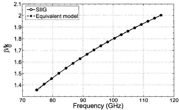
Figure 1.24 Comparison of the dispersion of the actual SIIG and its optimized equivalent model. Parameters of the equivalent are w_{\text{eff}} = 540 \mu\text{m} ( w = 510 \mu\text{m} ) and \epsilon_{r,\text{eff}} = 3.7 .
