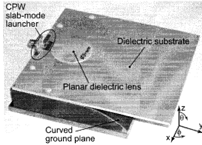
Figure 3.24 Photograph and part description of the realized slab-mode antenna prototype.
