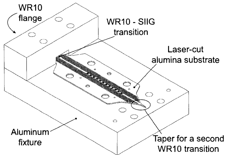
Figure 3.18 SIIG array antenna mounted on an aluminum base for measurement purposes. During measurements in the anechoic chamber, the base and the transition were clad with absorber material to avoid reflections and induced surface currents that would disturb the radiation pattern.
