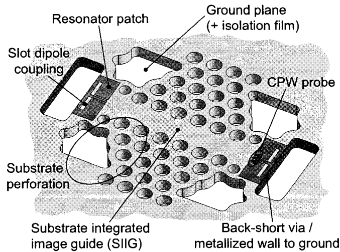
Figure 2.3 Back-to-back configuration of the proposed CPW-to-SIIG transition.
