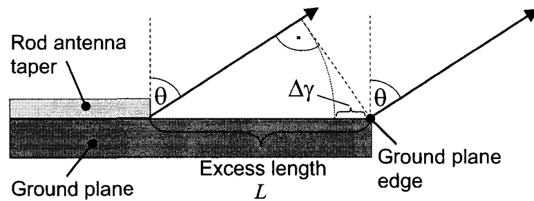
Figure 3.5 Interference and phase retardation of scattered waves from the ground plane edge, which gives rise to side lobes.
