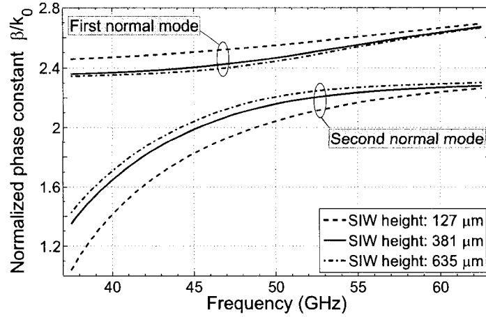
Figure 5.25 Phase constants of the first two normal modes with the SIW height d as a parameter. The coupling strength increases with decreasing d .
