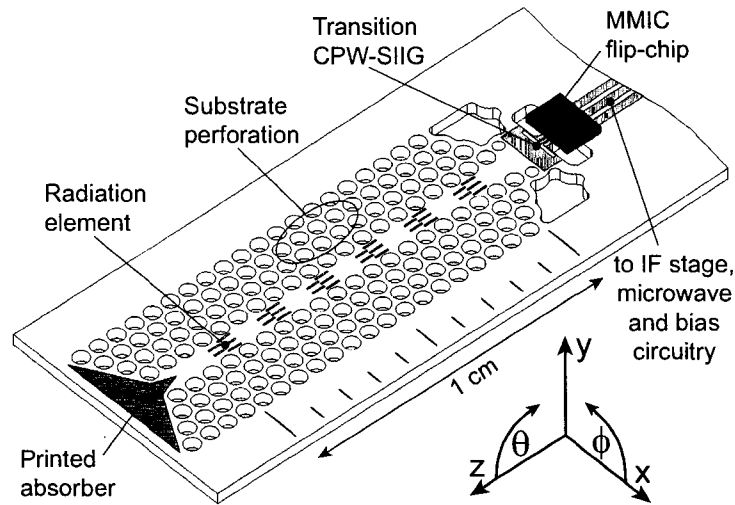
Figure 3.10 Conceivable low-loss assembly of an MMIC on an SIIG array antenna.
