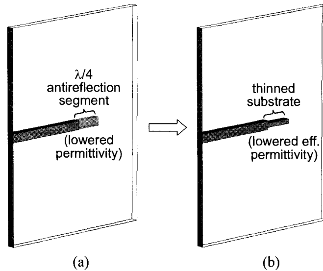
Figure 3.26 Antireflection segment at the substrate edge: (a) \lambda/4 substrate section of lowered permittivity or (b) thinned substrate with lowered effective permittivity.
