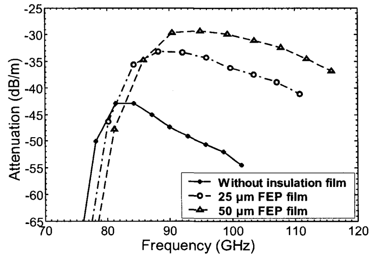
Figure 1.14 Waveguide attenuation of an HR-silicon SIIG for different insulation film thicknesses. Core dimensions: 380\text{ }\mu\text{m} \times 380\text{ }\mu\text{m} .
