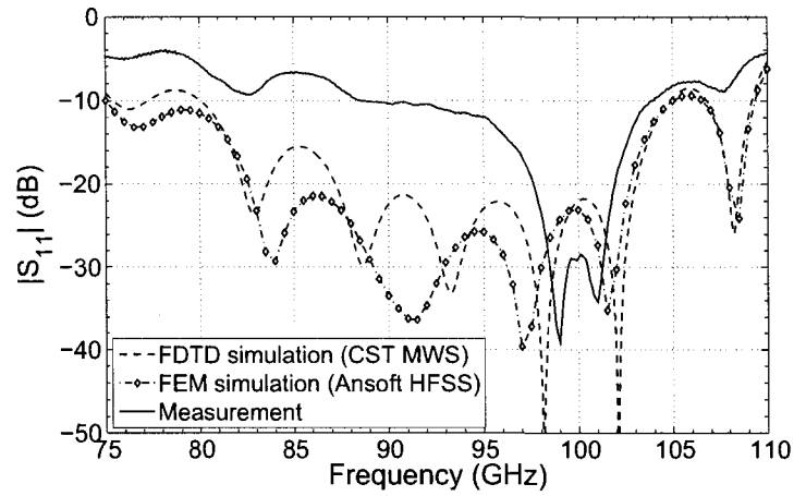
Figure 2.12 Simulated and measured return loss of the back-to-back transition. Material losses were considered in the simulations.
