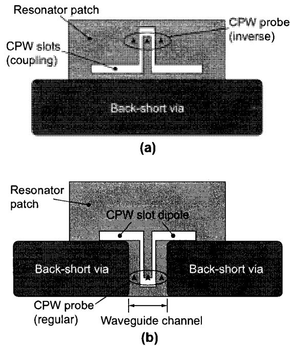
Figure 2.4 (a) Inverse dipole arrangement as used for the prototype and (b) regular configuration. Both yield almost identical performance.
