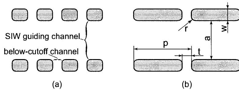
Figure 5.5 New SIW via slot configurations with (a) short slots and (b) long slots for operation below the first stop band or between the first and second stop bands, respectively.
