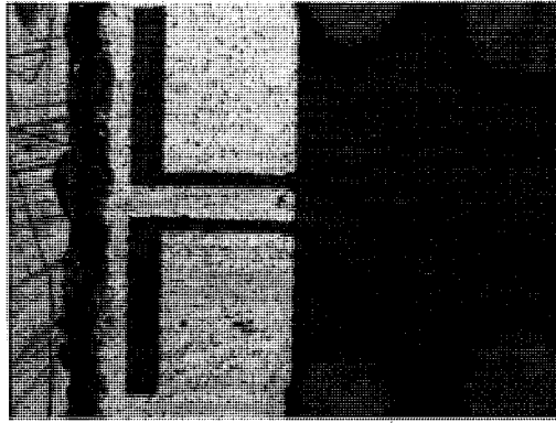
Figure 2.11 Conductive connection of the resonator patch to the back-short via with silver epoxy.
