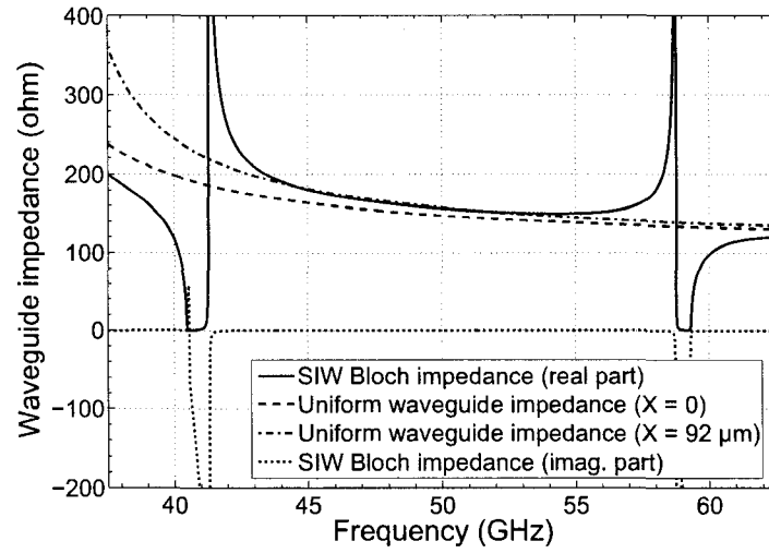
Figure 5.8 Calculated Bloch impedance of the given SIW in comparison with the characteristic impedance of uniform, dielectric-filled waveguides with equal width a and reduced width a-X .
