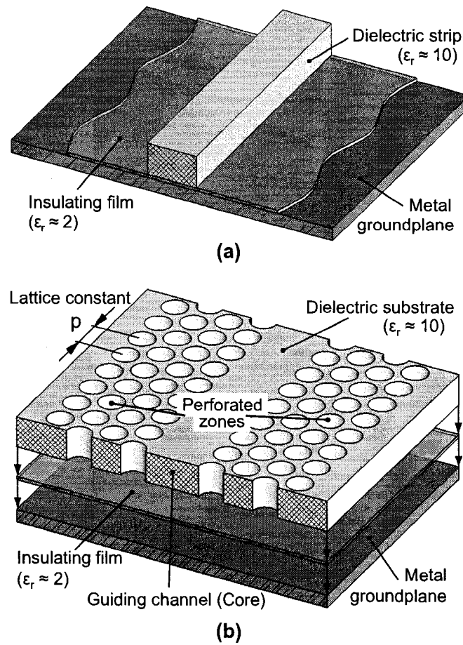
Figure 2 (a) Insulated image guide and (b) exploded view of substrate integrated image guide (SIIG).
