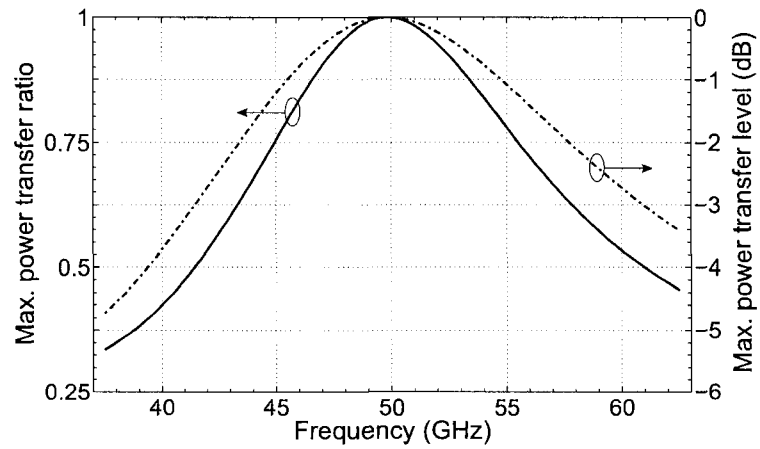
Figure 5.21 Maximum power transfer ratio and level over frequency.
