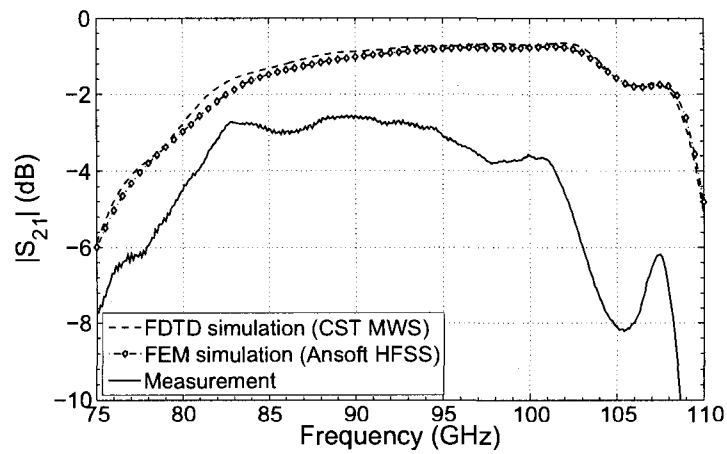
Figure 2.13 Simulated and measured insertion loss of the back-to-back transition. Material losses were considered in the simulations.
