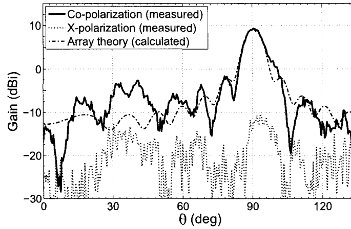
Figure 3.22 Calculated and measured E-plane radiation pattern ( \phi = 90^\circ ). The peak of the calculated curve is fit to the peak of the measured curve.
