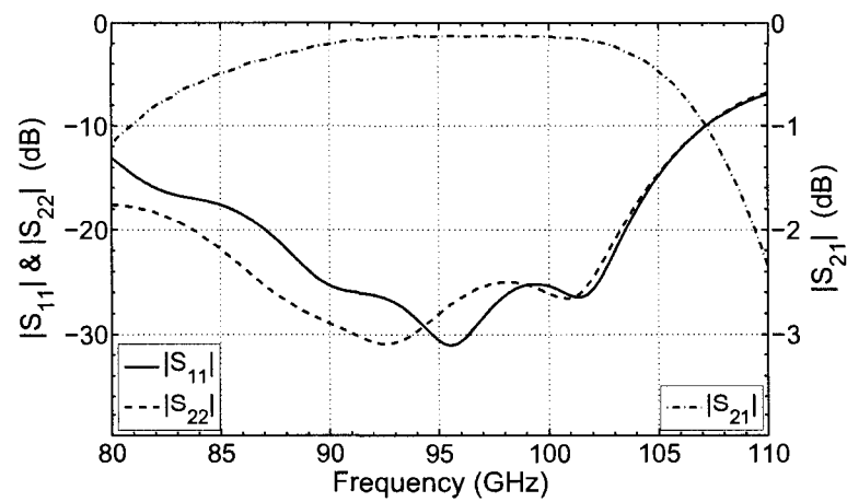
Figure 2.9 Time-domain simulation of a single transition excluding material losses. As a result, the plotted insertion loss only originates from radiation and return loss.
