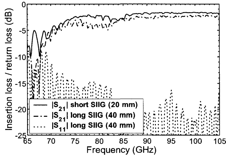
Figure 1.27 Measured insertion and return loss for the short and long SIIG sections fabricated of HR-silicon. Losses arising from the two transitions are included.
