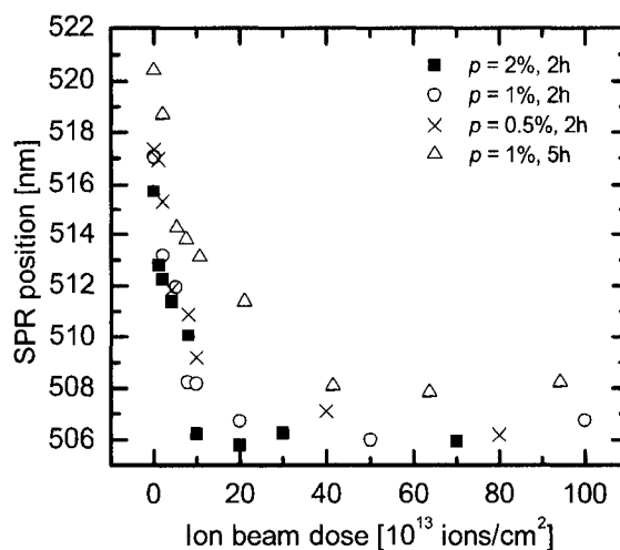
Figure 4.5 – SPR shift as a function of dose for 3 different gold concentrations ( p = 0.5 vol. %, 1 vol. % and 2 vol. %). The films were annealed at 900^\circ\text{C} for different annealing times prior to ion irradiation as indicated.
