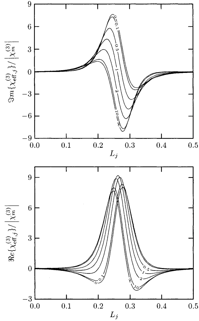
Figure 6.9 – Normalized \Im\{\chi_{\text{eff},j}^{(3)}\} and \Re\{\chi_{\text{eff},j}^{(3)}\} plotted as a function of L_j for different values of the \Im\{\chi_m^{(3)}\}/\Re\{\chi_m^{(3)}\} ratio.
