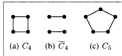
Figure 6.15 An illustration of the FSC algorithm for the class of split graphs, using \mathcal{G}^8 as search space.
