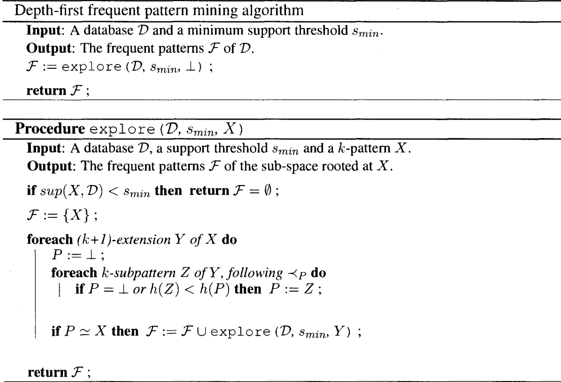
Figure 5.1 Our approach to depth-first frequent pattern mining.
