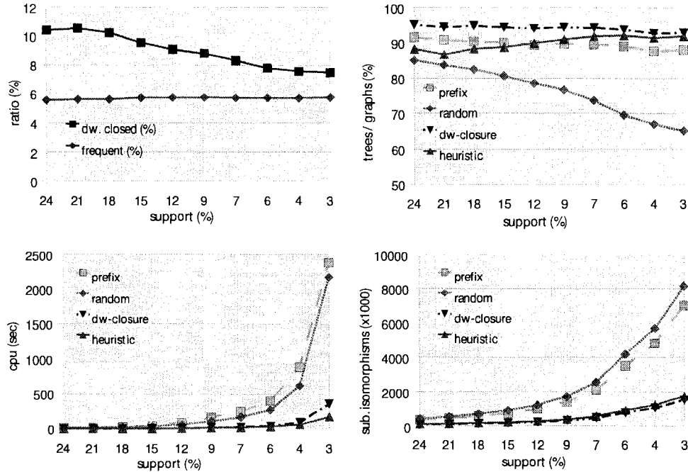
Figure 5.6 Ratio of downward closed and frequent visited graphs ( top left ), ratio of visited graphs that are trees ( top right ), runtimes ( bottom left ) and number of subgraphs isomorphism tests performed ( bottom right ), for the tested algorithms on the Predictive Toxicology Evaluation (PTE) dataset.
