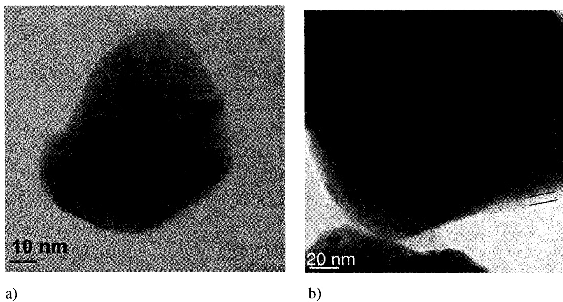
Figure 6.7. TEM images of a) original and b) coated zirconia nanoparticles
