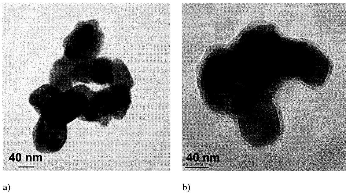
Figure 4.5. TEM images of a) original and b) coated zirconia agglomerate
