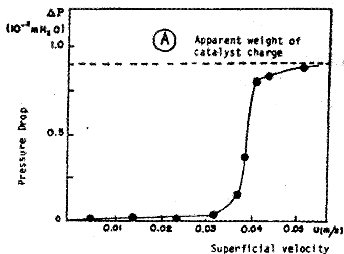
Fig. 1.8 Pressures drop of \text{CuO}/\text{Al}_2\text{O}_3 (Chaouki et al. 1985)
