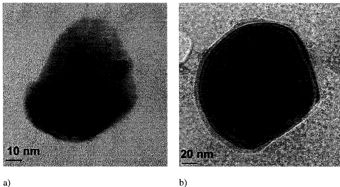
Figure 4.4. TEM images of a) original and b) coated zirconia nanoparticles
