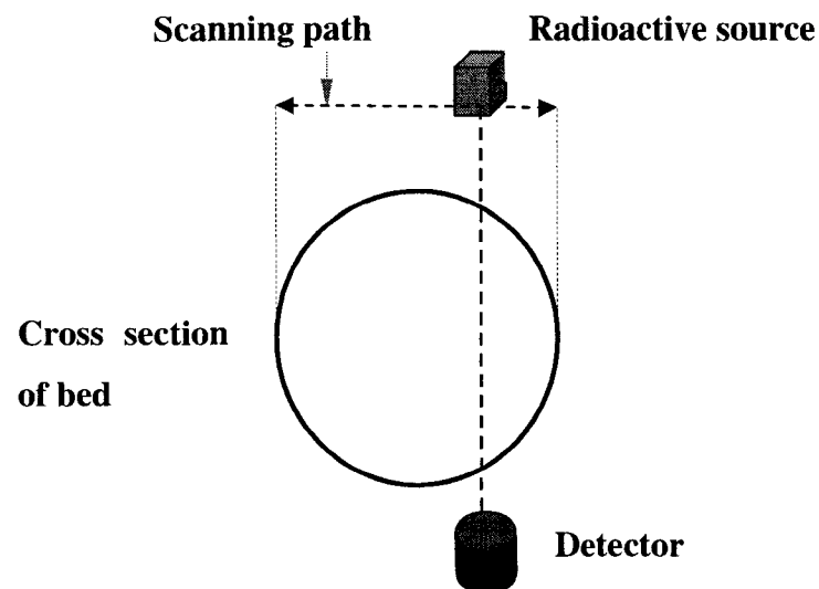
Figure 2.8 \gamma - ray densitometry
