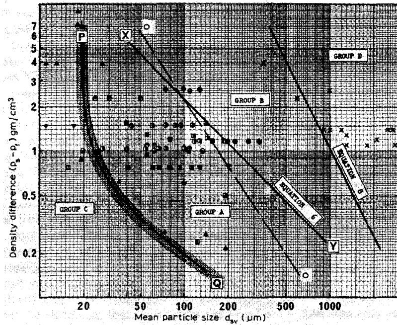
Fig. 1.5 Geldart classification of particle fluidization (Geldart, 1973).
