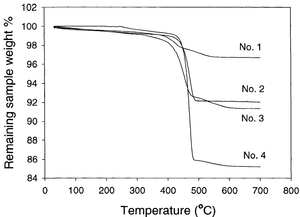
Figure 6.10. TGA graphs of zirconia encapsulation in different operations
