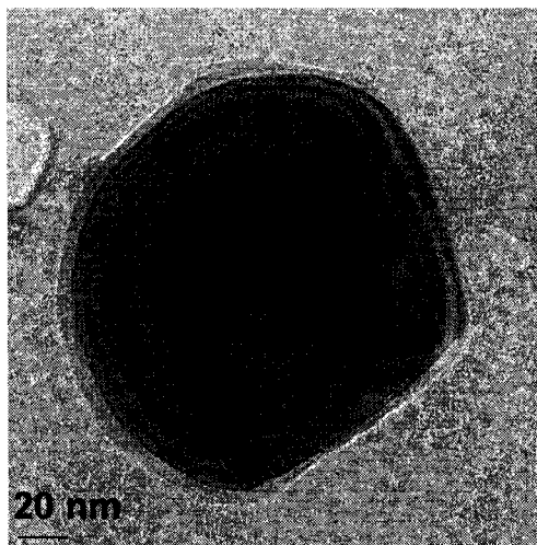
Fig. 1.4 TEM image of polymer coated zirconia (Esmaeili et al. 2006).
