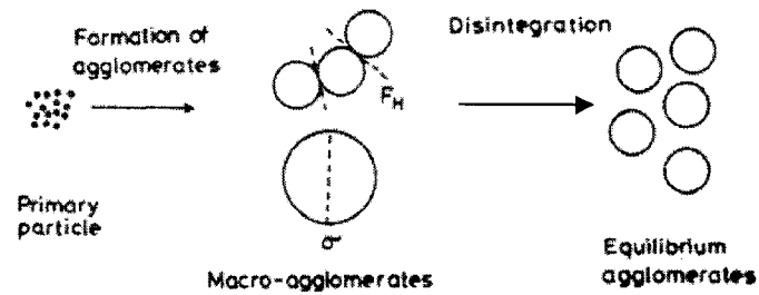
Fig. 1.14 Model for formation of equilibrium agglomerates (Morooka et al. 1988)
