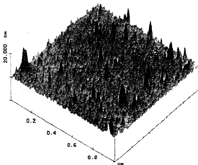
Fig. 1.3 AFM image of polymer –grafted silicon surface (Rovira-Bru et al. 2001).
