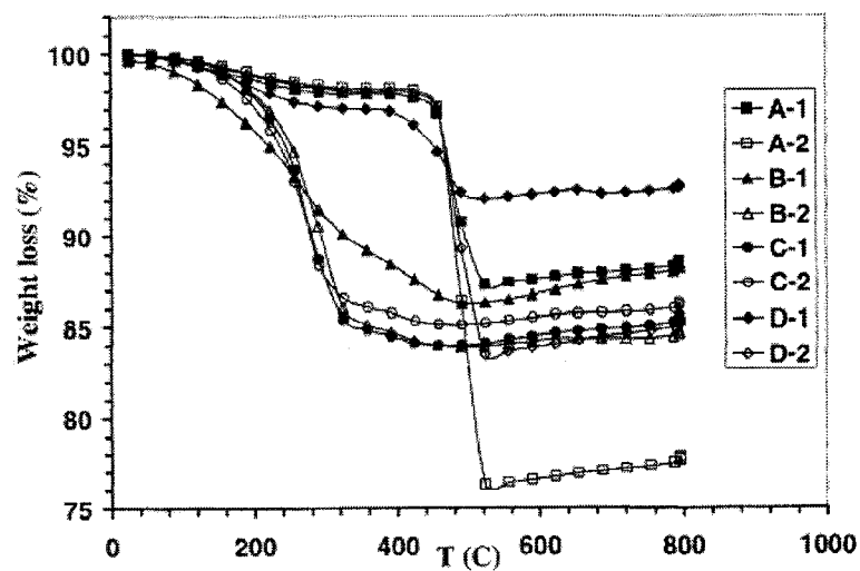
Fig. 1.1 TGA of samples of polyethylene coated aluminum (Roy et al. 2004).
