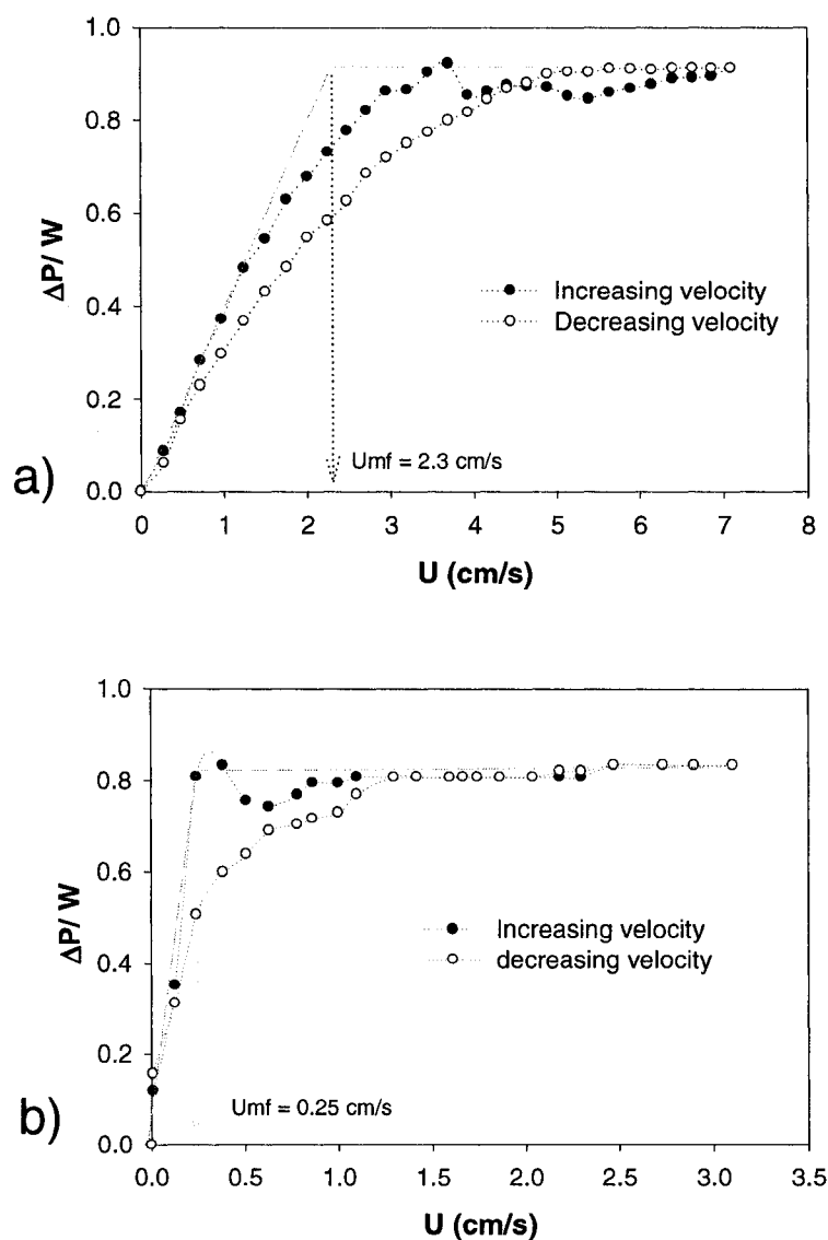
Figure 6.9. Minimum fluidization velocities for a) zirconia and b) aluminum nanoparticles
