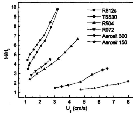
Fig. 1.11 Homogenous expansion of the fluidized bed (Yao et al. 2002).
