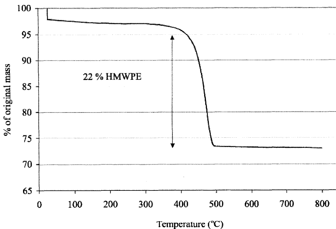
Figure 4.3. TGA graph of coated zirconia nanoparticles
