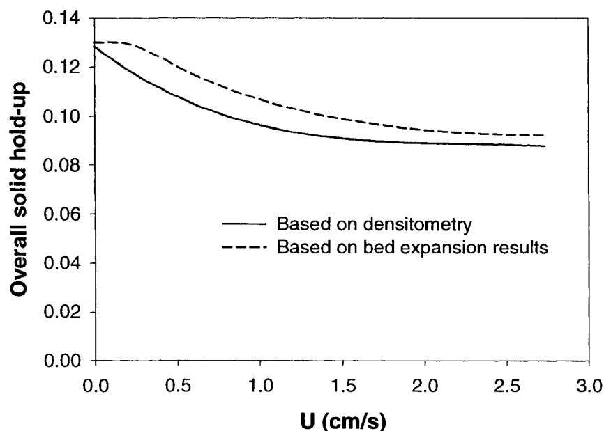
Figure 5.17. The comparison between overall solid-holdup obtained by densitometry and bed expansion results for aluminum nanoparticles
