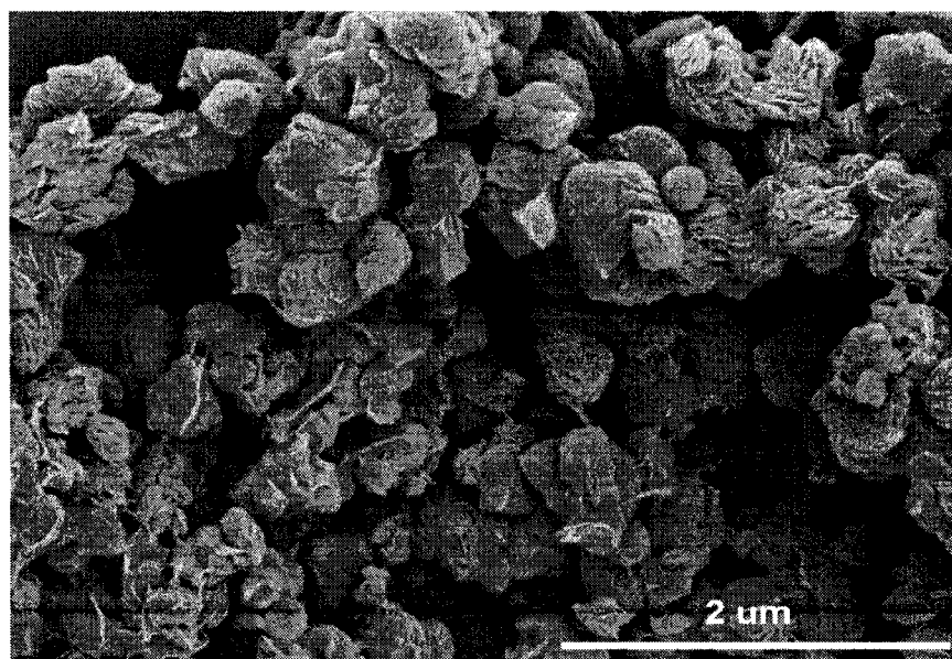
Figure 4.6. SEM image of original zirconia nanoparticles
