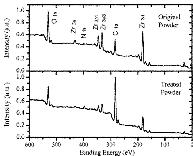
Fig. 1.2 Compared XPS results in survey binding energy scan between untreated and treated powders (He et al. 2004)
