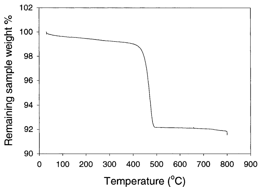
Figure 6.3. TGA graph of zirconia coated nanoparticles (Reaction conditions T = 65°C, P = 210 kPa)
