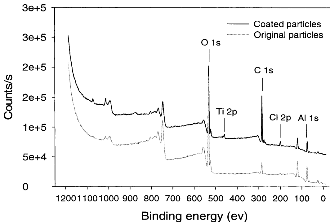
Figure 6.5. XPS graphs of original and coated aluminum nanoparticles
