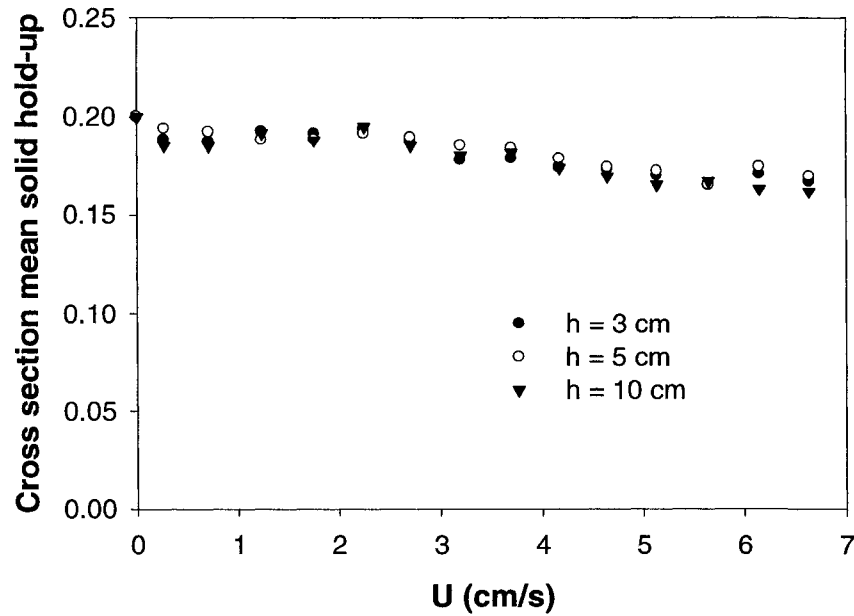
Figure 5.9. Cross section mean solid hold-up for zirconia nanoparticles
