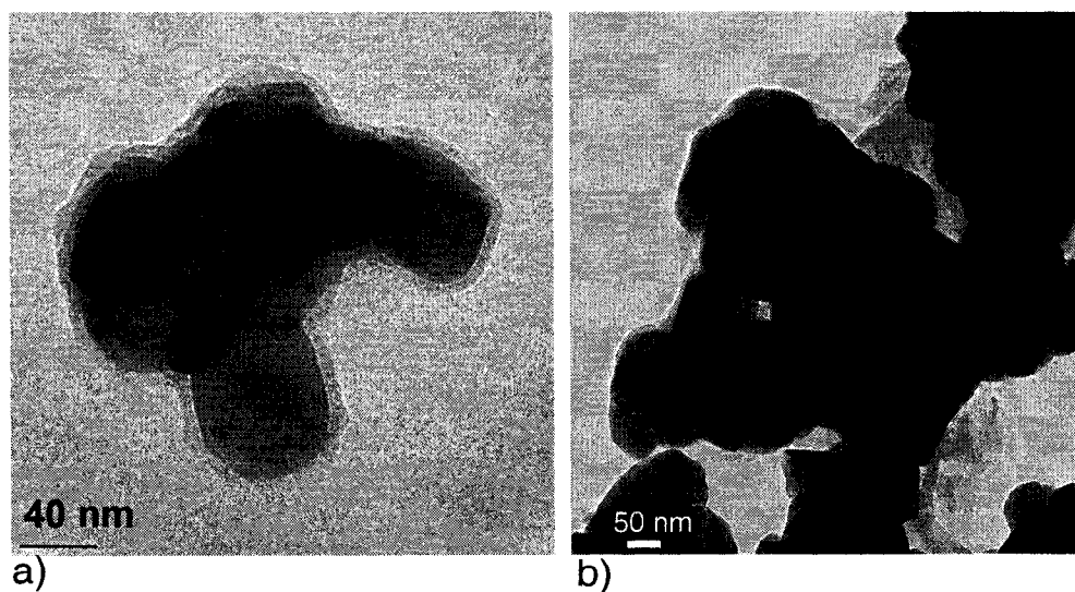
Figure 6.11. Coated agglomerates of zirconia in a) slurry phase and b) in fluidized bed
