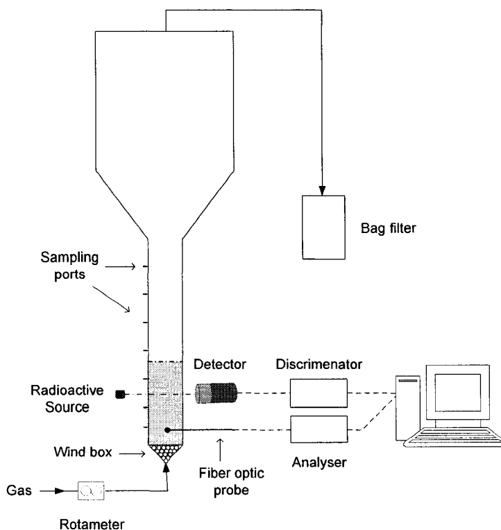
Figure 5.1. Schematic illustration of a fluidized bed and its accessories
