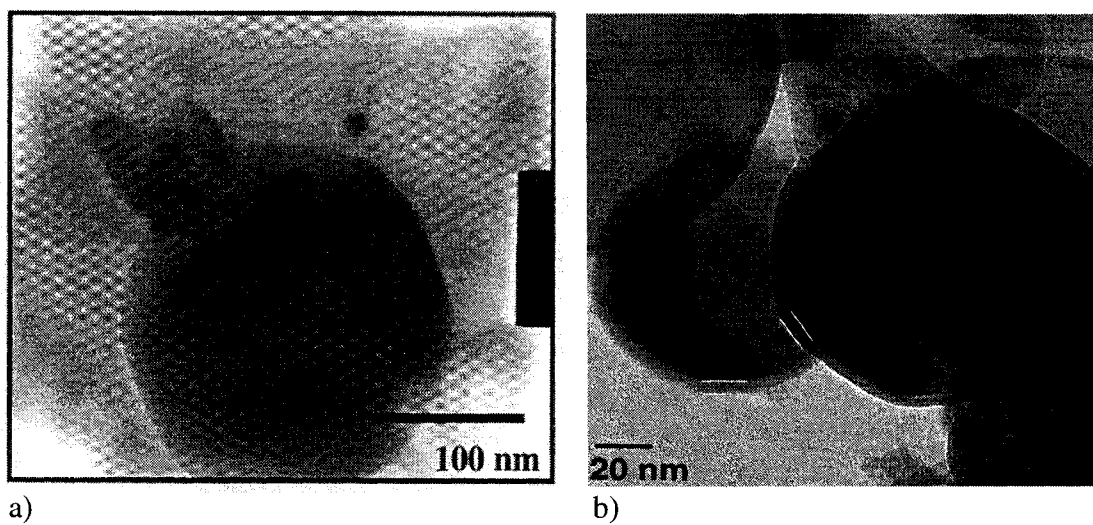
Figure 6.6. TEM images of a) original and b) coated aluminum nanoparticles
