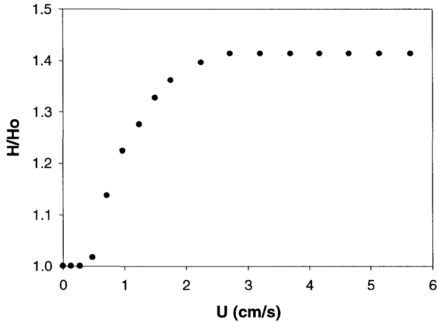
Figure 5.19. Bed expansion for titania nanoparticles.
