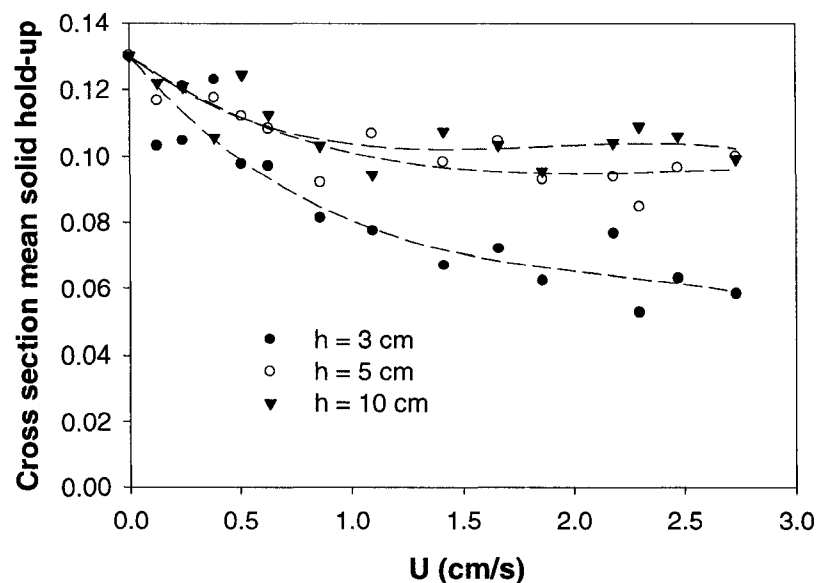
Figure 5.16. Cross section mean solid hold-up for aluminum nanoparticles
