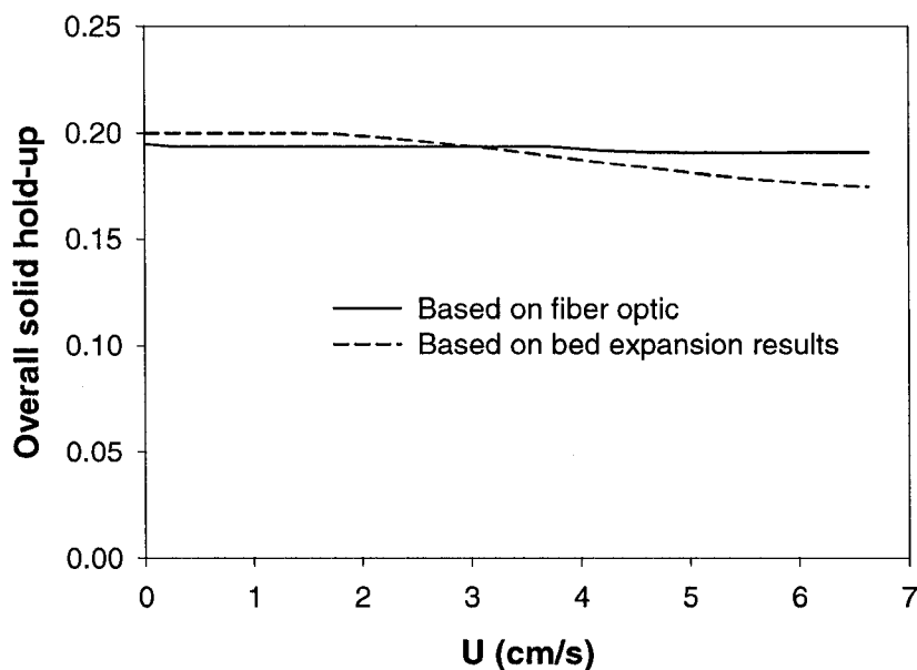
Figure 5.13. The comparison between overall solid-holdup obtained based on fiber optic and bed expansion results for zirconia nanoparticles.
