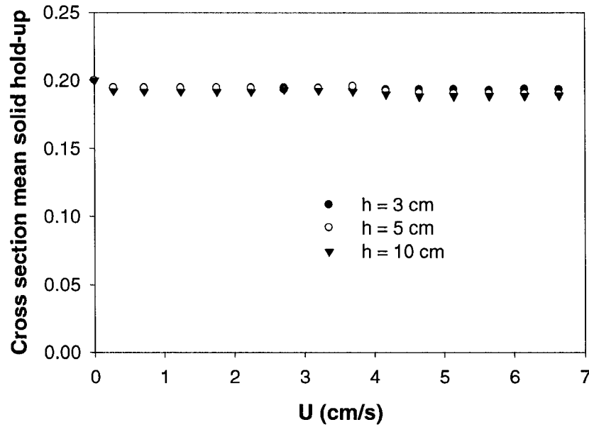
Figure 5.12. Cross section mean solid hold-up for zirconia nanoparticles
