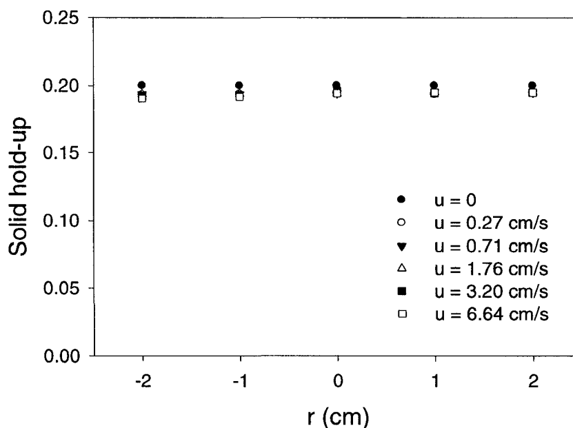
Figure 5.11. Local solid hold-up at 3 cm above the distributor for zirconia nanoparticles by fiber optic
