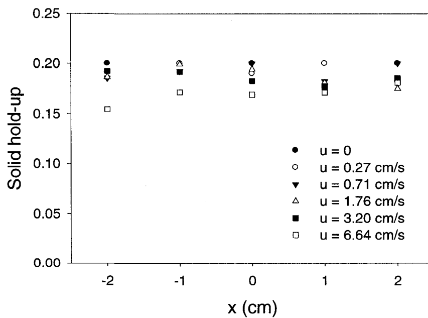
Figure 5.7. Line average solid hold-up at 5 cm above the distributor for zirconia nanoparticles by densitometry
