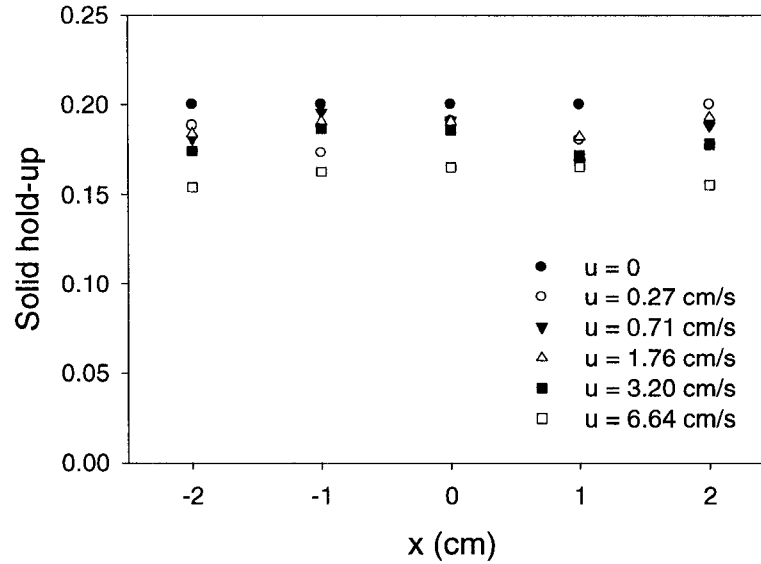
Figure 5.8. Line average solid hold-up at 10 cm above the distributor for zirconia nanoparticles by densitometry
