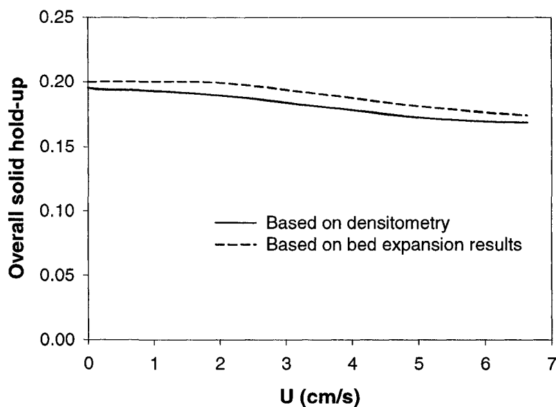
Figure 5.10. The comparison between overall solid-holdup obtained based on densitometry and bed expansion results for zirconia nanoparticles
