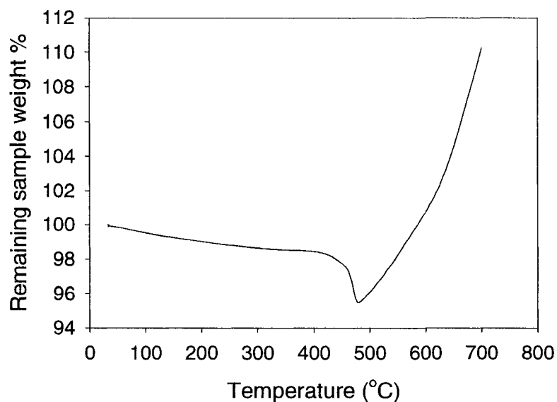
Figure 6.4. TGA graph of aluminum coated nanoparticles (Reaction conditions: T = 72 °C, P = 140 kPa)
