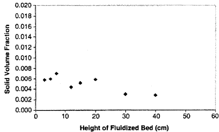
Fig. 1.13 Time-averaged solid volume fraction profile as a function of height of the fluidized bed (Jung and Gidaspow, 2002).
