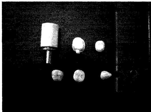
Figure 6.1. From left to right starting from the top: composite ingot, composite coping, densified coping, 3 false teeth ready to be implanted into the mouth.
