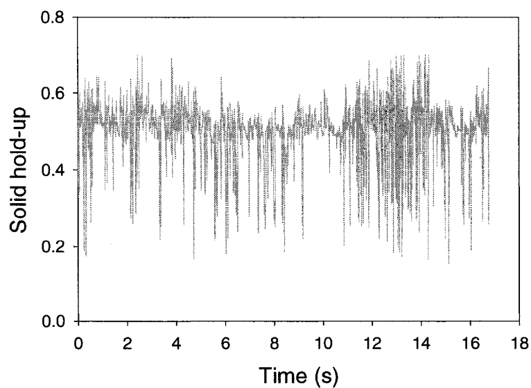
Figure 5.15. Solid hold-up for FCC fluidization at gas velocity 7 cm/s
