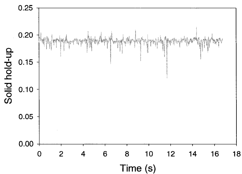
Figure 5.14. Solid hold-up for zirconia fluidization at gas velocity 7 cm/s
