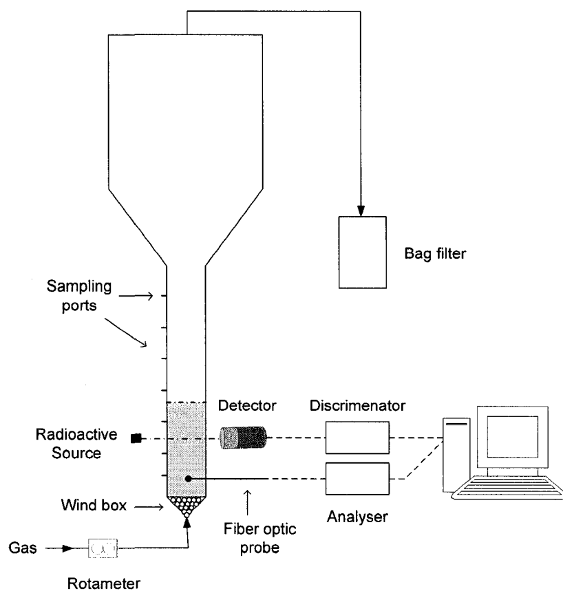
Figure 2.2 Schematic of a fluidized bed and its accessories
