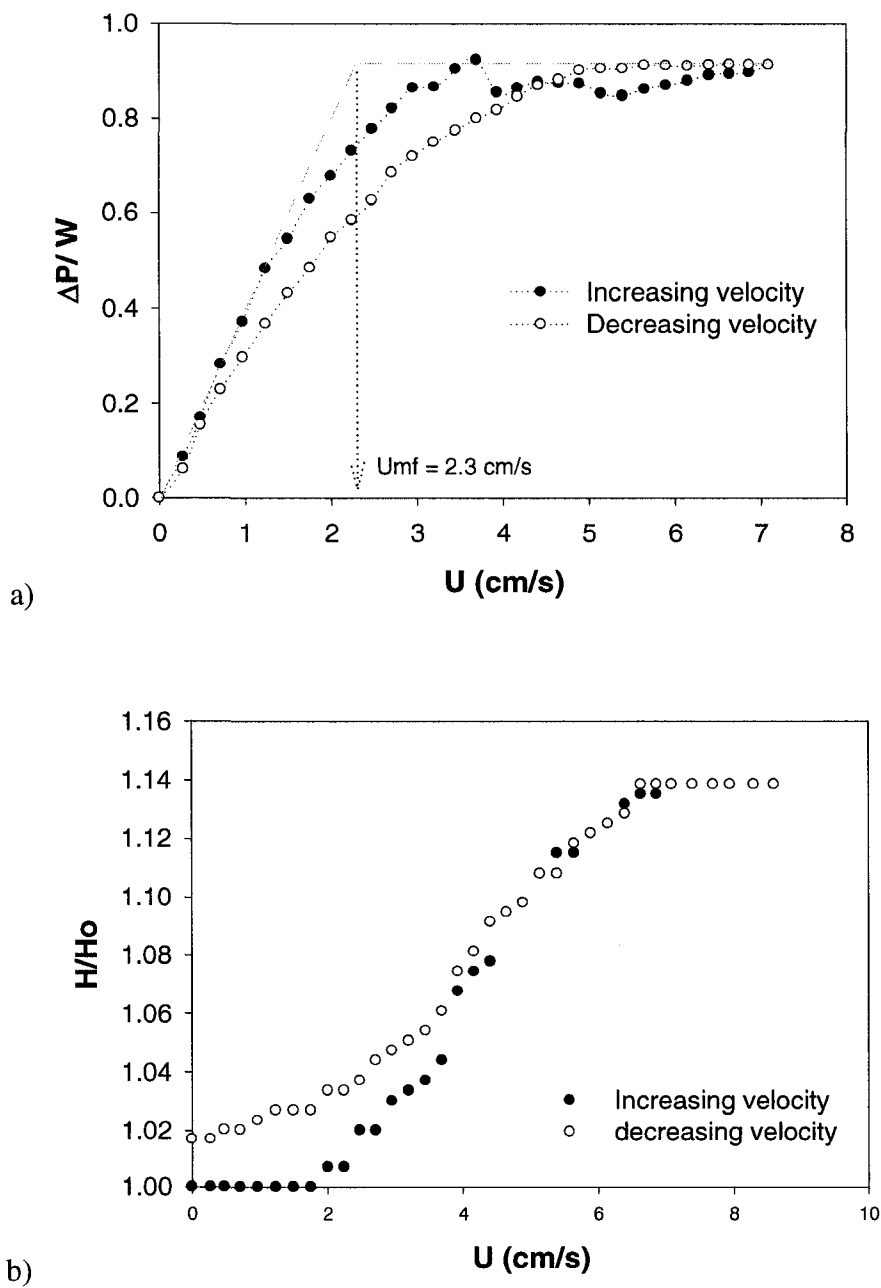
Figure 5.4. a) Normalized pressure drop and b) bed expansion for zirconia nanoparticles
