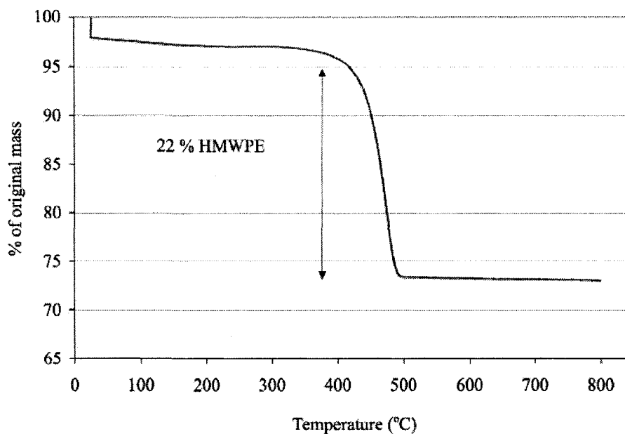
Fig. 2.4 TGA graph of polyethylene-coated zirconia nanoparticles.
