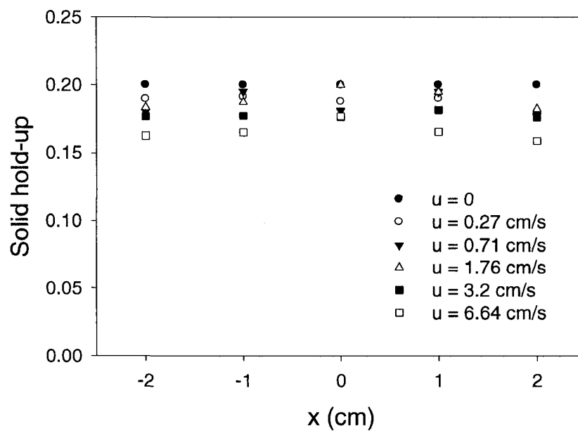
Figure 5.6. Line average solid hold-up at 3 cm above the distributor for zirconia nanoparticles by densitometry
