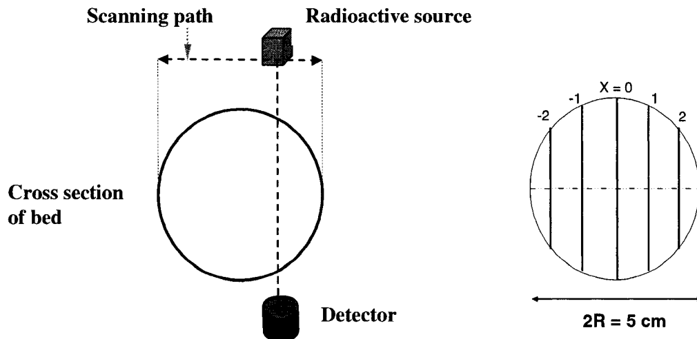
Figure 5.2. \gamma -ray densitometry and different linear positions for evaluating solid hold-up
