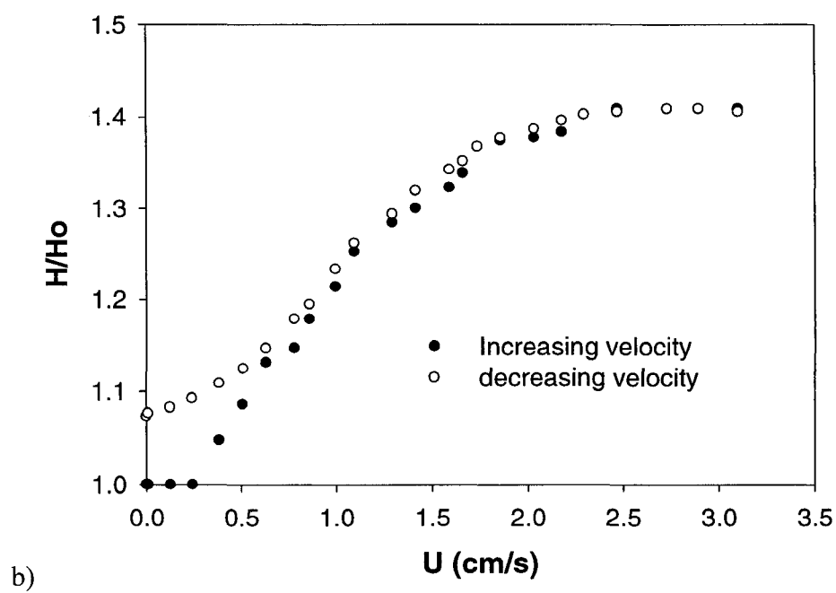
Figure 5.5. a) Normalized pressure drop and b) bed expansion for aluminum nanoparticles
