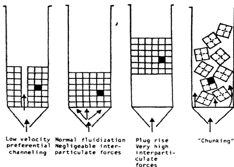
Fig. 1.9 Descriptive hydrodynamic behavior of fluidized aerogels (Chaouki et al. 1985).
