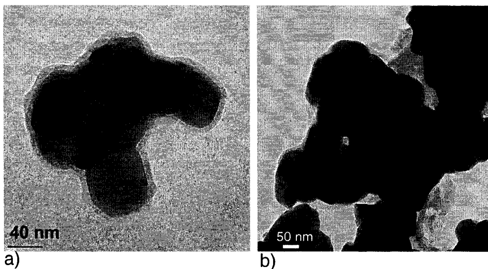
Figure 7.1. The coated agglomerates of zirconia in a) slurry phase and b) fluidized bed reactors
