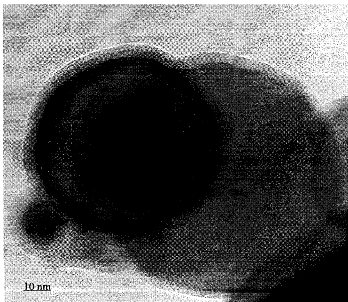
Fig. 2.5 A TEM image of polyethylene-coated aluminum nanoparticles.
