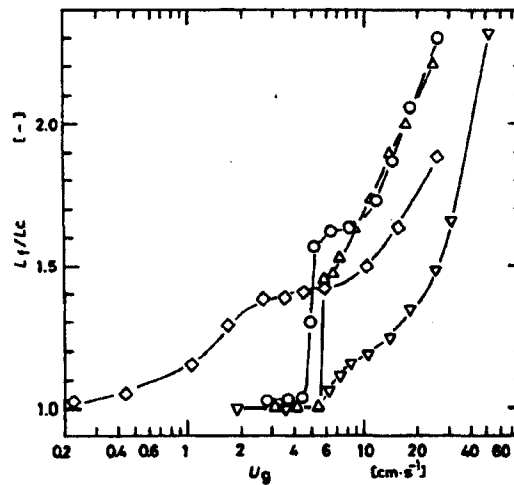
Fig. 1.10 Bed expansion across the bed (Morouka et al. 1988).
