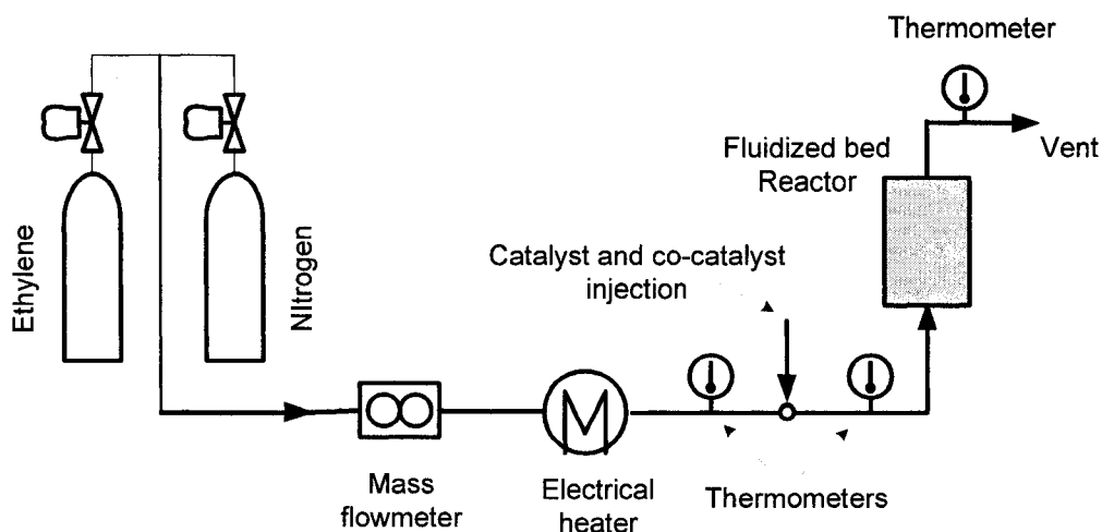
Figure 6.2. Schematic of the encapsulation of nanoparticles in fluidized bed reactor
