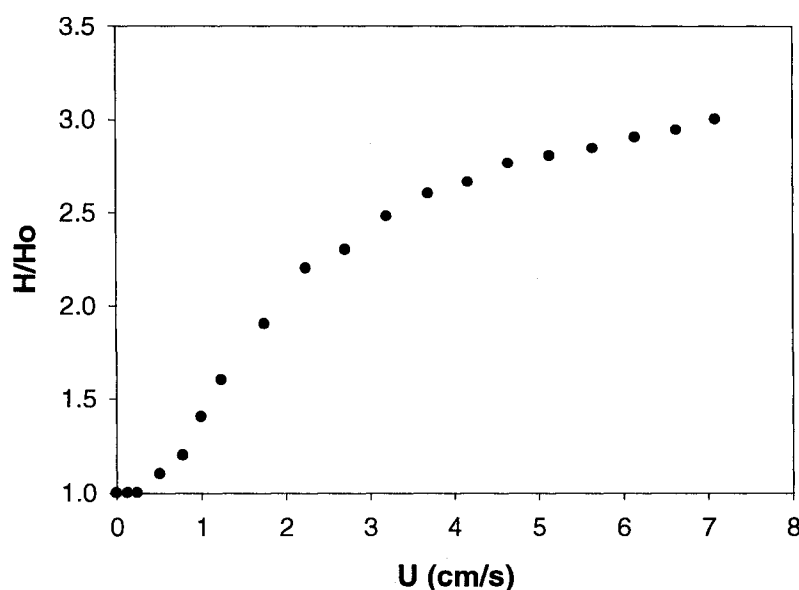
Figure 5.18. Bed expansion for fumed silica nanoparticles
