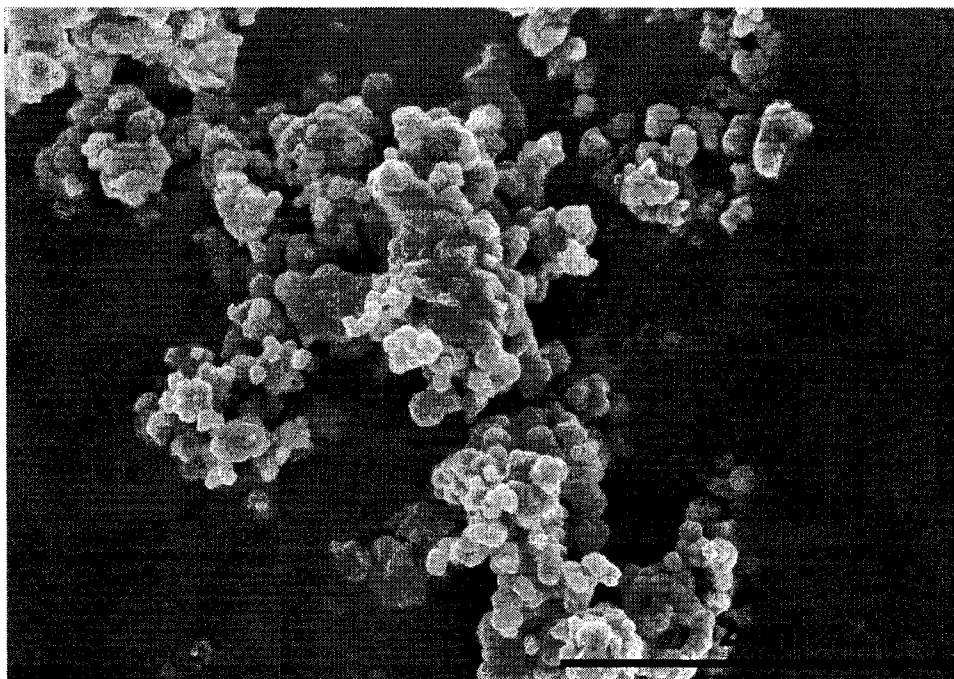
Figure 4.1. SEM image of original zirconia nanoparticles
