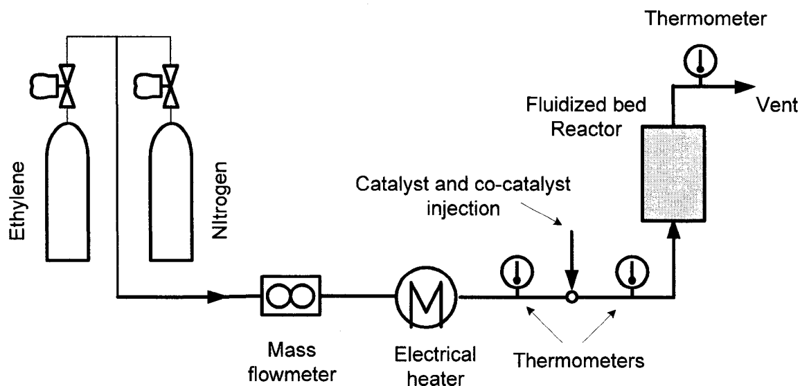
Fig. 2.3 Encapsulation of nanoparticles in a fluidized bed reactor
