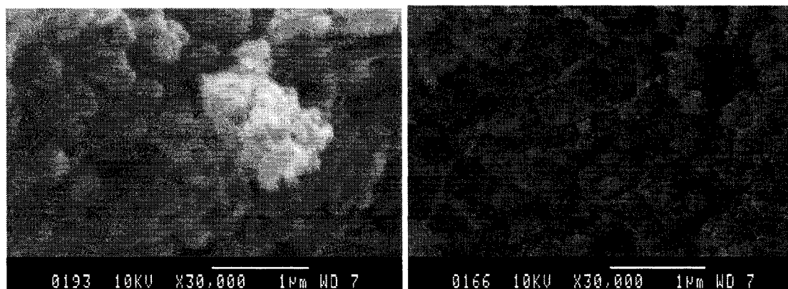
Fig 2.6 SEM images of polyethylene-coated aluminum nanoparticles.
