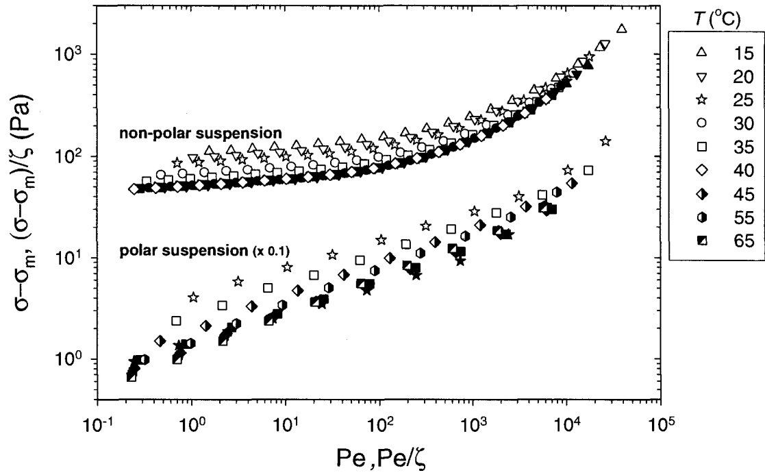
Figure 5.8 : Temperature dependency of \sigma - \sigma_m (unfilled and semi-filled symbols) and its scaling behavior (filled symbols) for the non-polar suspension prepared by ultrasonication ( \phi = 0.04 ) and the polar suspension ( \phi = 0.003 ).
