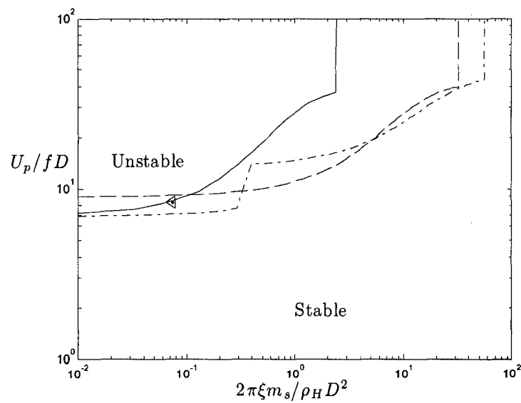
Figure 5.2 Stability boundary for a single-flexible tube model in air-water flow \beta = 80\% with \mu = 1 (—), \mu = 3 (---) and \mu = 5 (- - -). The abscissa is calculated using structural mass and damping; ( \triangle dynamic tests).
