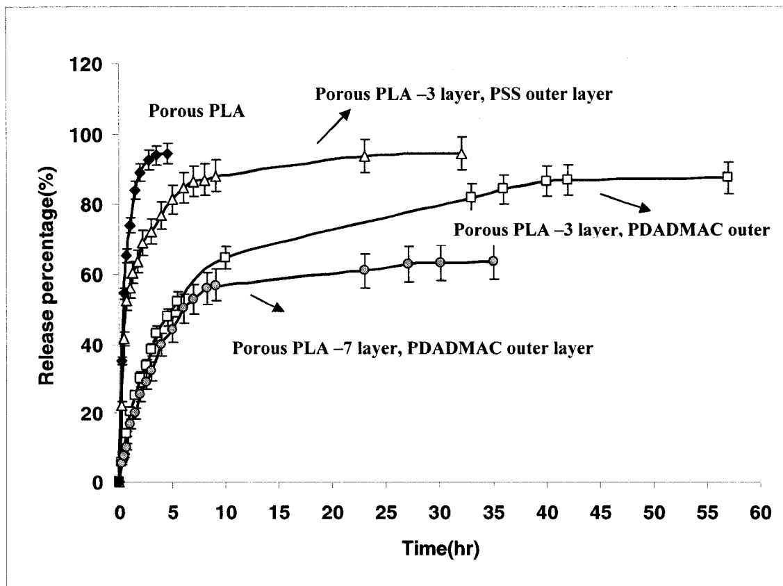
Figure 4.9 Drug release profile of Porous PLA of 1.56 \mu\text{m} (♦); PLA/PSS/PDADMAC/PSS ( \Delta ); PLA/PDADMAC/PSS/PDADMAC/BSA ( \square ); PLA/PDADMAC/PSS/...PDADMAC 7layer/BSA ( \bullet )
