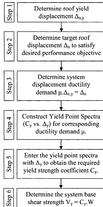
FIG. 3.18 Flowchart of YPS method (Aschheim, 2000).
