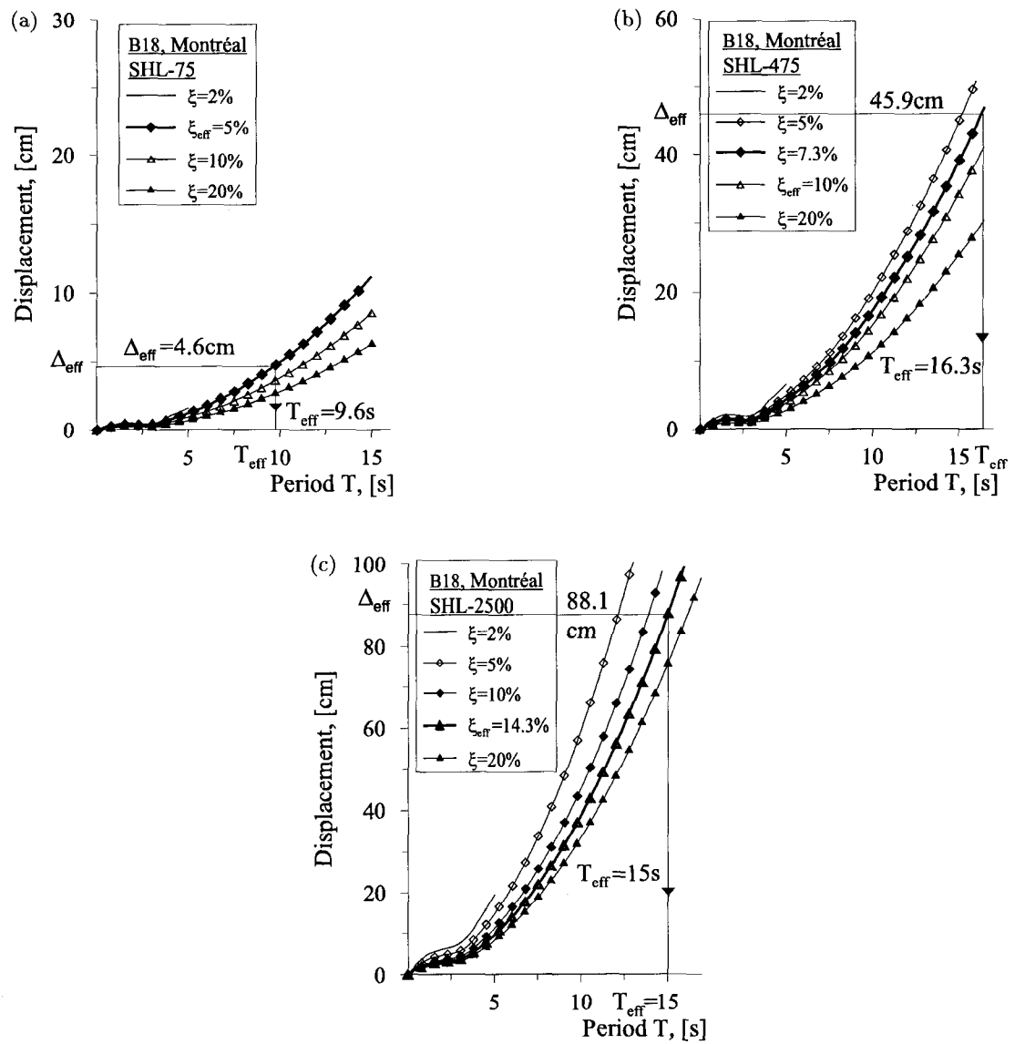
FIG. 5.15 Displacement Spectra for different damping values \xi for the B18 building in Montréal : (a) Seismic Hazard Level SHL-75 ; (b) Seismic Hazard Level SHL-475 and (c) Seismic Hazard Level SHL-2500.
