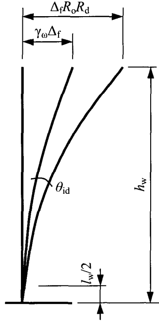
FIG. 2.3 Inelastic rotation
