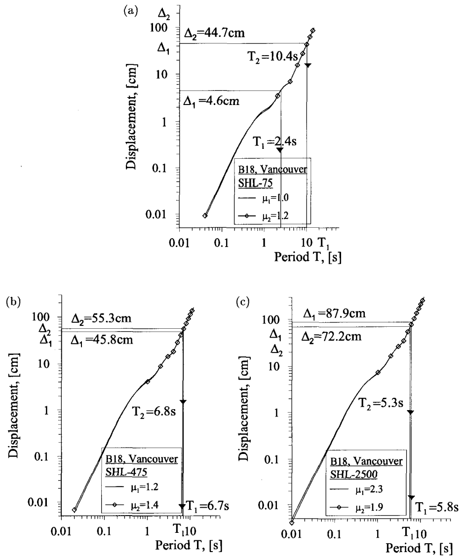
FIG. 5.23 Displacement Spectra for different ductility values \mu for the B18 building in Vancouver : (a) Seismic Hazard Level SHL-75 ; (b) Seismic Hazard Level SHL-475 and (c) Seismic Hazard Level SHL-2500.
