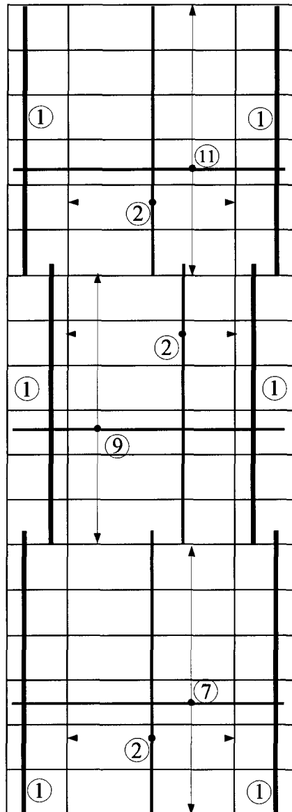
FIG. 4.10 Shear wall reinforcement in B18 building located in Montréal.
