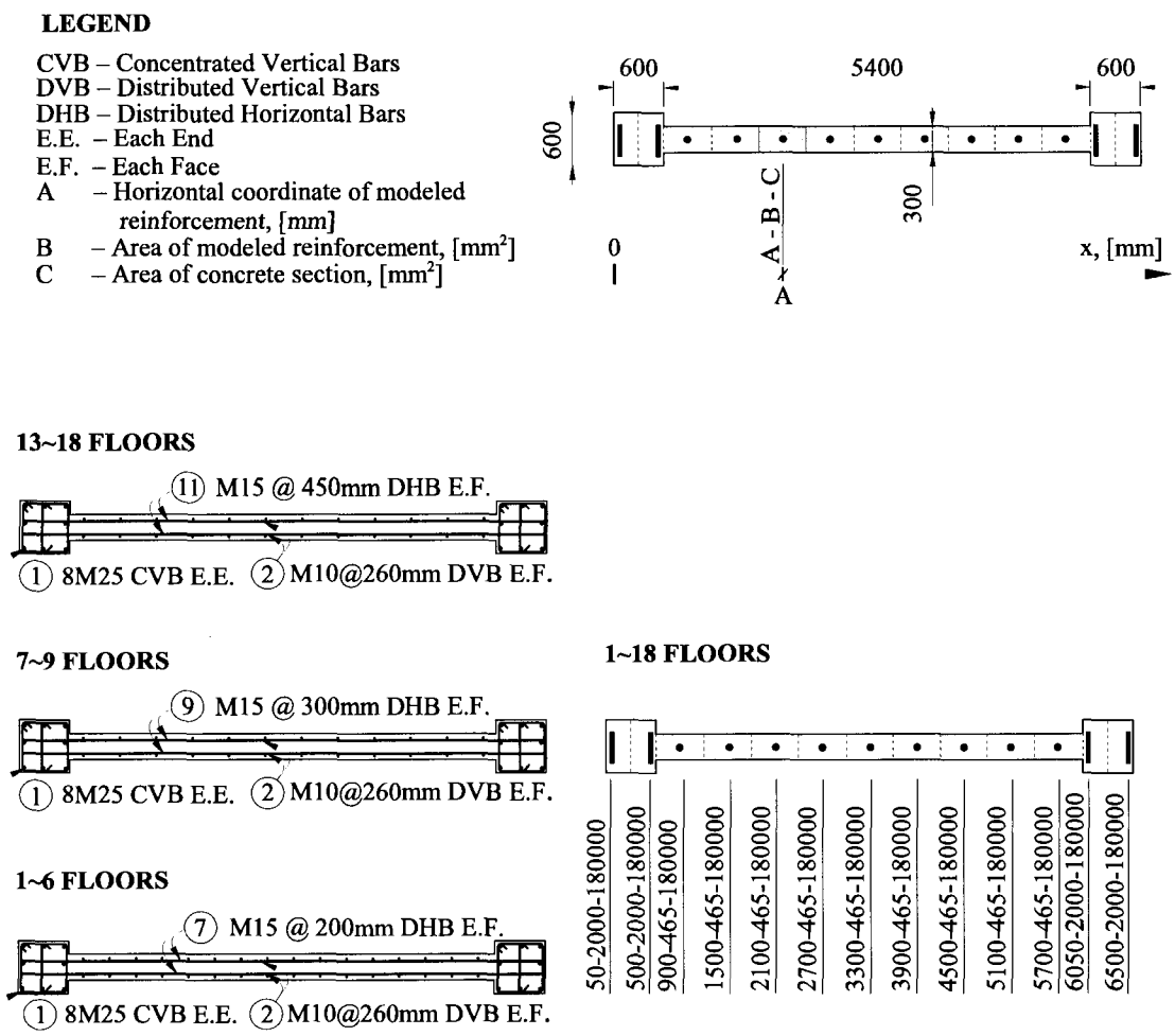
FIG. III.3 Modeling of shear wall sections for B18 located in Montréal
