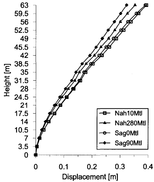
FIG. 6.39 Displacement results from non-linear dynamic analysis for earthquakes in Saguenay and Nahanni - 18 storey shear wall in Montréal
