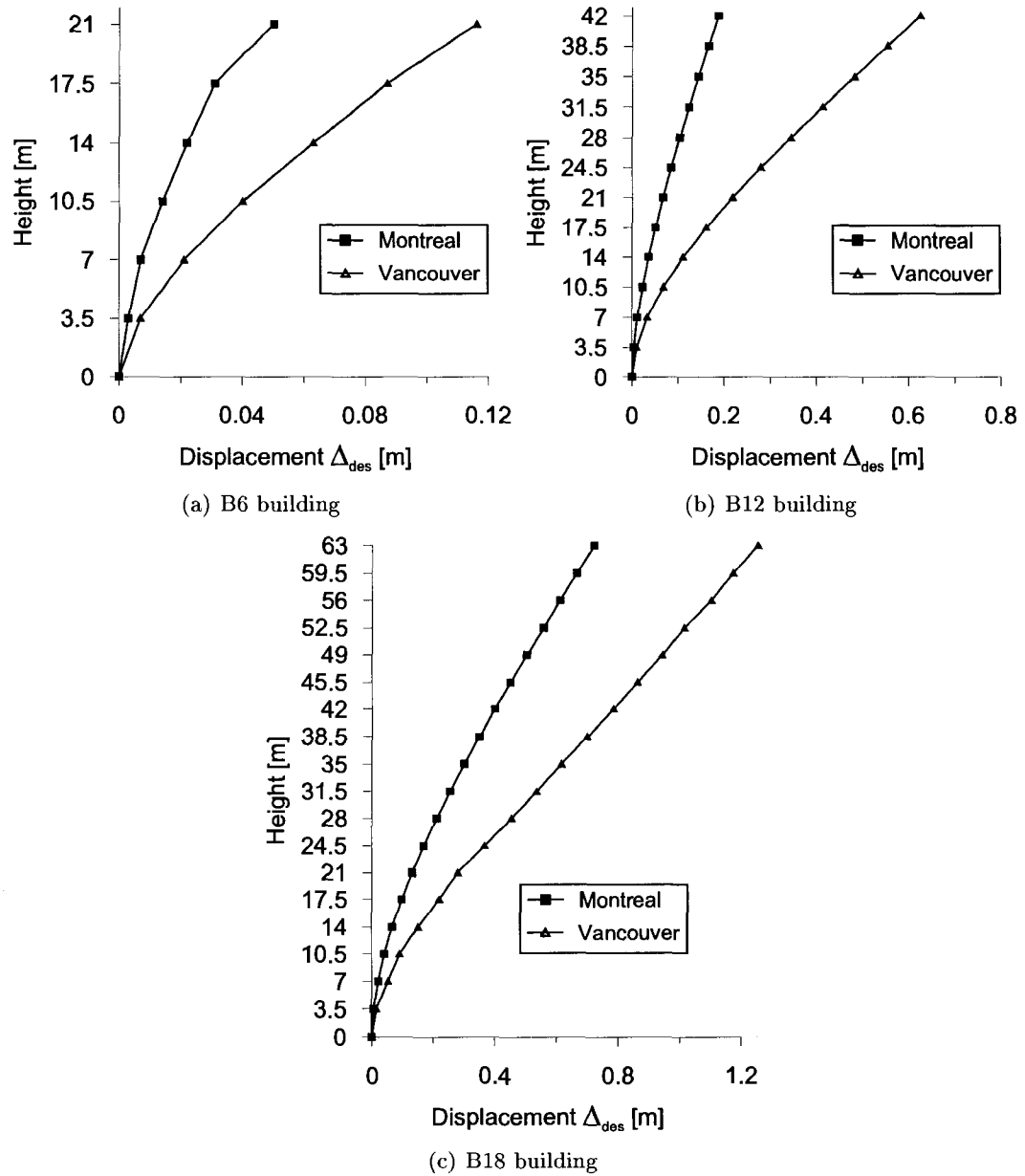
FIG. 4.7 Displacement results from spectral analysis for shear wall in B6, B12 and B18 in Montréal and Vancouver
