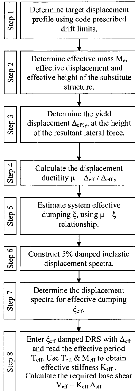
FIG. 3.19 Flowchart of DDBD method (Priestley and Kowalsky, 2000).
