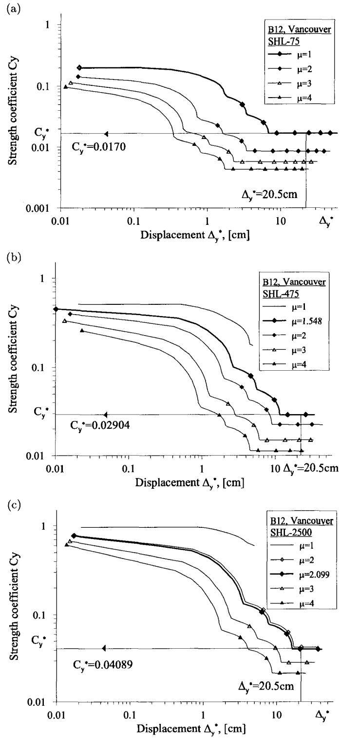
FIG. 5.6 Yield Point Spectra for the B12 building in Vancouver for different seismic hazard levels : (a) SHL-75; (b) SHL-475; and (c) SHL-2500.
