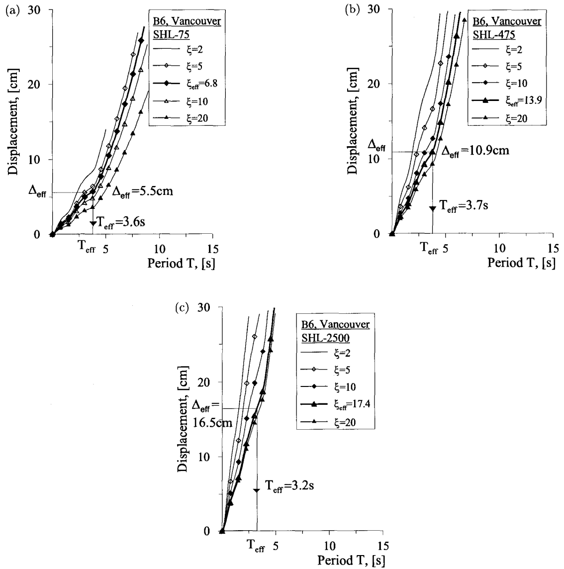
FIG. 5.12 Displacement Spectra for different damping values \xi for the B6 building in Vancouver : (a) Seismic Hazard Level SHL-75; (b) Seismic Hazard Level SHL-475 and (c) Seismic Hazard Level SHL-2500.
