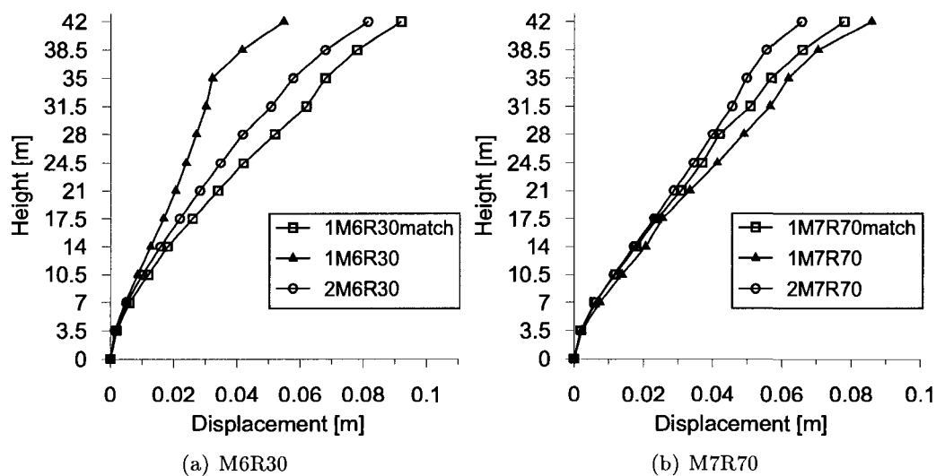
FIG. 6.36 Displacement results from non-linear dynamic analysis for 12 storey shear wall in Montréal
