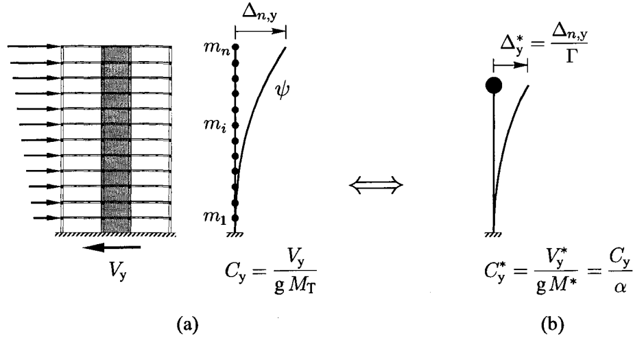
FIG. 3.16 Equivalent SDOF approximation : (a) MDOF system ; (b) Equivalent SDOF system.
