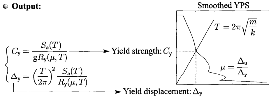
FIG. 3.2 Construction of Yield Point Spectra : (a) 'Exact' method ; (b) Approximate method.
