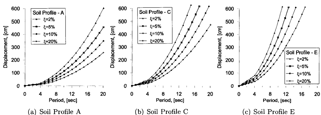
FIG. 3.21 Displacement response spectrums generated for different damping values for soil profiles A, C and E in Vancouver.
