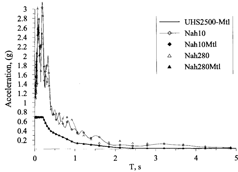
FIG. 6.8 Acceleration response spectra of original Nahanni ground motion and its close scaling to NBCC 2005 2% in 50 year UHS at Montréal.
