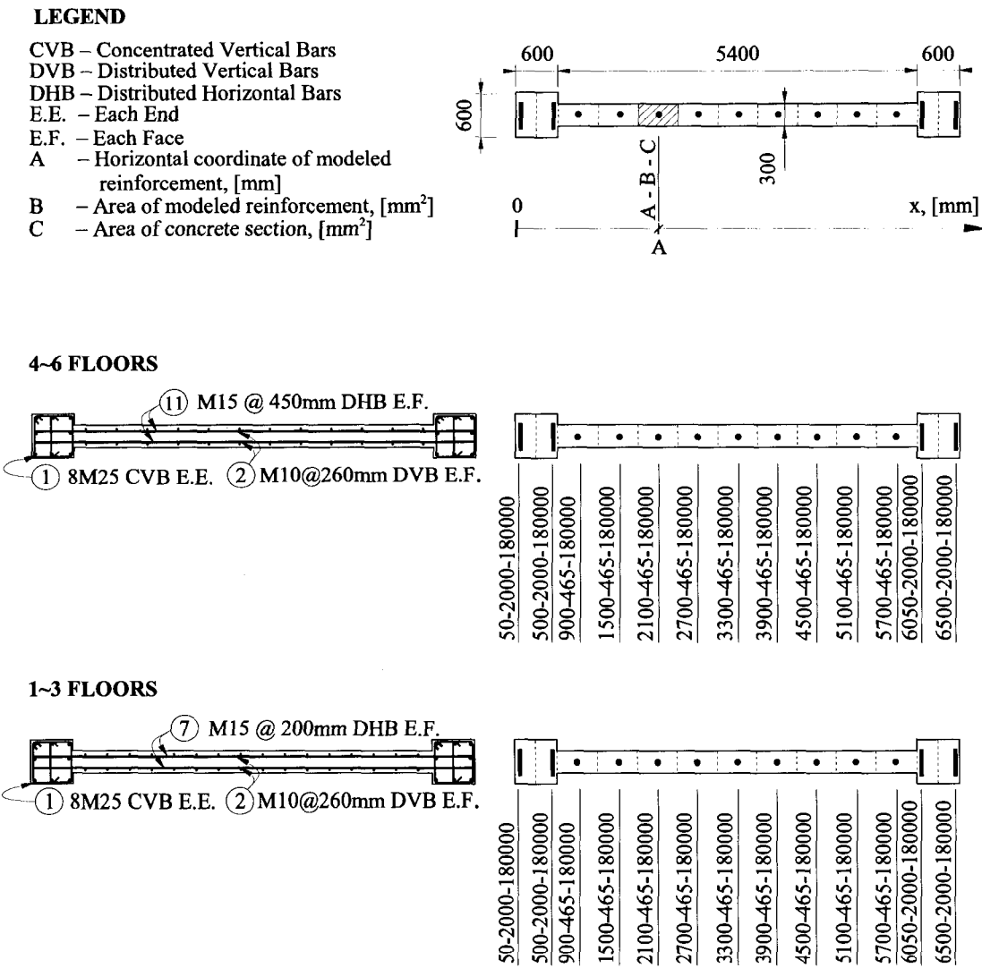
FIG. III.1 Modeling of shear wall sections for B6 located in Montréal
