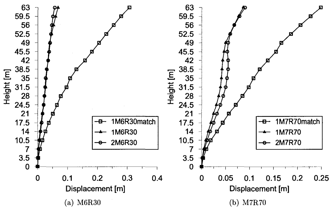
FIG. 6.38 Displacement results from non-linear dynamic analysis for 18 storey shear wall in Montréal
