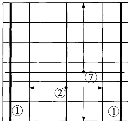
FIG. 4.11 Shear wall reinforcement in B6 building located in Vancouver.
