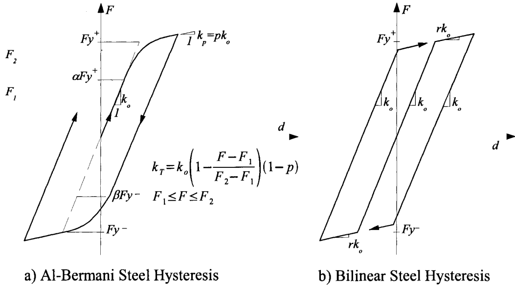
FIG. 6.13 Steel Hysteresis
