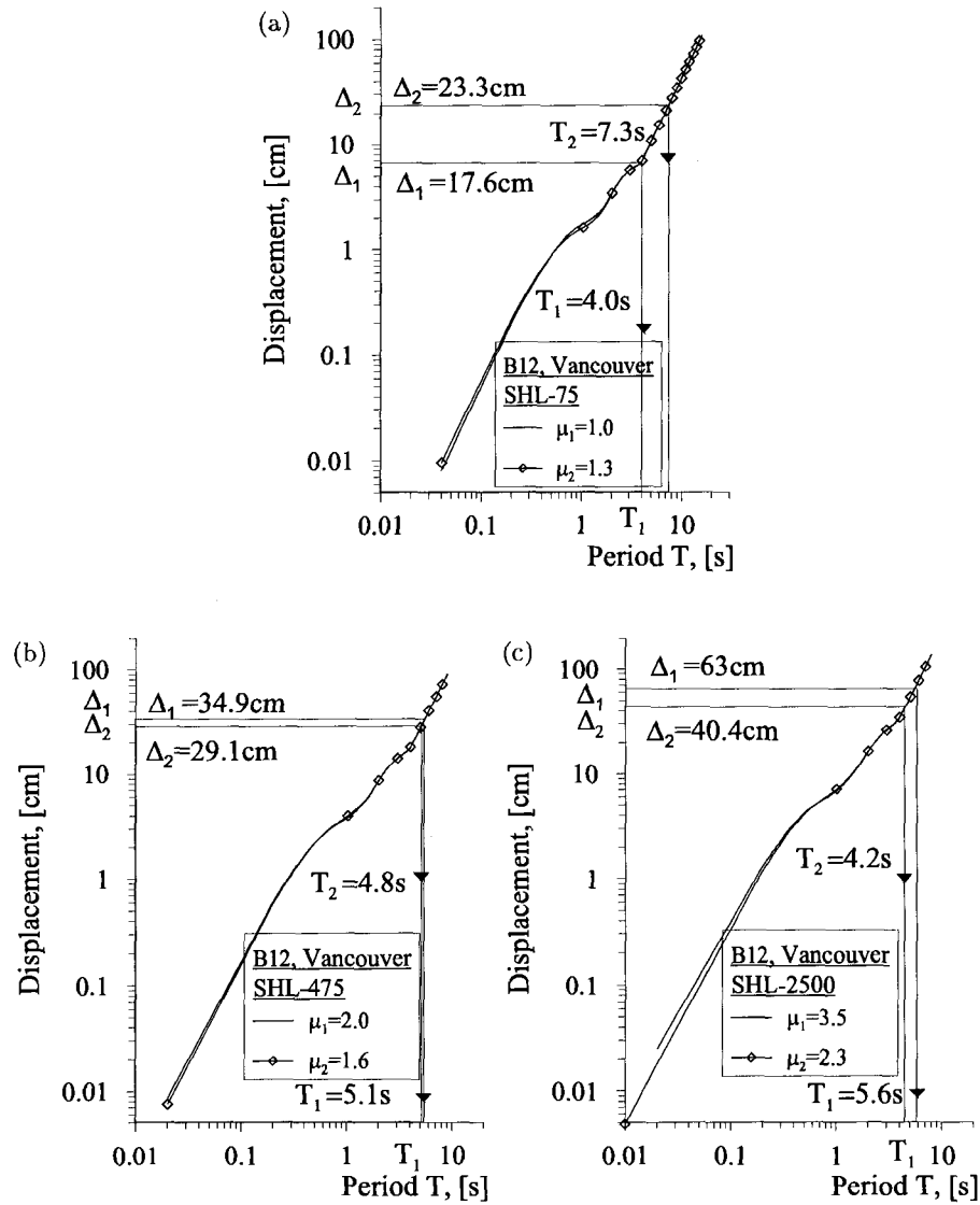
FIG. 5.21 Displacement Spectra for different ductility values \mu for the B12 building in Vancouver : (a) Seismic Hazard Level SHL-75; (b) Seismic Hazard Level SHL-475 and (c) Seismic Hazard Level SHL-2500.
