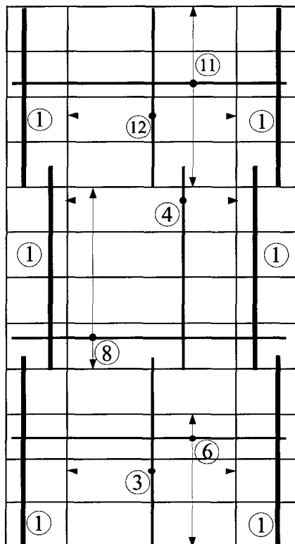
FIG. 4.12 Shear wall reinforcement in B12 building located in Vancouver.
