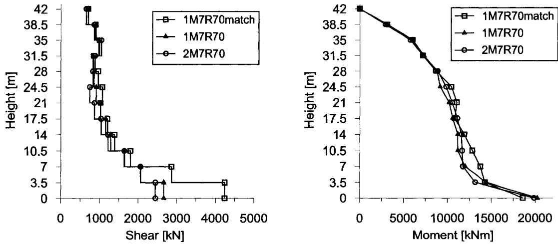
FIG. 6.20 Shear and moment results from non-linear dynamic analysis for earthquakes 1M7R70, 2M7R70 and 1M7R70match - 12 Storey
