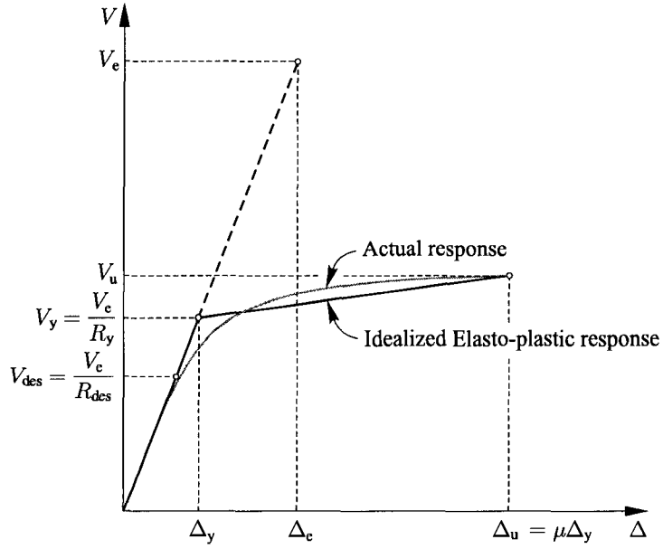
FIG. 3.1 Force-displacement relationships.
