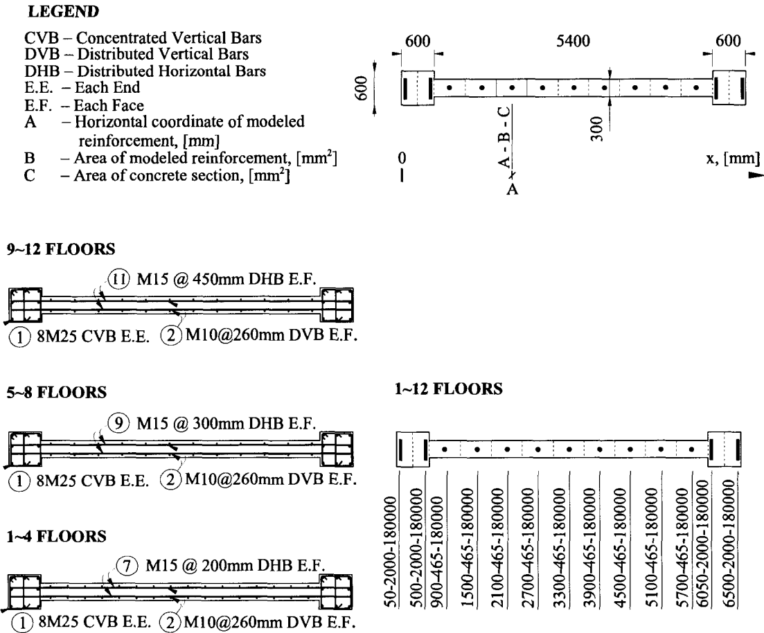
FIG. III.2 Modeling of shear wall sections for B12 located in Montréal
