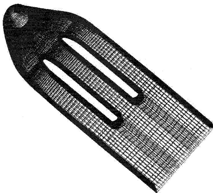
FIGURE 6.11 Resulting mesh - overall view
