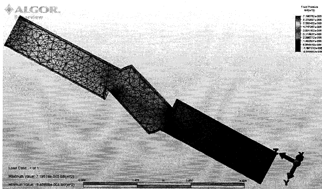
FIGURE 7.14 Pressure distribution
