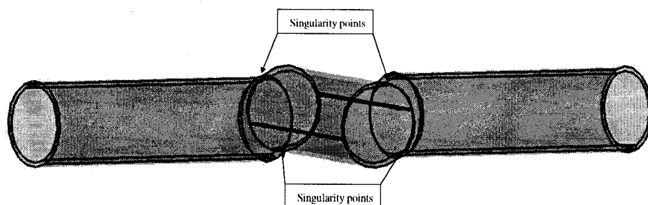
FIGURE 7.5 Boundary mesh interface
