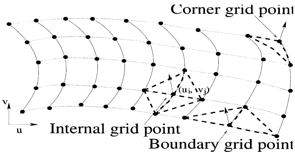
FIGURE 3.4 Direct offset method - quadrilateral discretization
