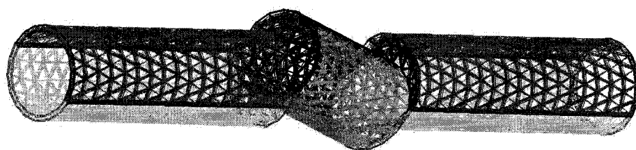
FIGURE 7.6 Boundary mesh
