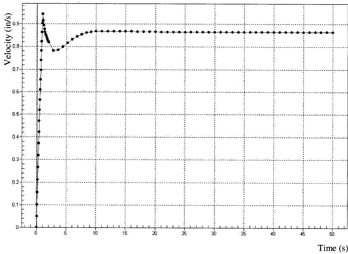
FIGURE 7.17 Velocity variation at node# 2794
