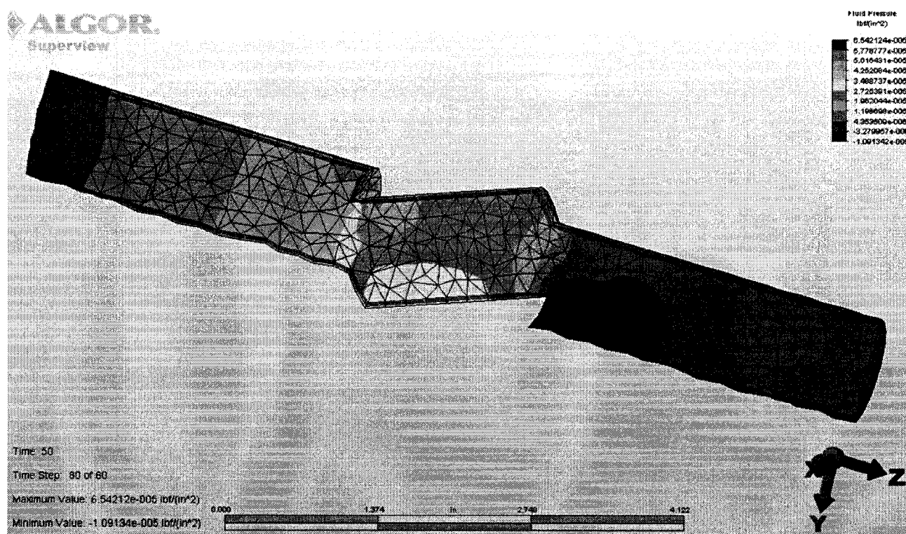
FIGURE 7.18 Pressure distribution
