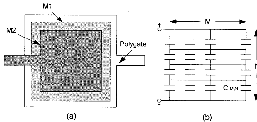
Figure 4.2. : Layout of the capacitor built with: (a) Polygate-Metal1-Metal2 and (b) using cascade M \times N array standard element.
