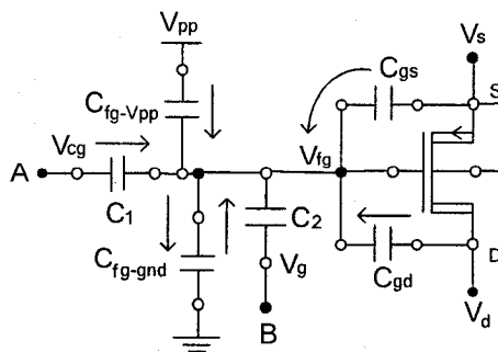
Figure 4.3. : Current model for FG DMOS transistor.
