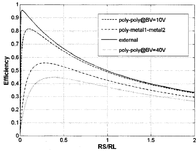
Figure 3.9. : Power efficiency versus R_S/R_L for various capacitors.
