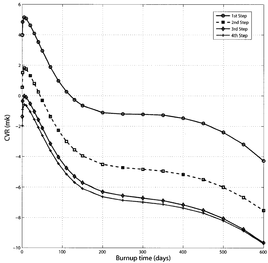
Figure III.15 CVR versus burnup time for Case 2
