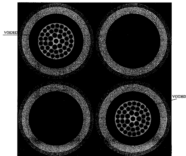
Figure III.2 2 \times 2 ACR assembly for checkerboard voiding study
