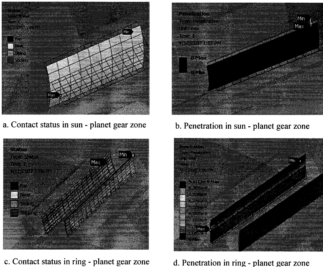
Fig. 3.10 Contact status and penetration with Pure Lagrange
