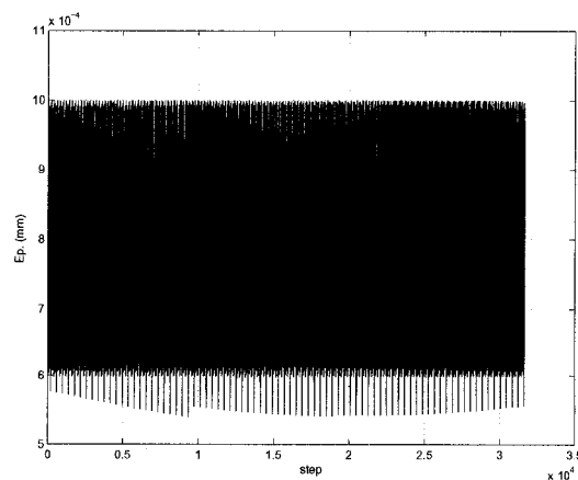
Figure 3.11: Positioning error from optimal post-processing
