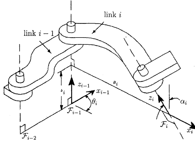
Figure 1.10: D-H parameters [26]
