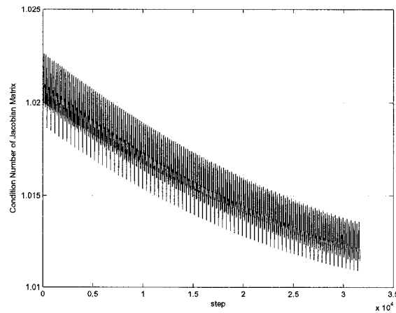
Figure 3.10: Condition number of the Jacobian matrix from optimal post-processing processing. Also, the positioning error of this process is shown in Fig. 3.11, according
