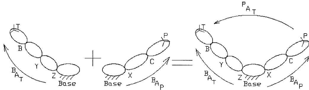
Figure 1.15: The kinematic chain of a five-axis machine-tool
