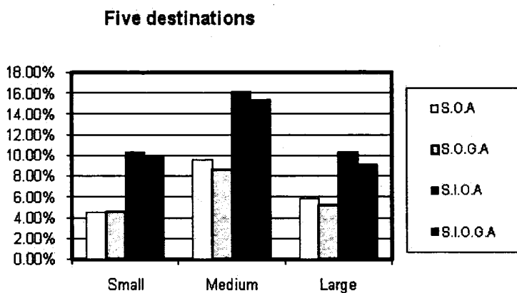
Figure 5-4: Compare algorithms performance for five destinations
