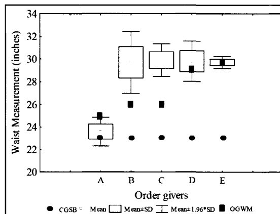
Figure 3.2 : Scatter plot
