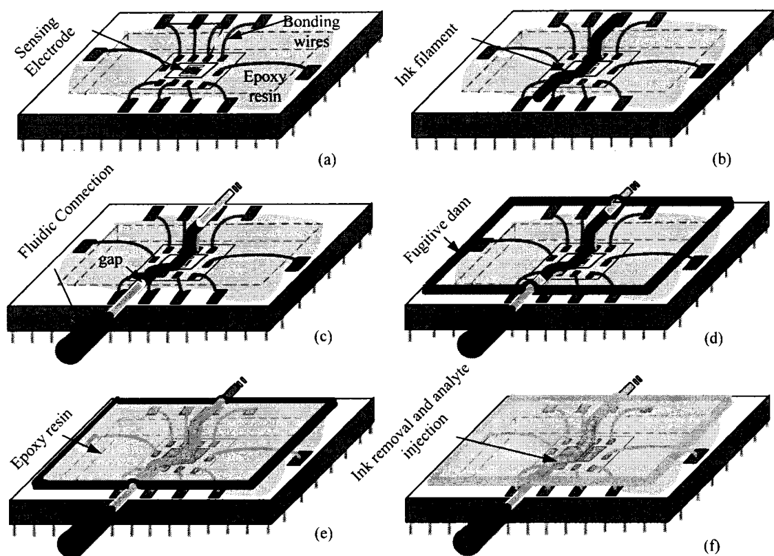
Figure. 5.1. Microfluidic packaging procedure: (a) wire bonding encapsulation, (b) ink deposition, (c) fluidic connection, (d) fugitive dam, (e) fugitive ink encapsulation and (f) ink removal and analyte injection.
