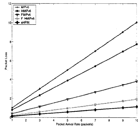
Figure 6.13 Packet loss vs. packet arrival rate.
