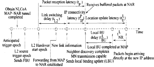
Figure 6.5 Handoff delay timeline of eHPIN for intra-BEN roaming.
