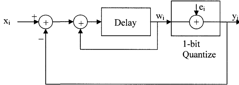
Figure 2-2: Block diagram of a first-order Delta Sigma modulator.
