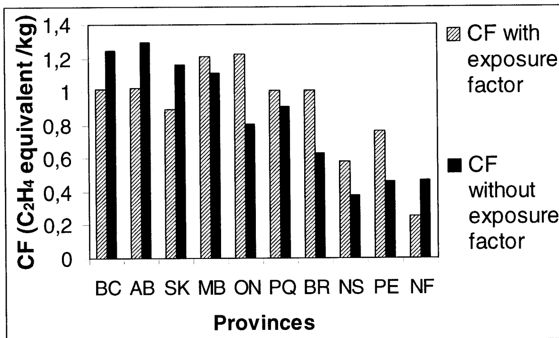
Figure 4.5 : Variation of the regional characterisation factors of Photochemical Ozone Formation expressed in kg ethylene (C 2 H 4 ) equivalent plotted against the variation of the fate factor, expressed as a Characterization factor without the exposure factor.
