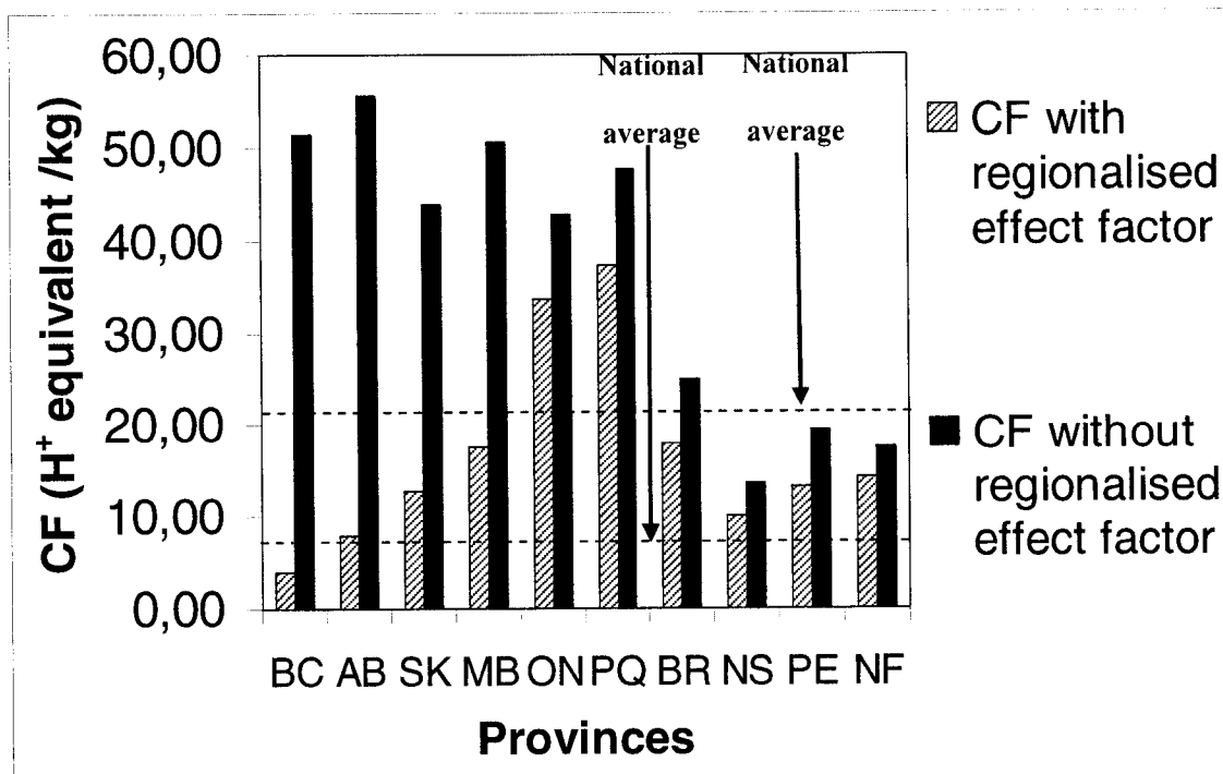
Figure 4.4 : Variation of the Fate factor (expressed as a Characterization factor without the effect factor) versus the characterization factor (including fate and effect) for sulphur dioxide ( \text{SO}_2 ) emissions for the acidification impact category.
