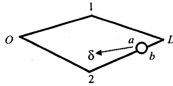
Figure 2.1: Exemple de chemins IIA.
