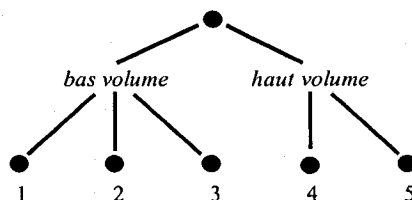
Figure 5.1: Structure imbriquée de nids.
