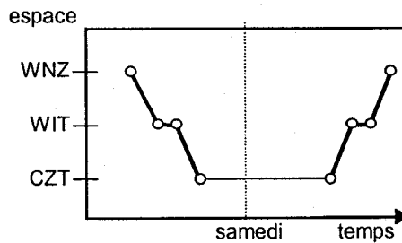
Figure 4.2: Voyage de plaisance type.
