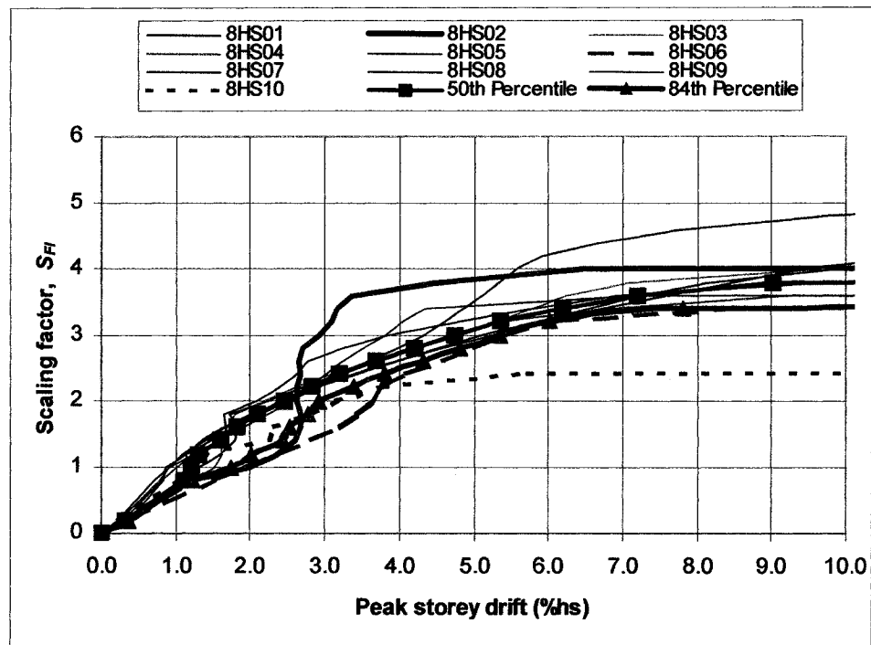
Fig. 5.5.1.1 Incremental dynamic analysis curve for 8-storey building
