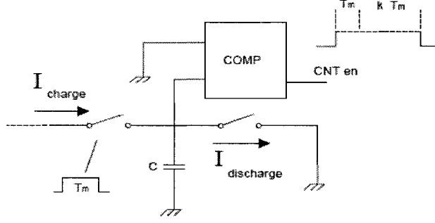
Figure 2.2: Time Interval Stretching Circuit Diagram
