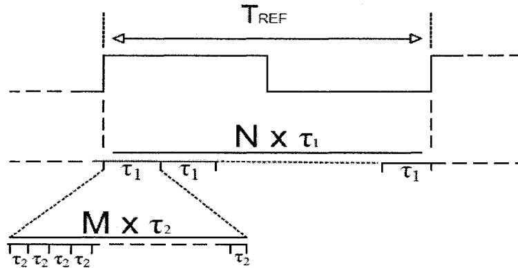
Figure 4.1: Two-level time interpolation
