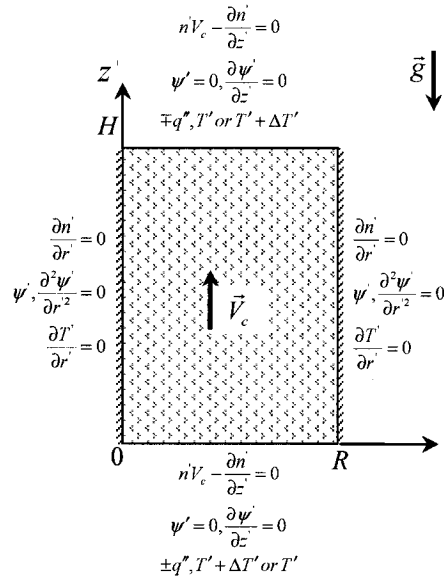
Figure 1.2 Coordinate system, computational domain and boundary conditions for thermo-bioconvection in vertical cylinders.
