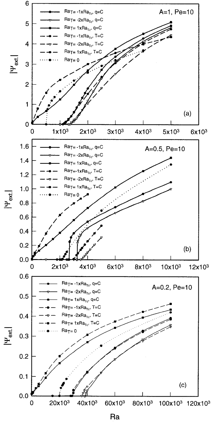
Figure 4.4 Bifurcation diagram for Ra_T = -1x Ra_{Tc} , -2x Ra_{Tc} , 1x Ra_{Tc} and Pe=10 . (a) A=1 , (b) A=0.5 , (c) A=0.2 .
