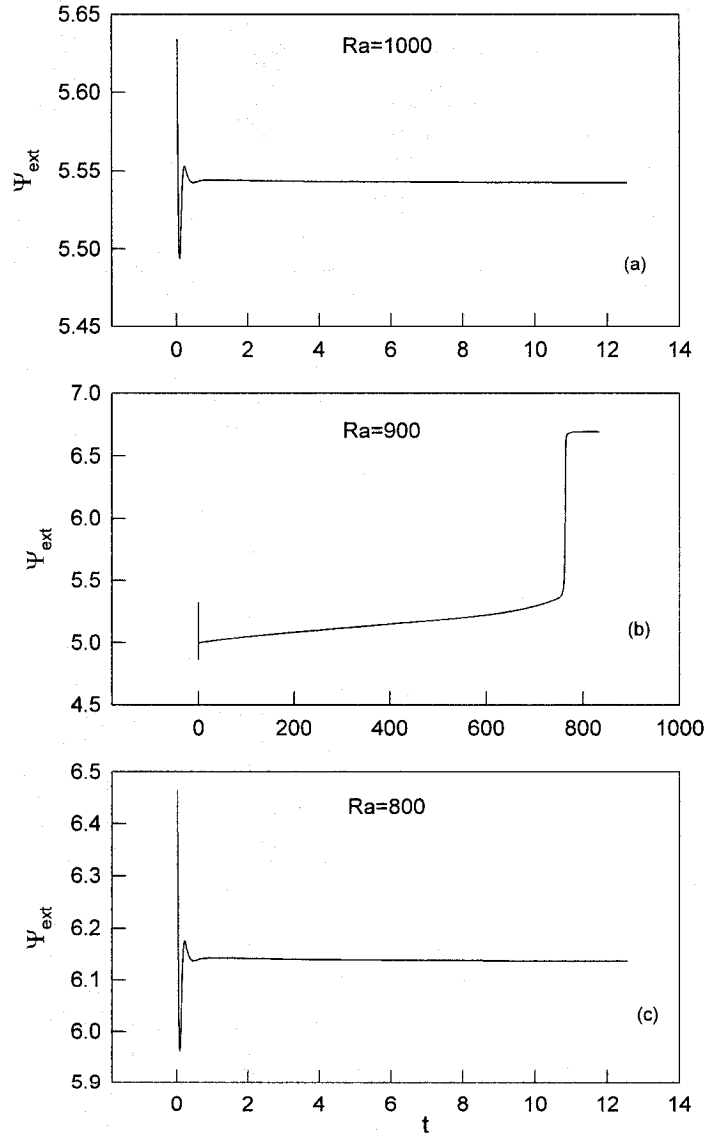
Figure 3.8 Time sequence diagrams corresponding to the case with A=5 , Pe=10 of Figure 3.5(c) at a) Ra=1000 , b) Ra=900 , c) Ra=800 .
