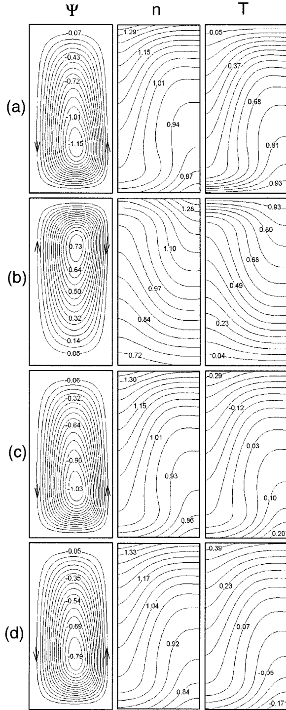
Figure 4.7 Streamlines, iso-concentration and isotherm for A=0.5 , Pe=1 and Ra=5Ra_c .
