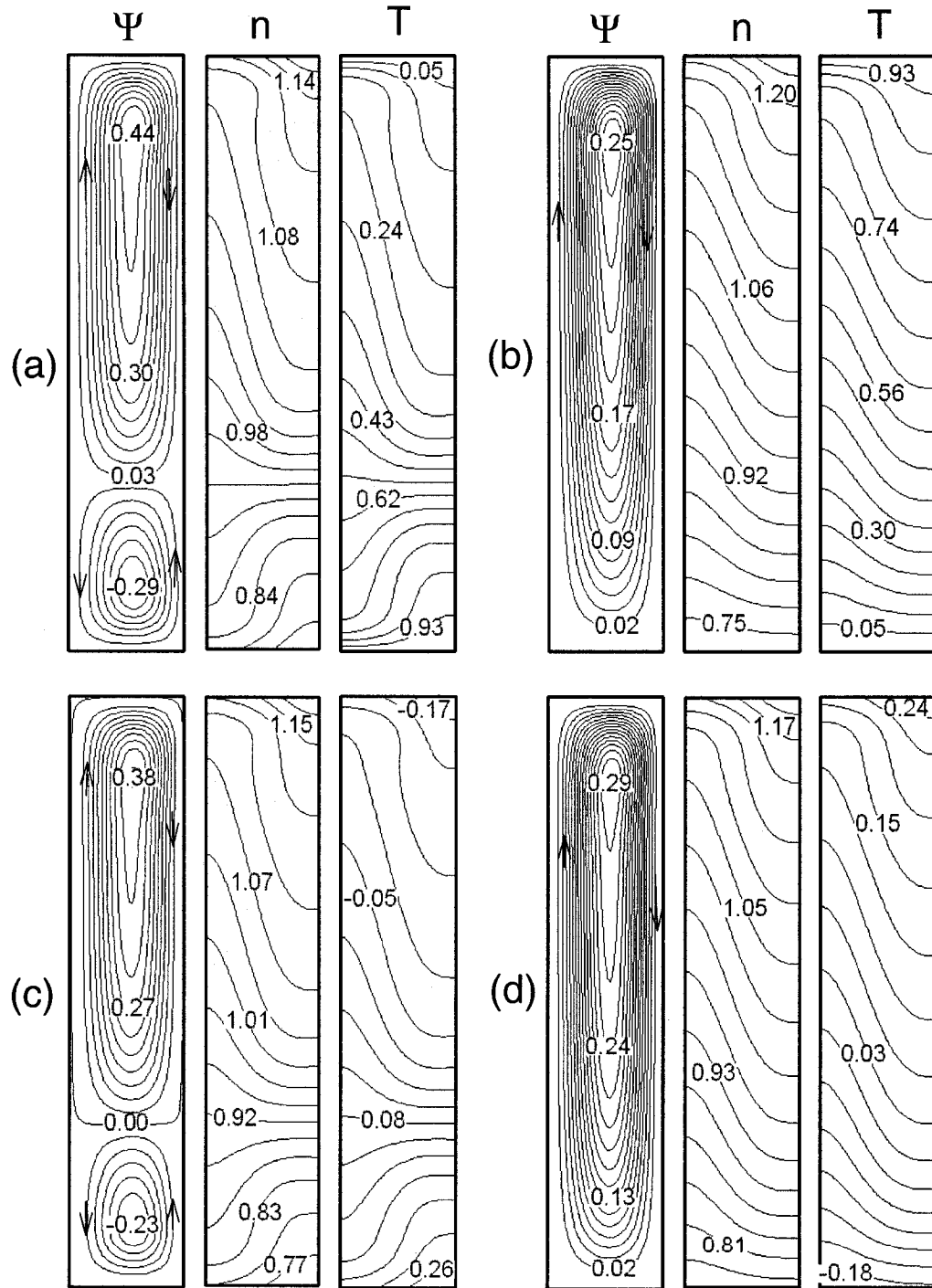
Figure 4.8 Streamlines, iso-concentration and isotherm for A=0.2 , Pe=1 and Ra=5 \times Ra_c .
