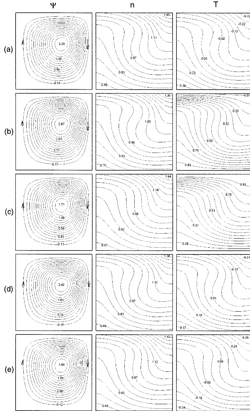
Figure 4.6 Streamlines, iso-concentration and isotherm for A=1 , Pe=1 and Ra=5 \times Ra_c . (a) Ra_T=0 (b) T=\text{constant} , Ra_T=1 \times Ra_{Tc} (c) T=\text{constant} , Ra_T=-1 \times Ra_{Tc} (d) q=\text{constant} , Ra_T=1 \times Ra_{Tc} , (e) q=\text{constant} , Ra_T=-1 \times Ra_{Tc} .
