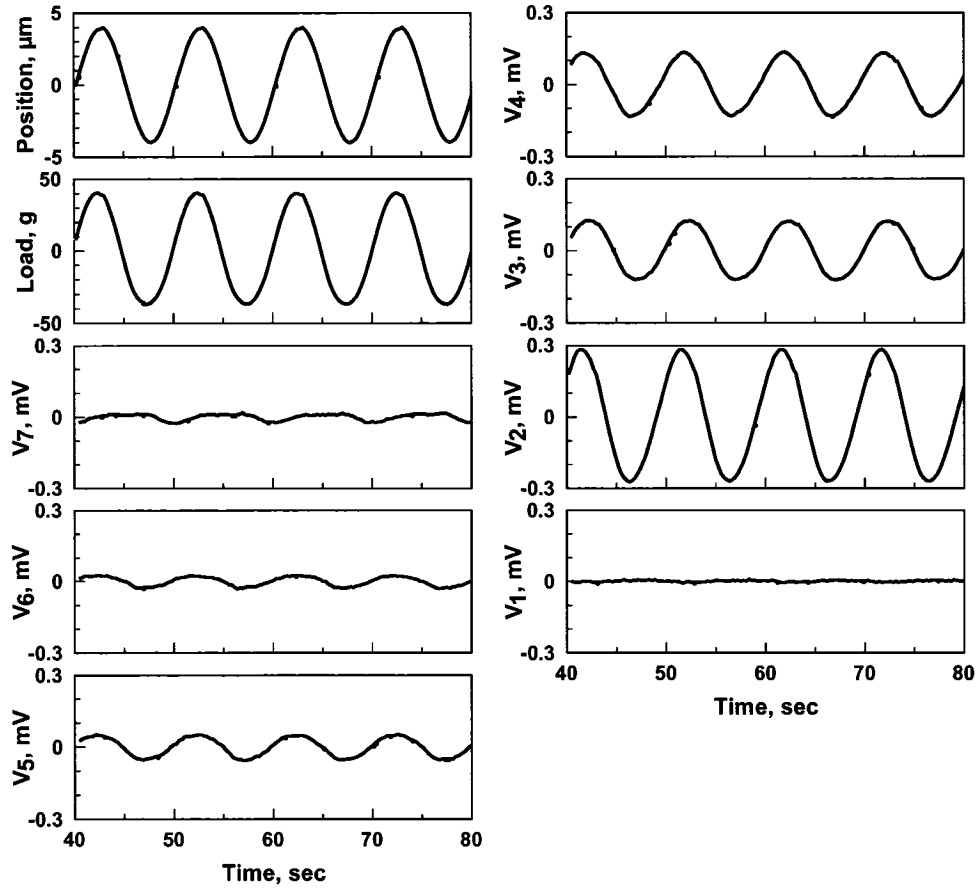
Figure 1-4 : Position, Load and Streaming Potential Raw Data . A sinusoidal displacement of 4\mu\text{m} amplitude and 0.1 Hz frequency was applied in unconfined compression geometry generating a load of approximately 40g amplitude. The differential potential between adjacent electrodes is shown starting with the electrode pair ( V_7 ) on the opposite side of the disk center and ending with the electrode pair in the bath ( V_1 ) (refer to Figure 1-2). The amplitude of the differential potential increases towards the periphery of the disk, in agreement with biphasic model predictions that the relative velocity of fluid with respect to solid increases with radius across the disk during unconfined compression.
