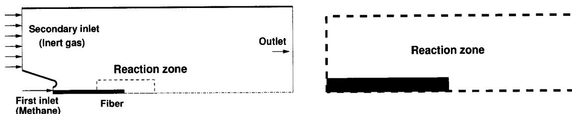
Figure 7.1 Domain decomposition
