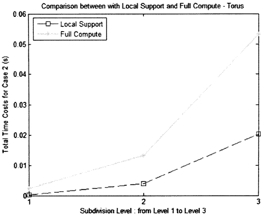
Figure 4-8: The comparison of editing one selected vertex on the Loop subdivision torus surfaces between with local support and with full compute.
