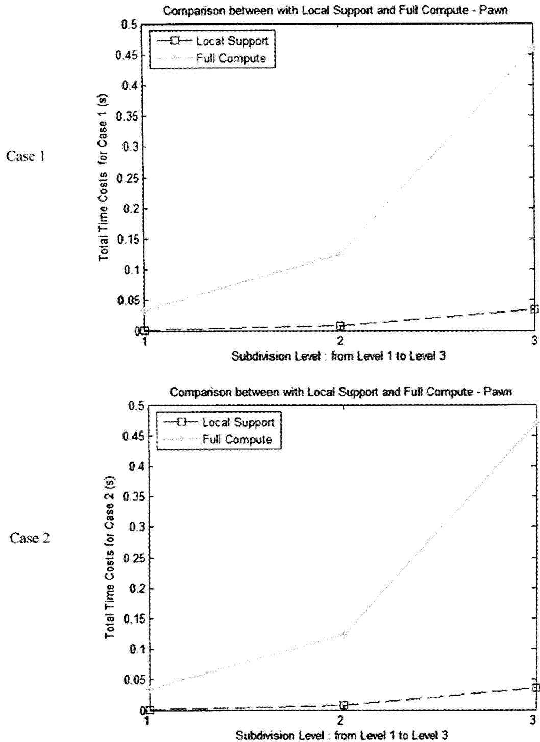
Figure 4-9: The comparison of editing one selected vertex on the Loop subdivision pawn surfaces between with local support and with full compute.
