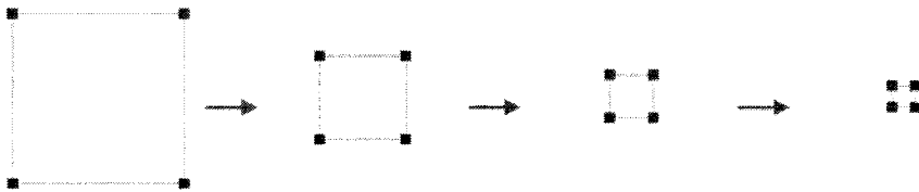
Figure 2-8: Averaging (the old retained vertices are shrunk along their diagonals).
