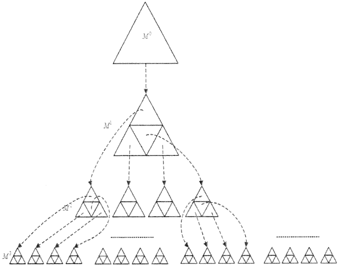
Figure 3-23: Triangle QuadTree as the global data structure for meshes from coarse level to finer levels, where M^i represents the triangle surface at i^{\text{th}} level.
