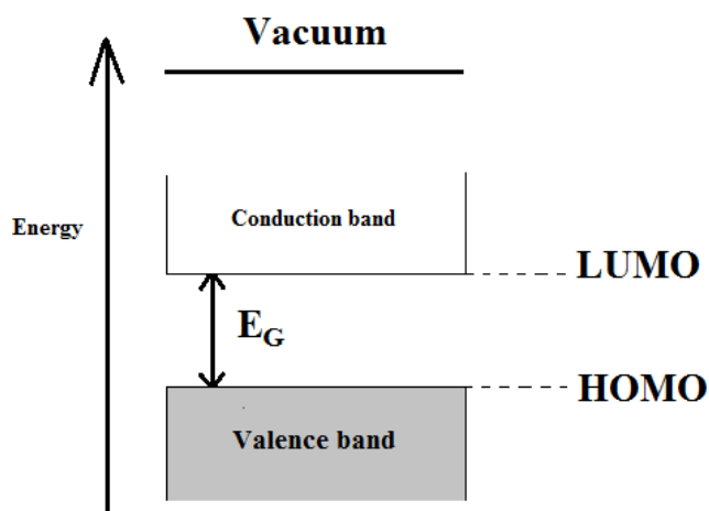
Figure 1.3: Scheme of the energy band diagram for organic semiconductors.
