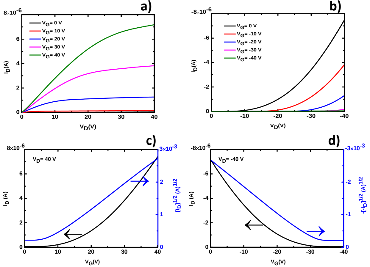
Figure 3.16: Output characteristics of SWCNT P3HT/PCBM (1:1) TFTs for n-type a) and p-type b) behaviors. Transfer characteristics of SWCNT P3HT/PCBM (1:1) TFTs for n-type c) and p-type d) behaviors. V_D ( V_G ) changes by \pm 100 mV ( W/L = 1540 \mu\text{m} / 10 \mu\text{m} , 100 nm thick \text{SiO}_2 ).
