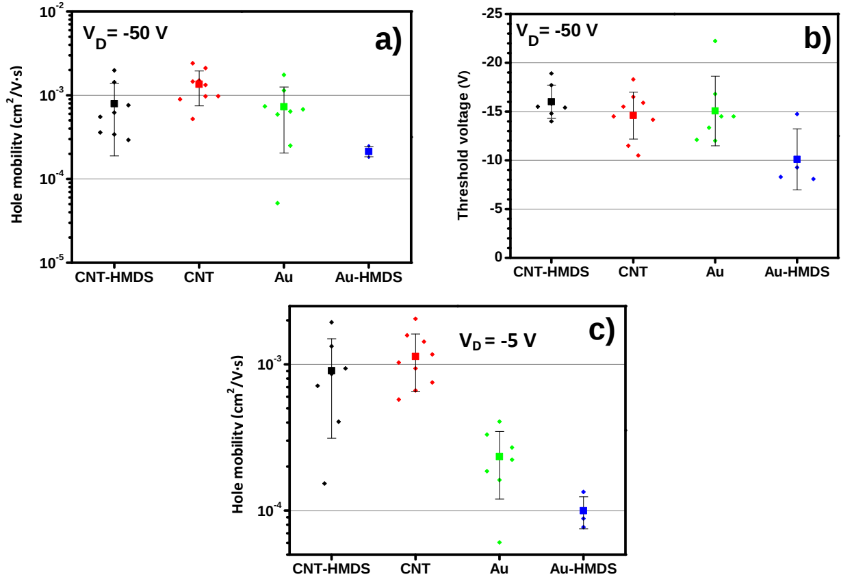
Figure_A 2.5: Hole mobility a), threshold voltage b) extracted in the saturation regime ( V_D = -50 V) and hole mobility (c) extracted in the linear regime ( V_D = -5 V) of SWCNT P3HT TFTs, Au P3HT TFTs, SWCNT HMDS P3HT TFTs, Au HMDS P3HT TFTs. Error bars denote the standard deviation. L/W = 5/1555 \mu\text{m}/\mu\text{m} , L/W = 10/1540 \mu\text{m}/\mu\text{m} , L/W = 20/1510 \mu\text{m}/\mu\text{m} , L/W = 50/1413 \mu\text{m}/\mu\text{m} .
