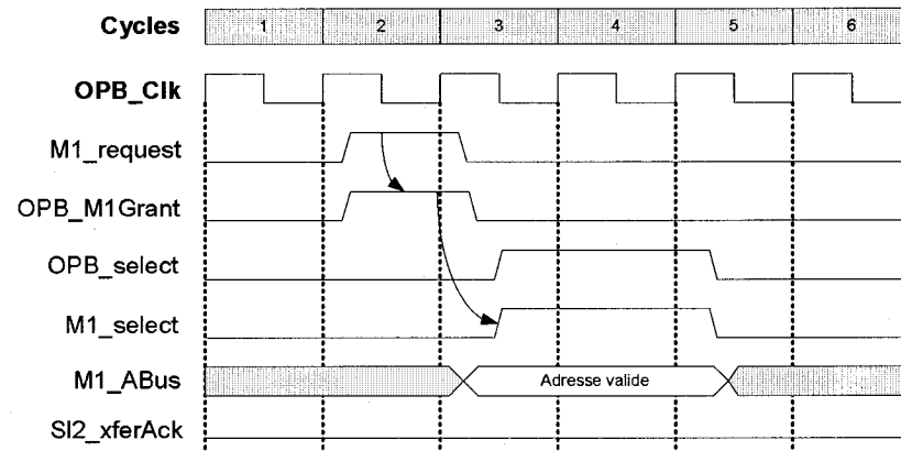
Figure 2.4 : Annulation de requête [IBM02]
