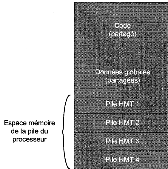
Figure 3.4: Organisation de la mémoire
