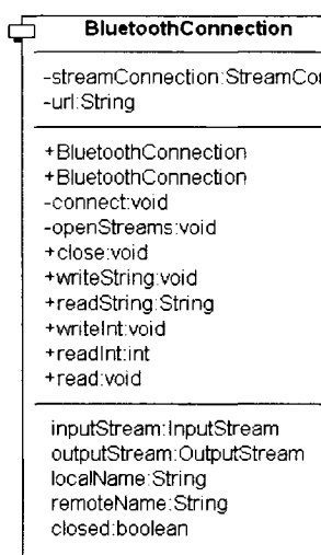
Figure 4.5 Classe BluetoothConnection
