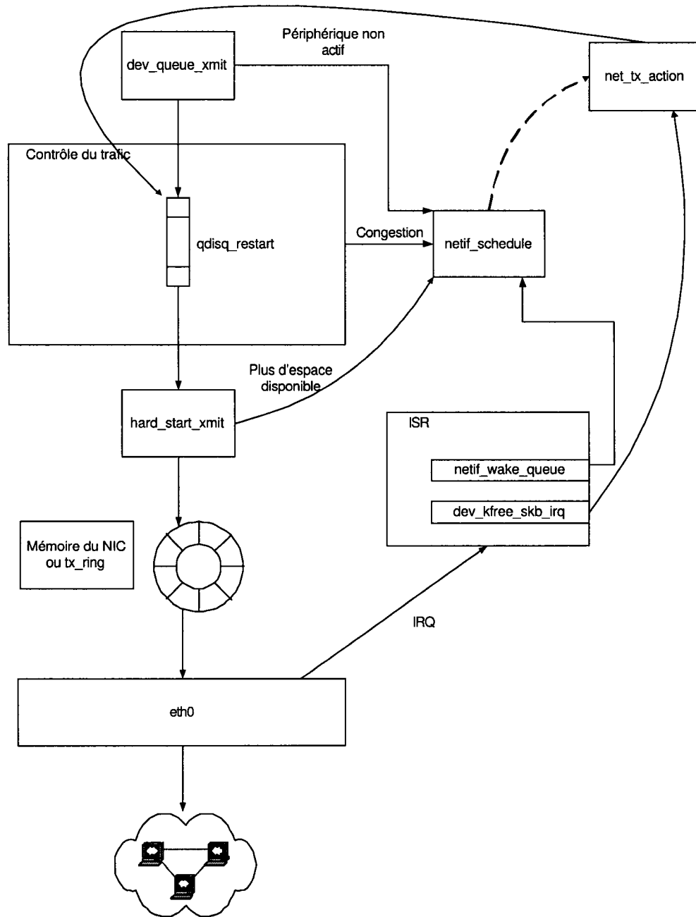
Figure 2.6 Transmission de paquets
