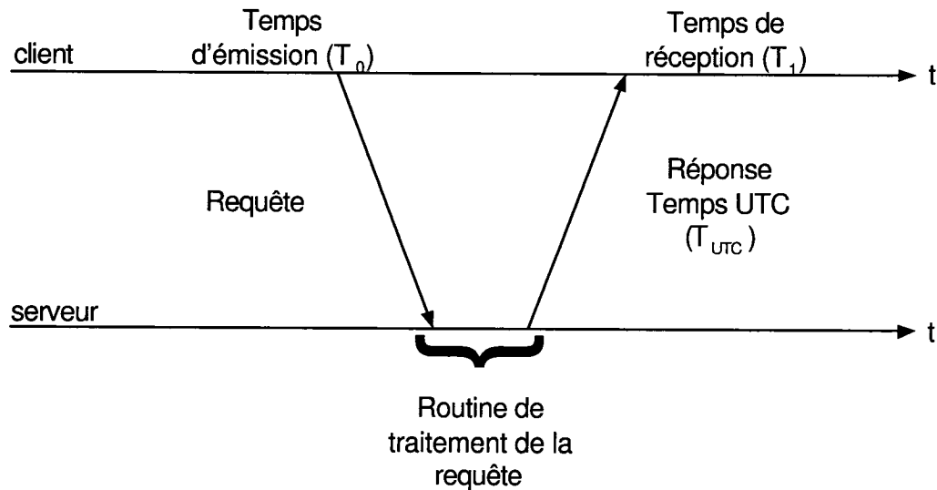
Figure 1.1 Algorithme de Cristian
