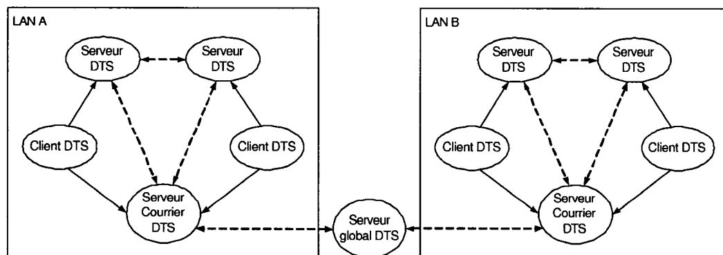
Figure 1.3 Architecture du service DTS
