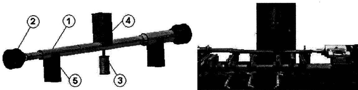
Figure 1.5 Press straightening from Eitel Presses [9]
