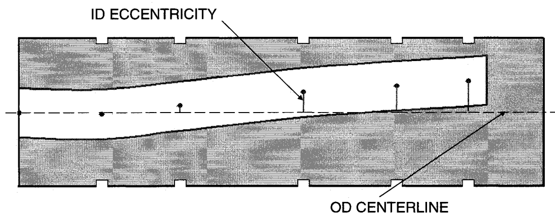
Figure 3.3 ID eccentricities measured along the length
