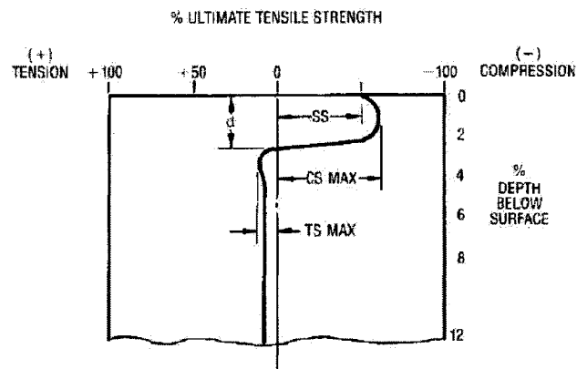
Figure 1.12 Typical residual compressive stress profile [29]
