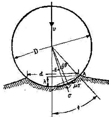
Figure 1.11 Plastic dimple created by shot peening [25]
