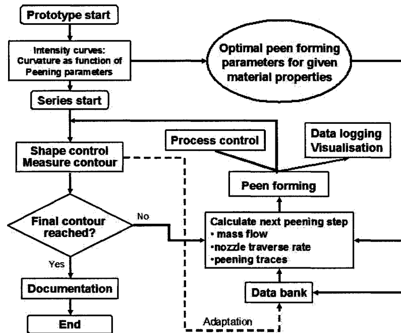
Figure 1.13 Flow chart for controlled peen forming [26]
