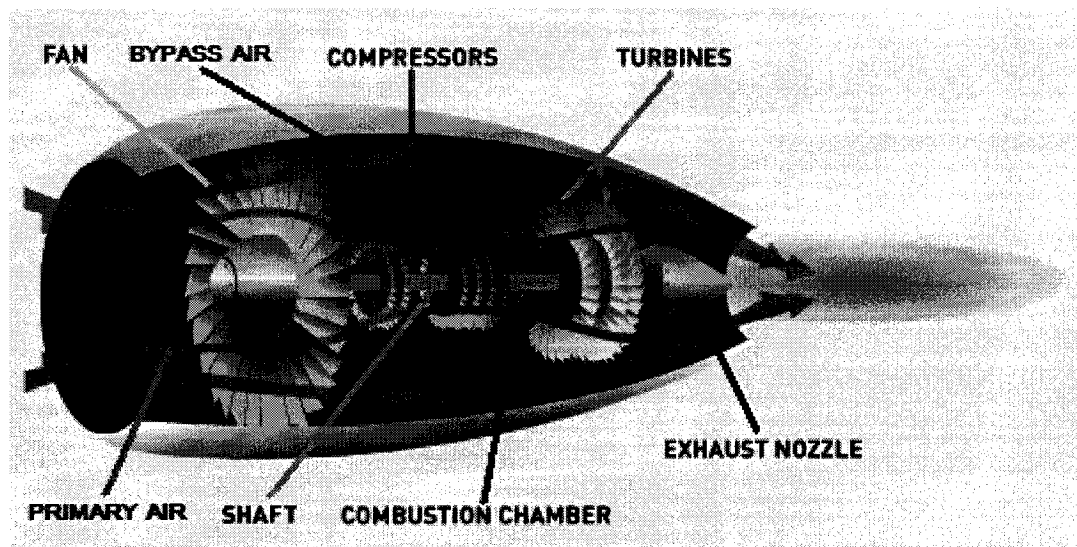
Figure 1.1 Turbofan [2]
