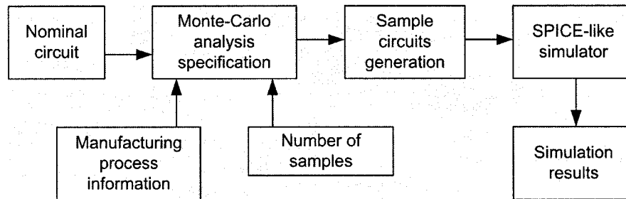
Figure 5.3 : Block diagram of MC analysis tools
