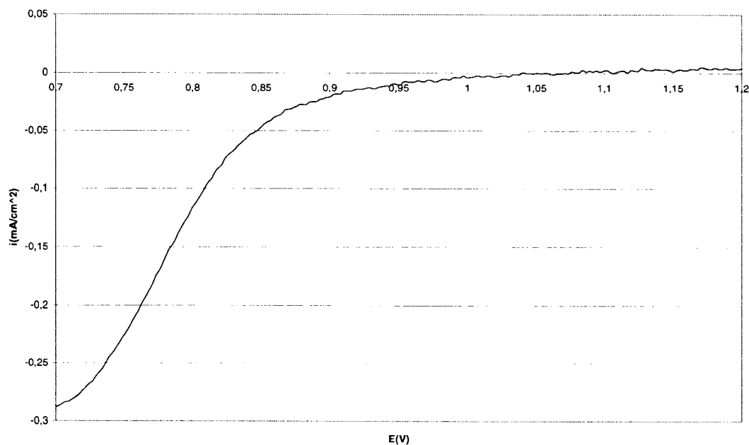
Figure 3.2: CV in 0,5M \text{H}_2\text{SO}_4 on bulk Pt (ambient temperature, oxygen saturated / 60 minutes bubbling, sweep rate of 50mV/s)
