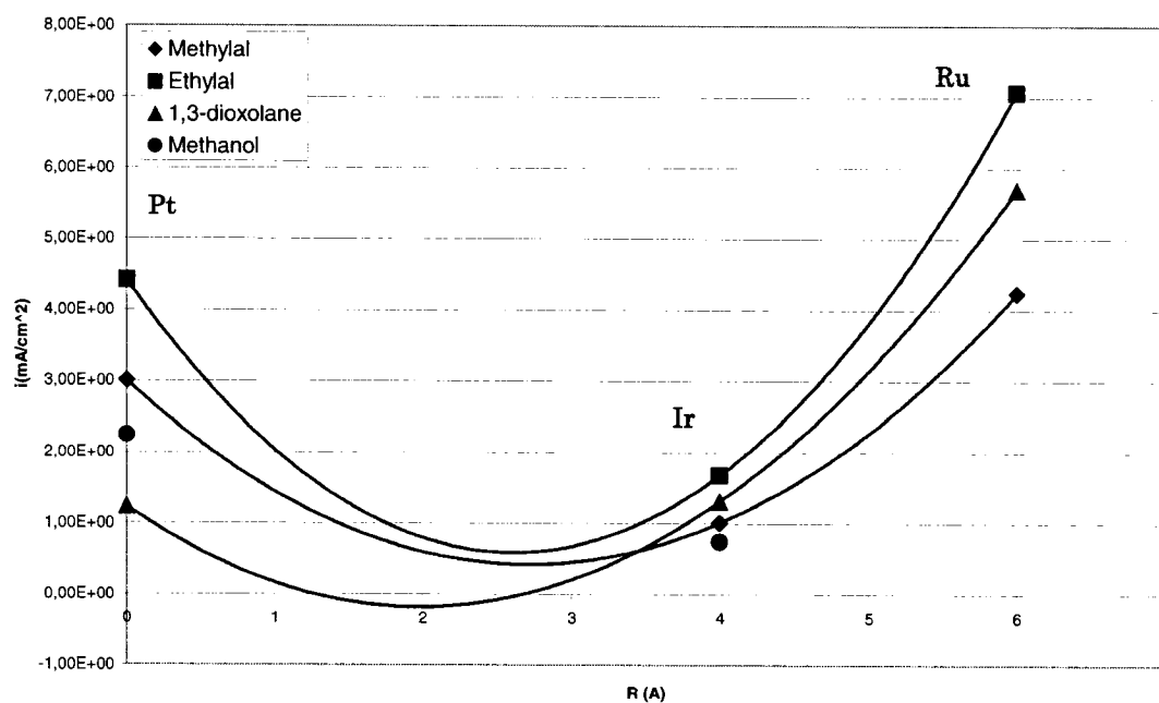
Figure 3.23: Current intensity of the oxidation peak against \Delta R with methylal, ethylal, 1,3-dioxolane, and methanol in 0,5M \text{H}_2\text{SO}_4 (ambient temperature, oxygen saturated / 60 minutes bubbling, sweep rate of 50mV/s)
