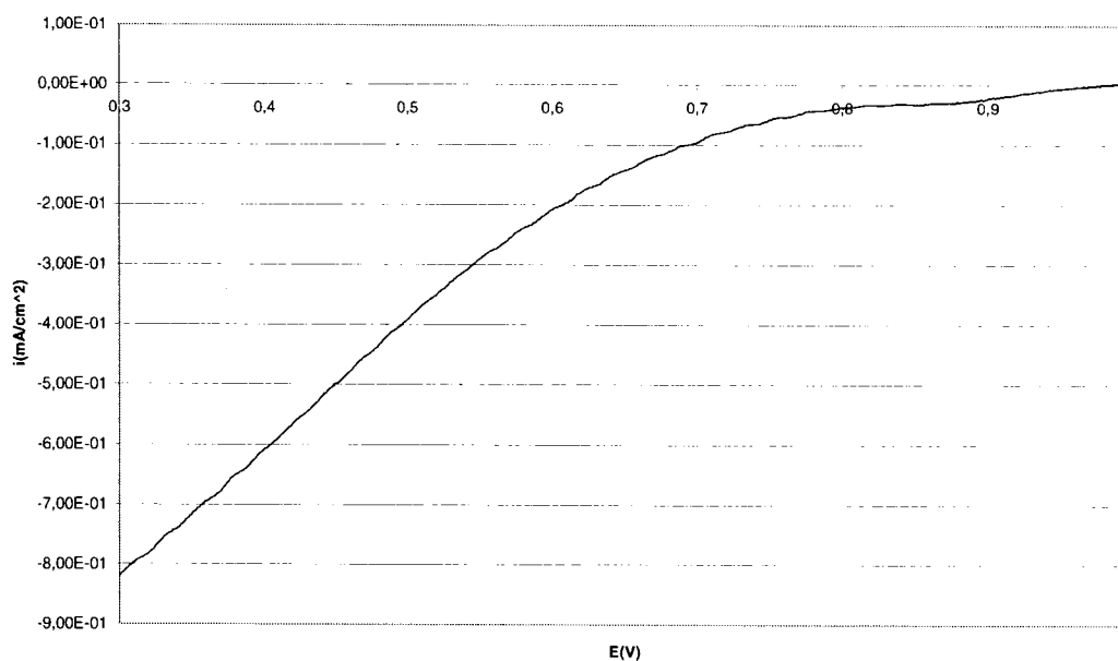
Figure 3.19: CV in 0,5M \text{H}_2\text{SO}_4 on PtIr/C (ambient temperature, oxygen saturated / 60 minutes bubbling, sweep rate of 5mV/s)
