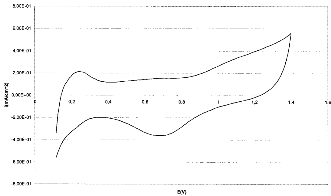
Figure 3.7: CV in 0,5M H 2 SO 4 on Pt/C (ambient temperature, nitrogen saturated / 60 minutes bubbling, sweep rate of 50mV/s)
