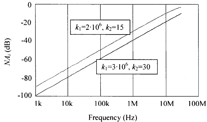
Figure 2.17 Noise attenuation of the current injected active filter
