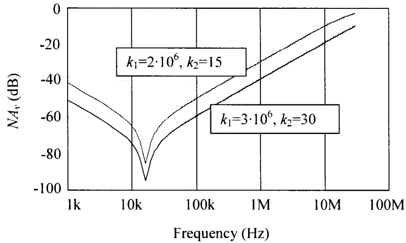
Figure 2.16 Noise attenuation of the voltage injected active filter
