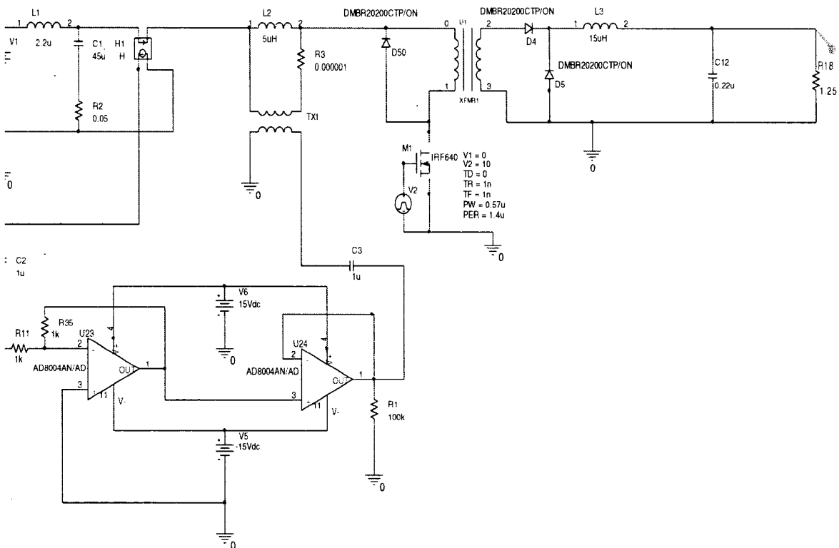
Figure C.1 DC/DC converter Simulation diagram including the active EMI filter
