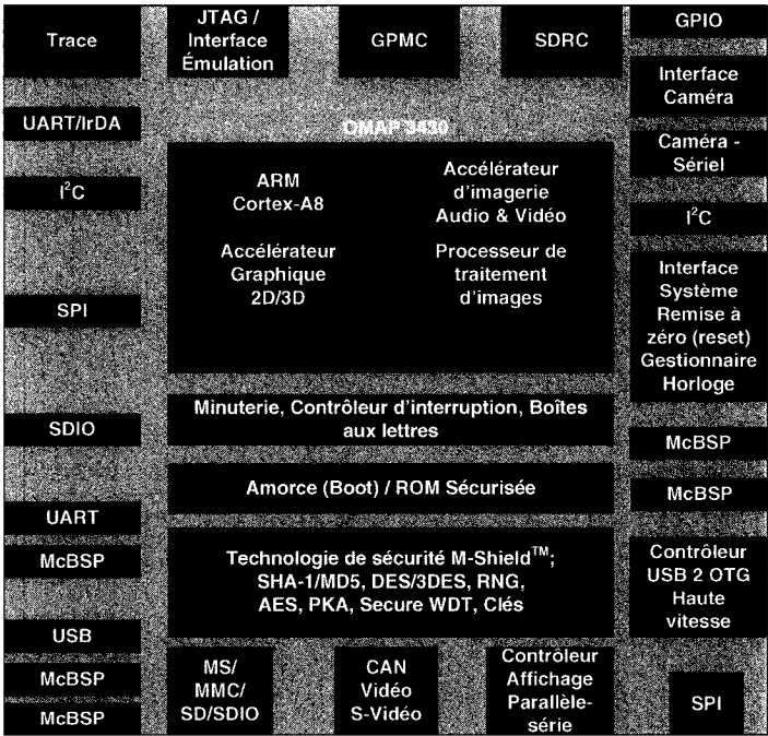
Figure 2.9 Architecture de la plateforme OMAP (Texas Instruments)
