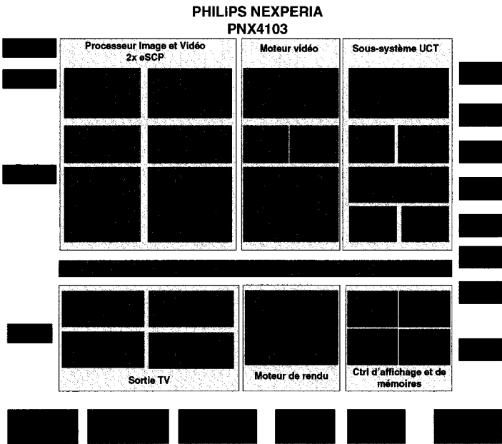
Figure 2.10 Architecture de la plateforme Nexperia (Philips)
