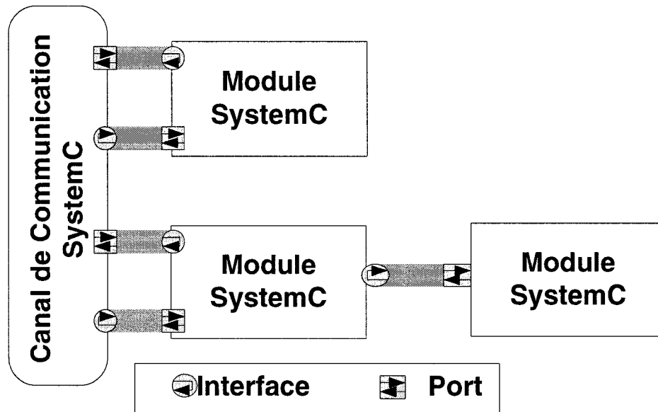
Figure II.1 Structure architecturale des composants SystemC
