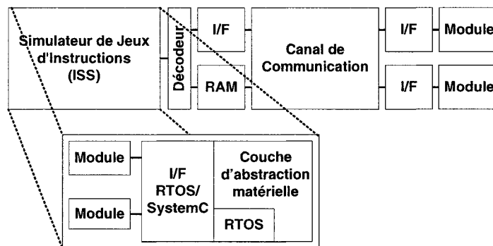
Figure 2.7 Architecture de la plateforme SPACE
