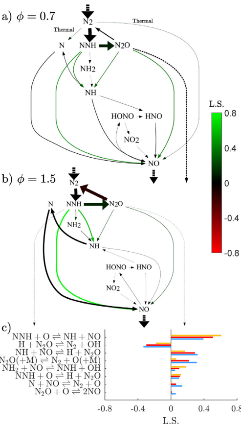
Fig. 5. RPA shown for (a) \phi = 0.7 and (b) \phi = 1.5 . Arrows are scaled by the flux of N-atoms where only fluxes > 1\% are shown for clarity. Dashed arrows represent fluxes entering and leaving the control volume. The red-to-green coloring is obtained from sensitivity analyses. The sensitivity to individual reactions in the nitrogen chemistry is shown in (c) for \phi = [0.7, 1.0, 1.5] by blue, red, and yellow bars, respectively.
