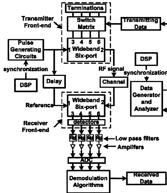
Fig. 2-1. Diagram of Multi(six)-port impulse-UWB platform.
