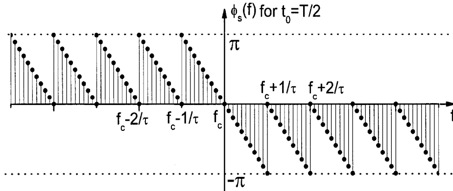
Fig. 5-2. Phase spectra of pulse signal s(t) .
