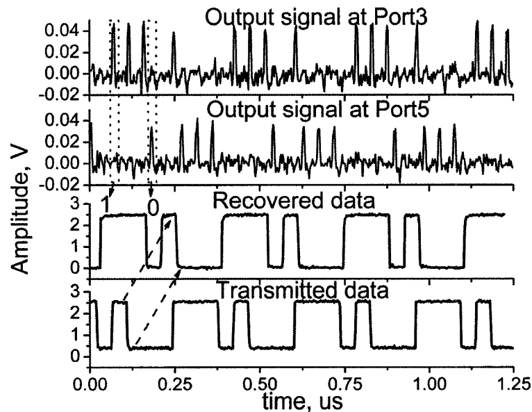
Fig. 4-22. Measured waveforms at ports 3 and 5 and comparison of recovered data with transmitted data.
