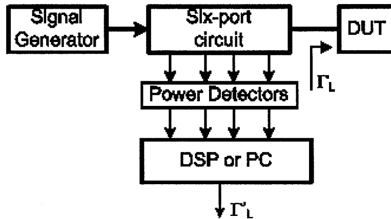
Fig. 1-4. Six-port reflectometer for microwave measurement.
