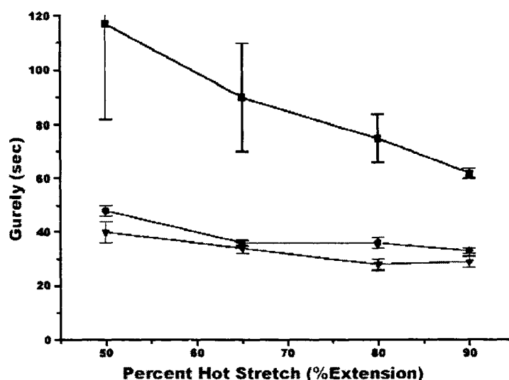
Figure 2.18 Effect of the hot stretching parameters ( T_{hs} and %HS) on the Gurley number for PMP Stretched films (■) T_{hs} = 120^{\circ}\text{C} , (●) T_{hs} = 160^{\circ}\text{C} and (▼) T_{ca} = 180^{\circ}\text{C} (Johnson et al. (2000)).
