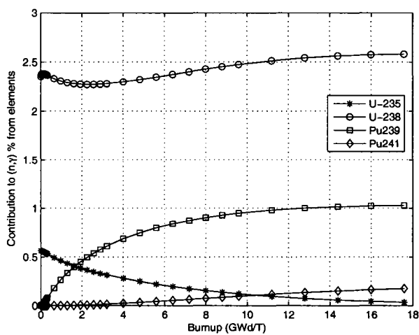
Figure 6.8 Contribution of (n, \gamma) to power normalization by selected actinides ('MODEL-1') as a function of burnup
