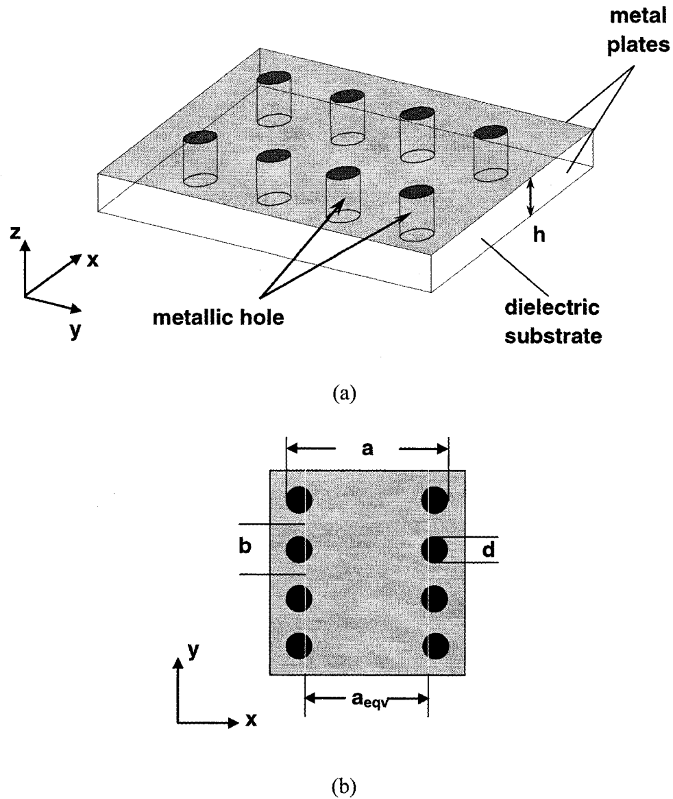
Figure 5.1 Topology of SIW structure (a) solid view; (b) top view
