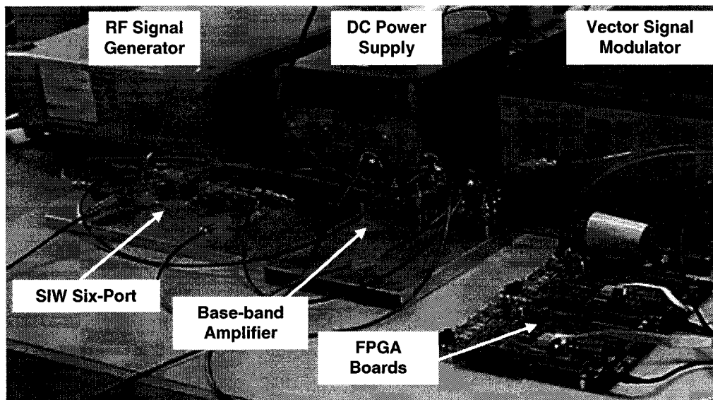
Figure 7.22 Test bed setup for receiver performance evaluation
