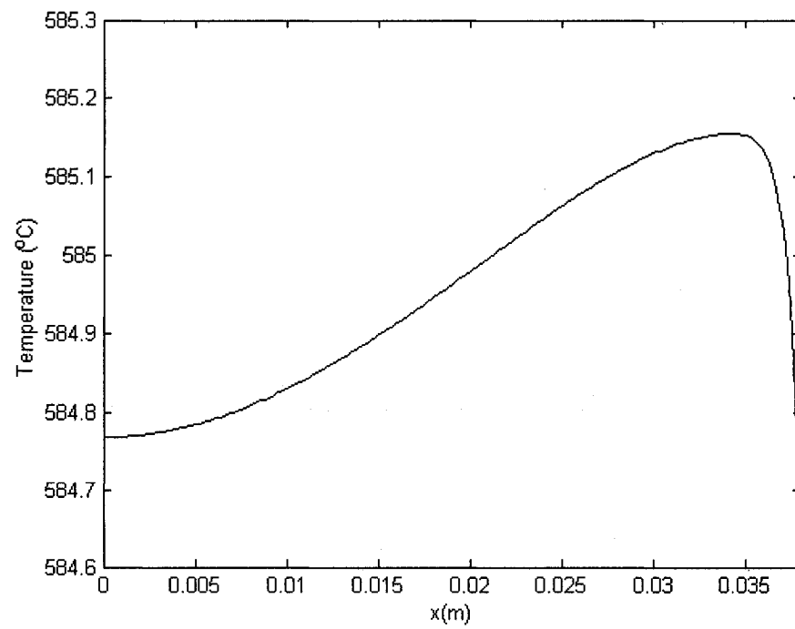
Figure 4.20b: Temperature distribution at the final time, t_f = 490\text{s} , P(t) = 50\%P_{\max}
