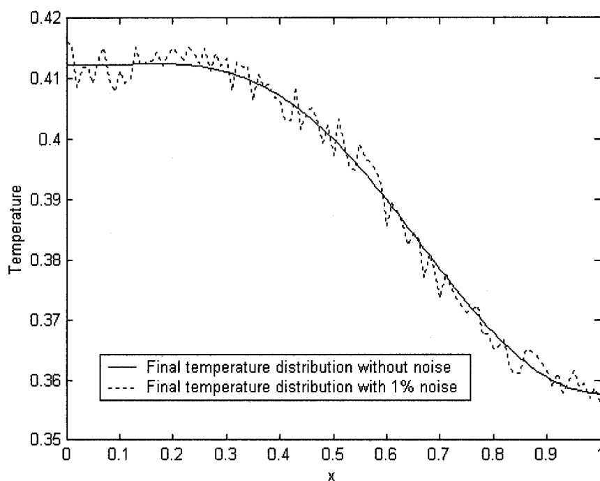
Figure 3.7b: Final temperature distribution, triangular profile
