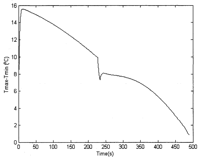
Figure 4.14c: Evolution temperature difference, t_f = 490\text{s} , initial guess G^0 = 65\%P_{\max} \sin(0.5\pi(t_f - t)/t_f)
